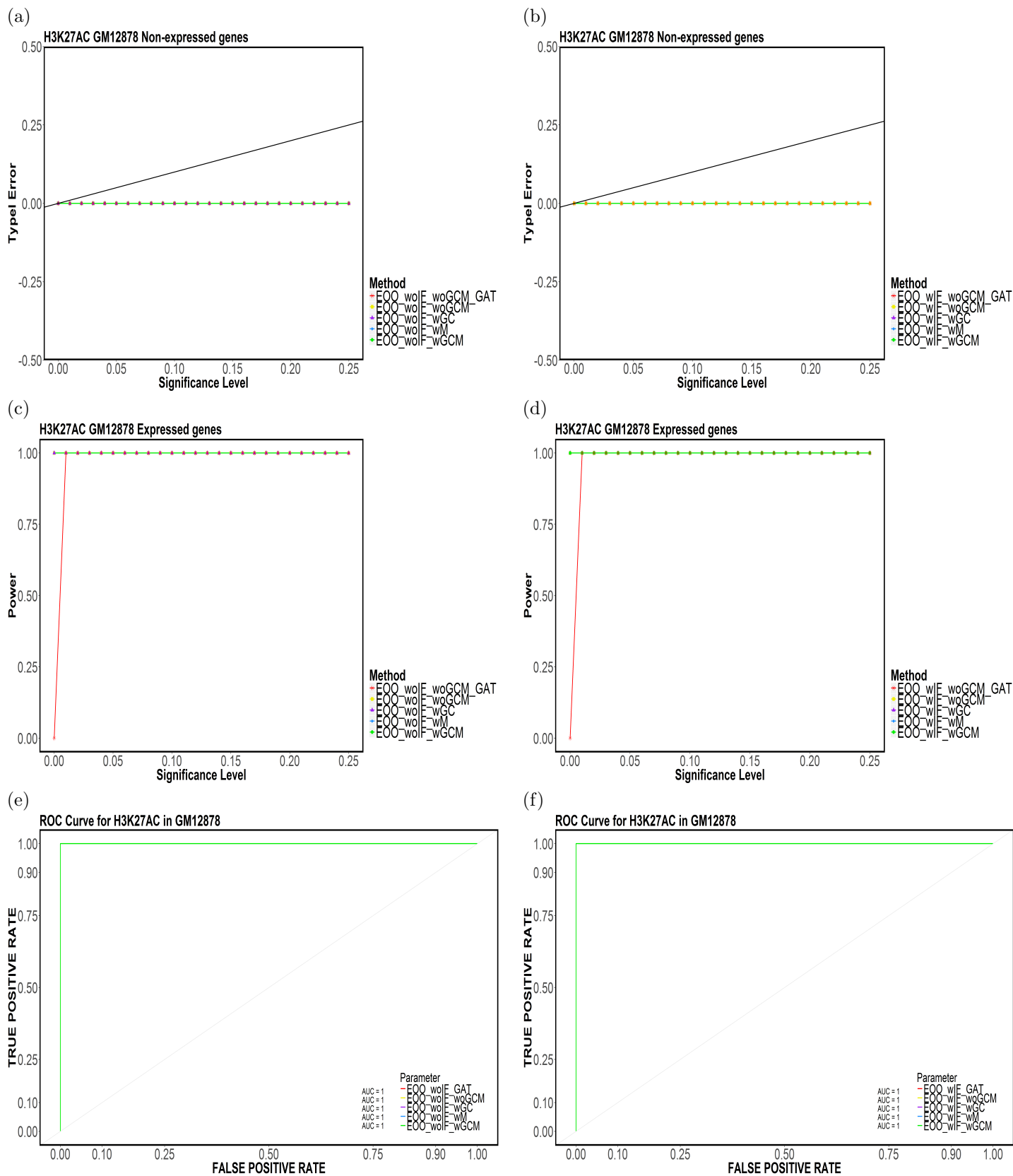
Figure 41: Element-based (a,b) Type-I Error, (c,d) Power and (e,f) ROC Curves for H3K27AC in GM12878 for (E00,CompletelyDiscard,Top5).
