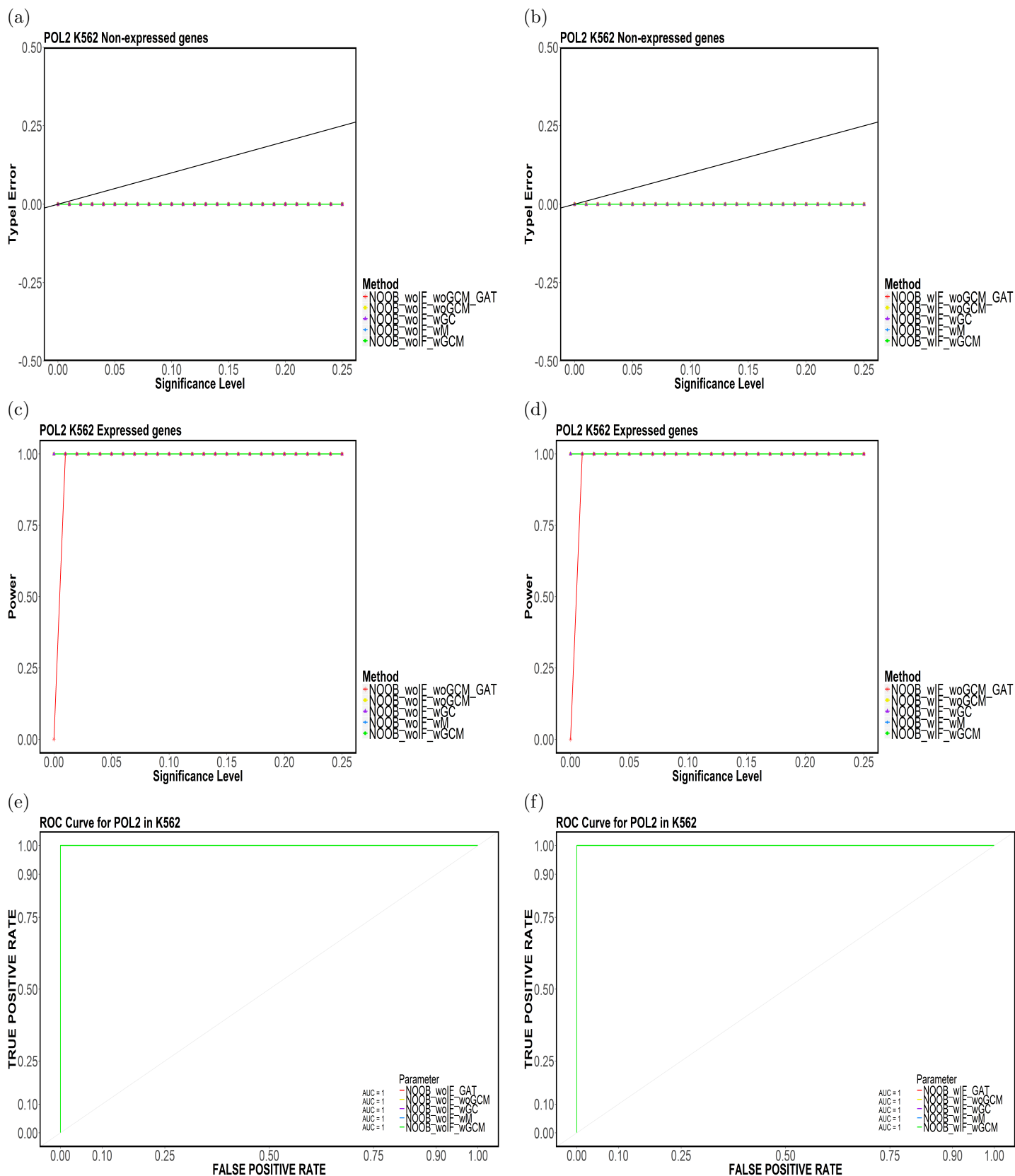
Figure 92: Element-based (a,b) Type-I Error, (c,d) Power and (e,f) ROC Curves for POL2 in K562 for (NOOB,TakeTheLongest,Top20).
