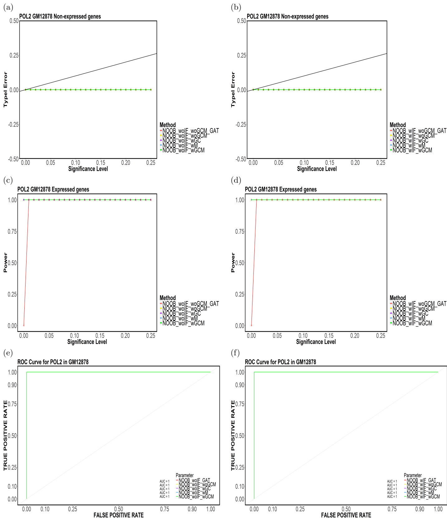
Figure 86: Element-based (a,b) Type-I Error, (c,d) Power and (e,f) ROC Curves for POL2 in GM12878 for (NOOB, CompletelyDiscard, Top5).
