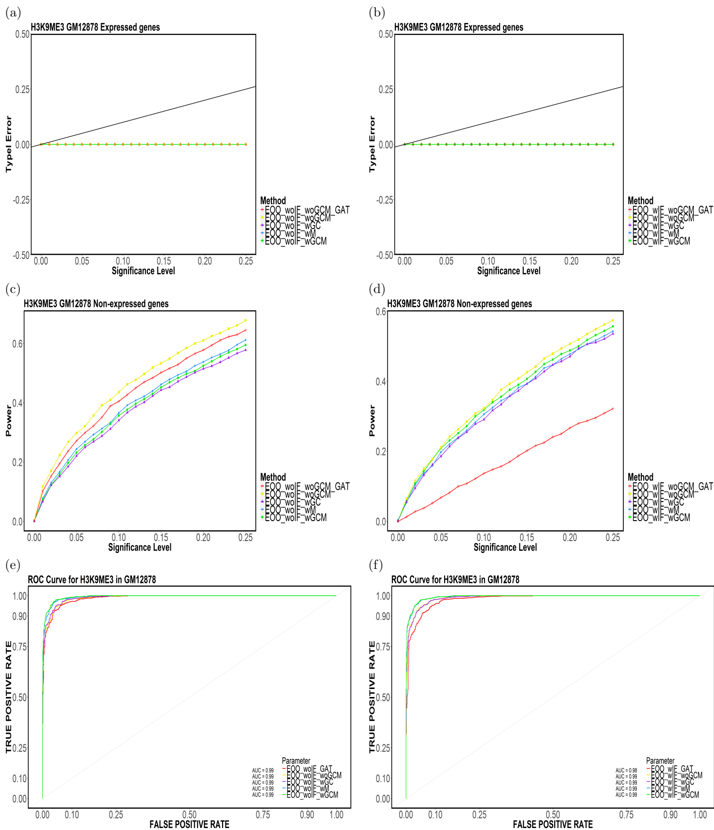
Figure 13: Element-based (a,b) Type-I Error, (c,d) Power and (e,f) ROC Curves for H3K9ME3 in GM12878 for (E00,TakeTheLongest,Top20).
