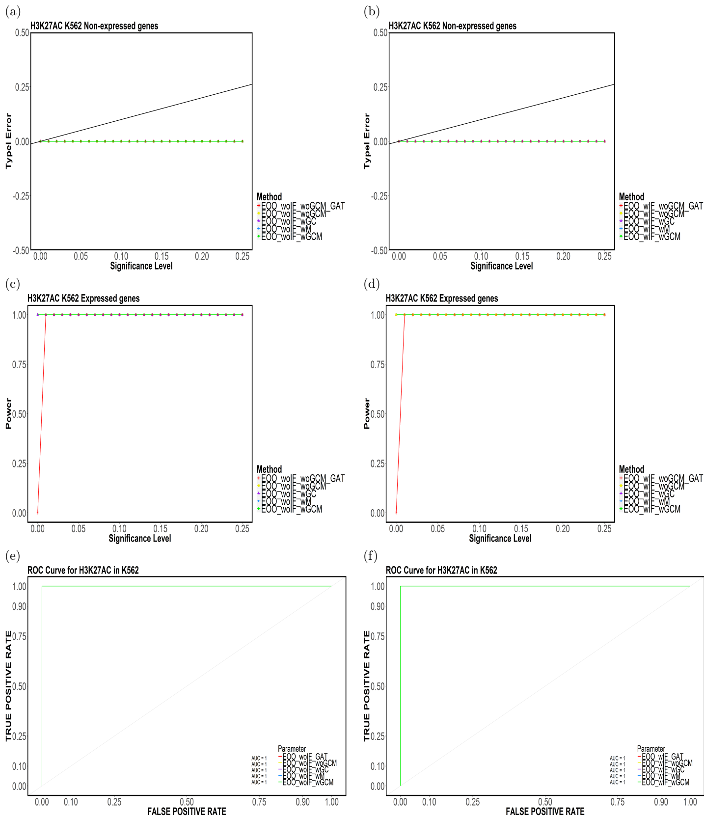
Figure 47: Element-based (a,b) Type-I Error, (c,d) Power and (e,f) ROC Curves for H3K27AC in K562 for (E00,TakeTheLongest,Top20).
