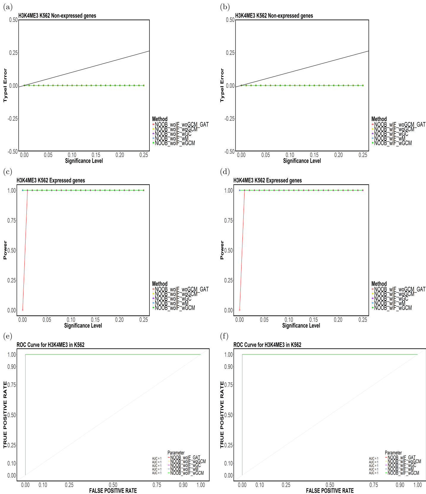
Figure 60: Element-based (a,b) Type-I Error, (c,d) Power and (e,f) ROC Curves for H3K4ME3 in K562 for (NOOB, CompletelyDiscard, Top5).
