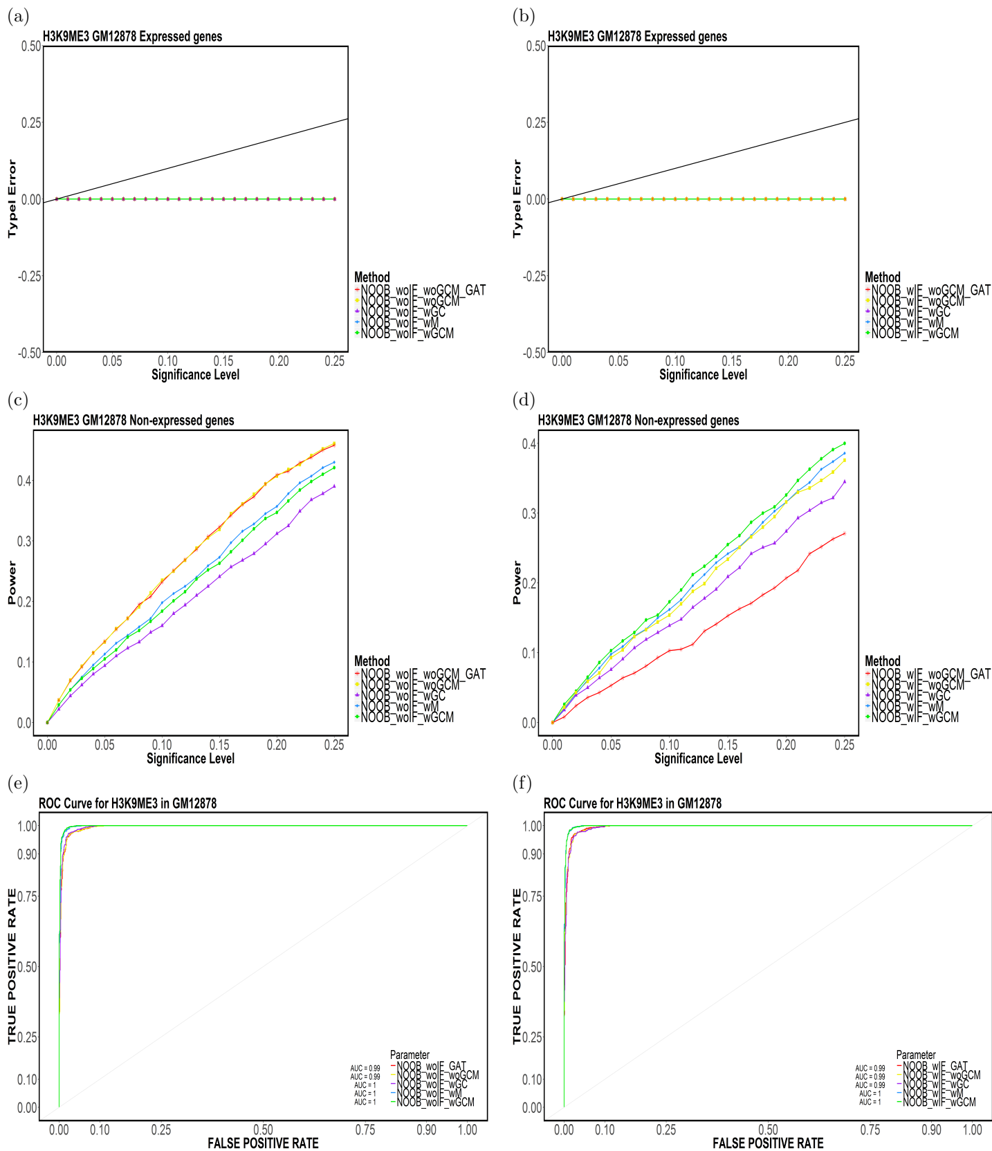
Figure 10: Element-based (a,b) Type-I Error, (c,d) Power and (e,f) ROC Curves for H3K9ME3 in GM12878 for (NOOB, CompletelyDiscard, Top5).
