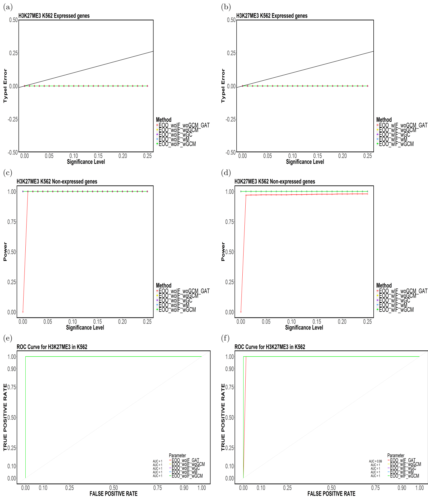
Figure 99: Element-based (a,b) Type-I Error, (c,d) Power and (e,f) ROC Curves for H3K27ME3 in K562 for (E00,TakeTheLongest,Top20).
