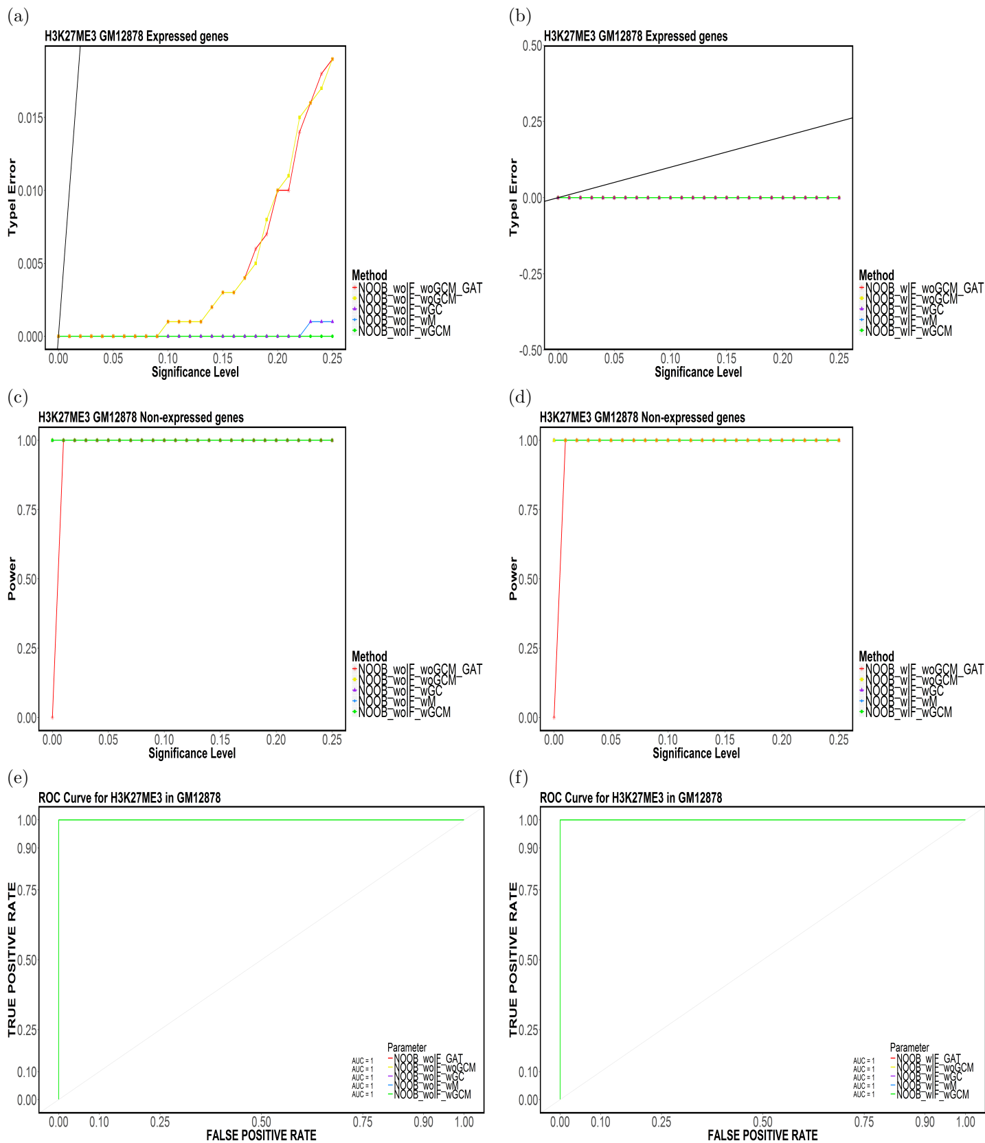
Figure 94: Element-based (a,b) Type-I Error, (c,d) Power and (e,f) ROC Curves for H3K27ME3 in GM12878 for (NOOB,CompletelyDiscard,Top5).
