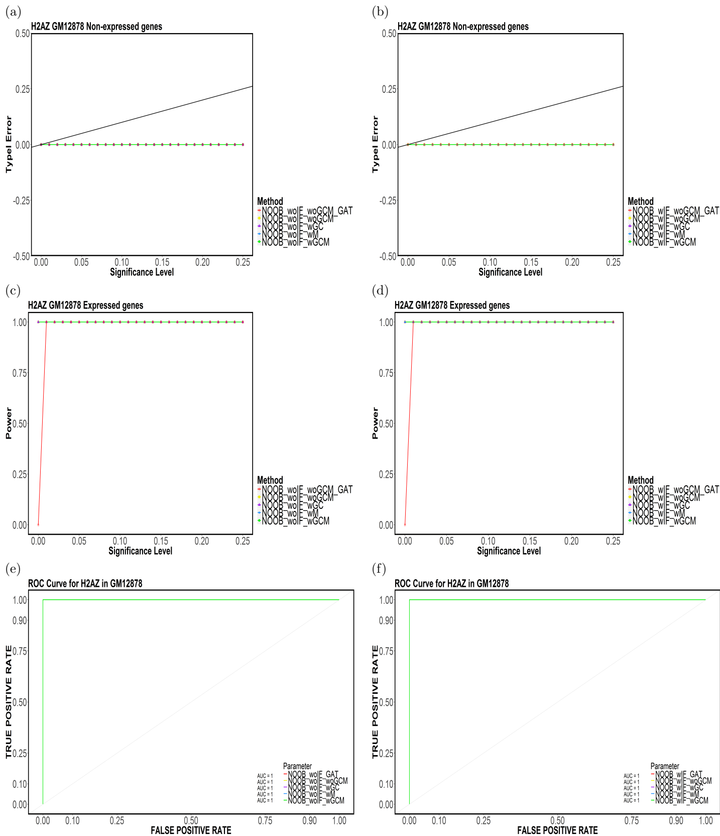
Figure 34: Element-based (a,b) Type-I Error, (c,d) Power and (e,f) ROC Curves for H2AZ in GM12878 for (NOOB, CompletelyDiscard, Top5).
