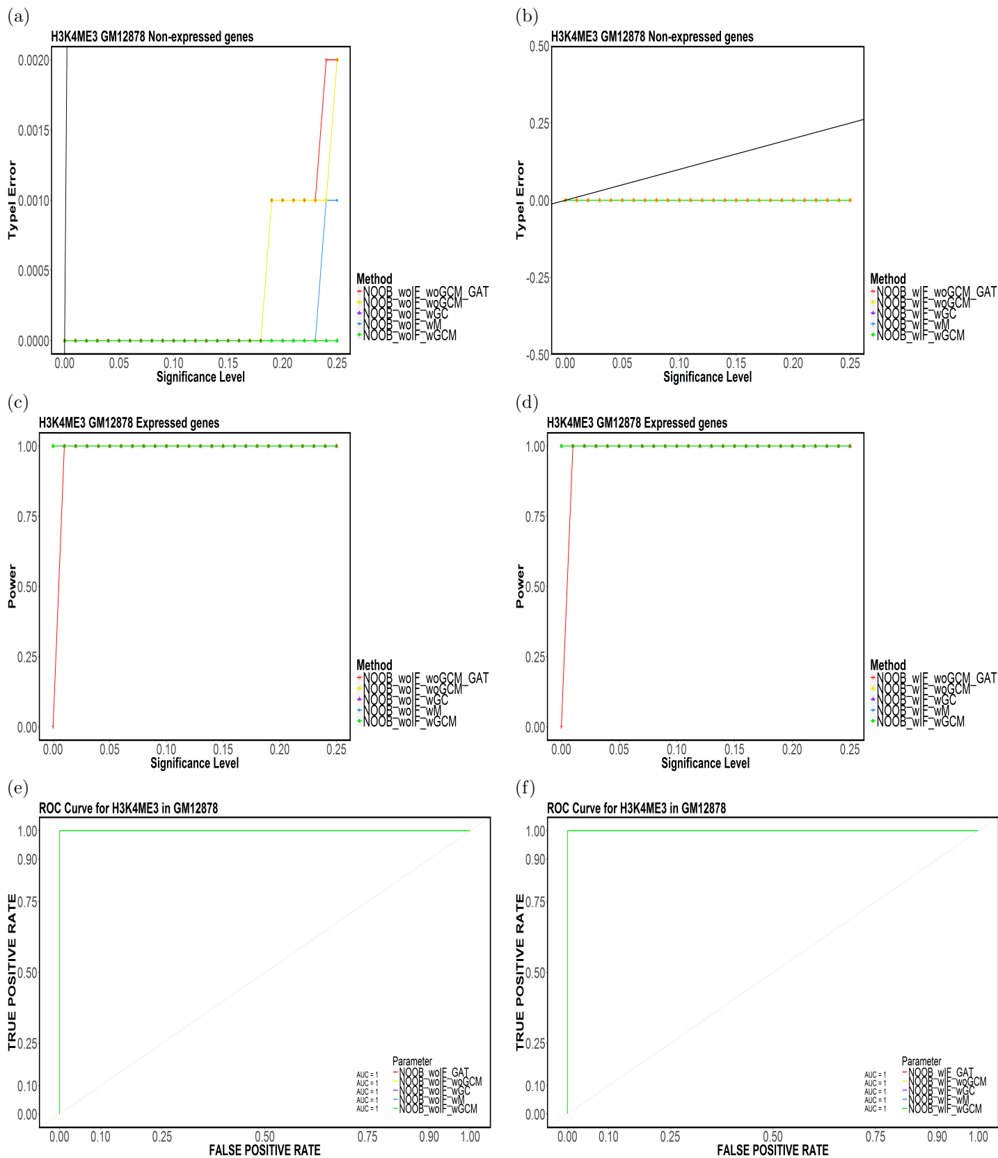
Figure 62: Element-based (a,b) Type-I Error, (c,d) Power and (e,f) ROC Curves for H3K4ME3 in GM12878 for (NOOB,TakeTheLongest,Top20).
