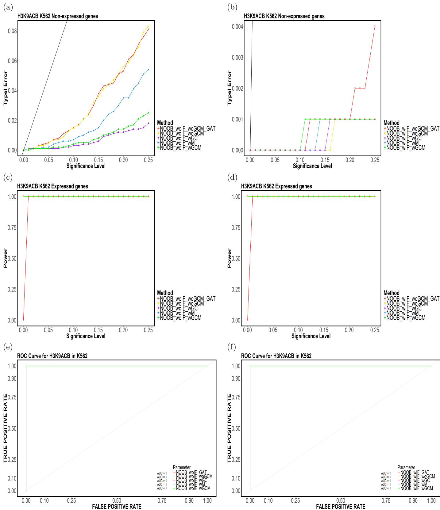
Figure 84: Element-based (a,b) Type-I Error, (c,d) Power and (e,f) ROC Curves for H3K9ACB in K562 for (NOOB,TakeTheLongest,Top20).
