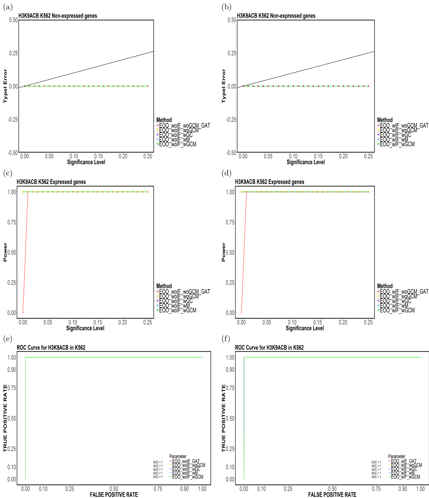
Figure 81: Element-based (a,b) Type-I Error, (c,d) Power and (e,f) ROC Curves for H3K9ACB in K562 for (E00,CompletelyDiscard,Top5).
