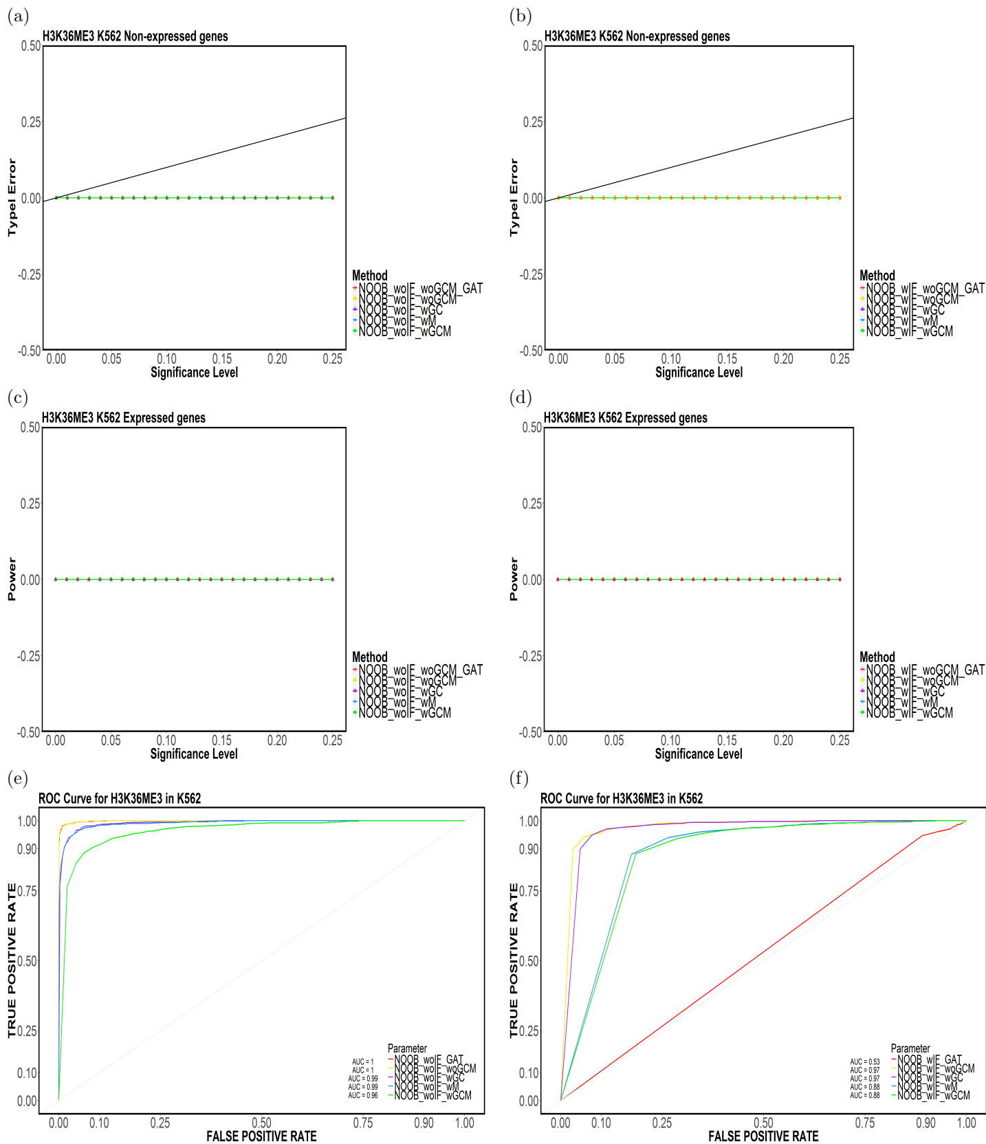
Figure 28: Element-based (a,b) Type-I Error, (c,d) Power and (e,f) ROC Curves for H3K36ME3 in K562 for (NOOB, CompletelyDiscard, Top5).
