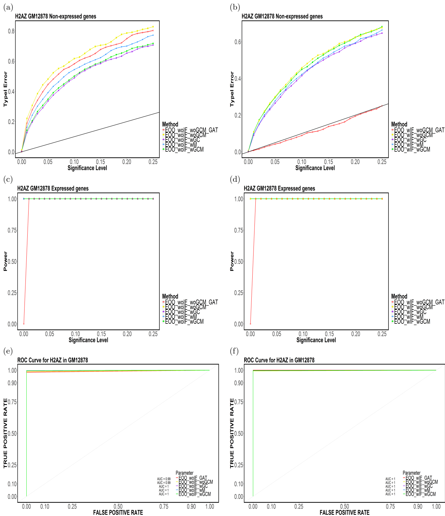
Figure 37: Element-based (a,b) Type-I Error, (c,d) Power and (e,f) ROC Curves for H2AZ in GM12878 for (E00,TakeTheLongest,Top20).
