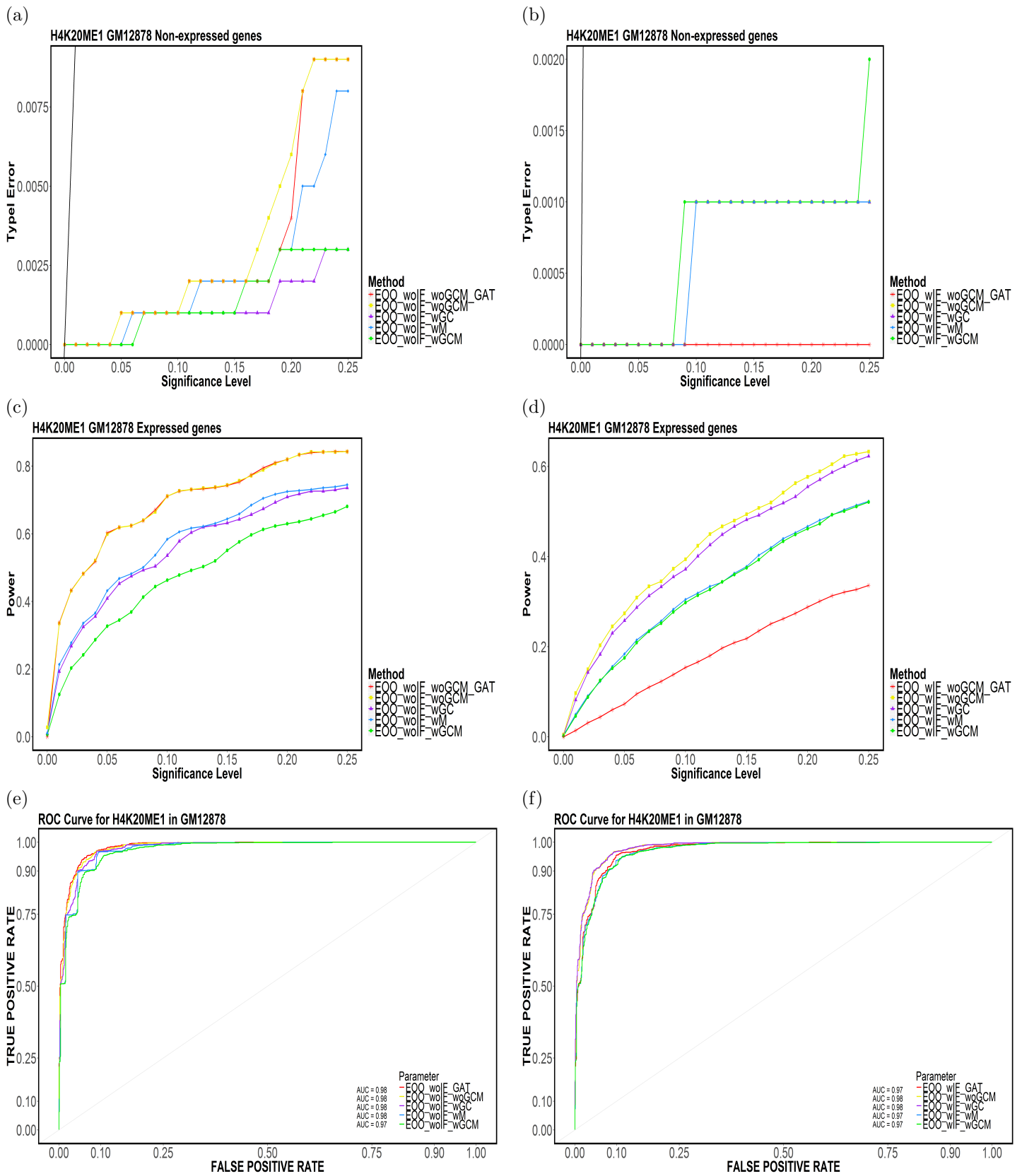
Figure 5: Element-based (a,b) Type-I Error, (c,d) Power and (e,f) ROC Curves for H4K20ME1 in GM12878 for (E00,TakeTheLongest,Top20).
