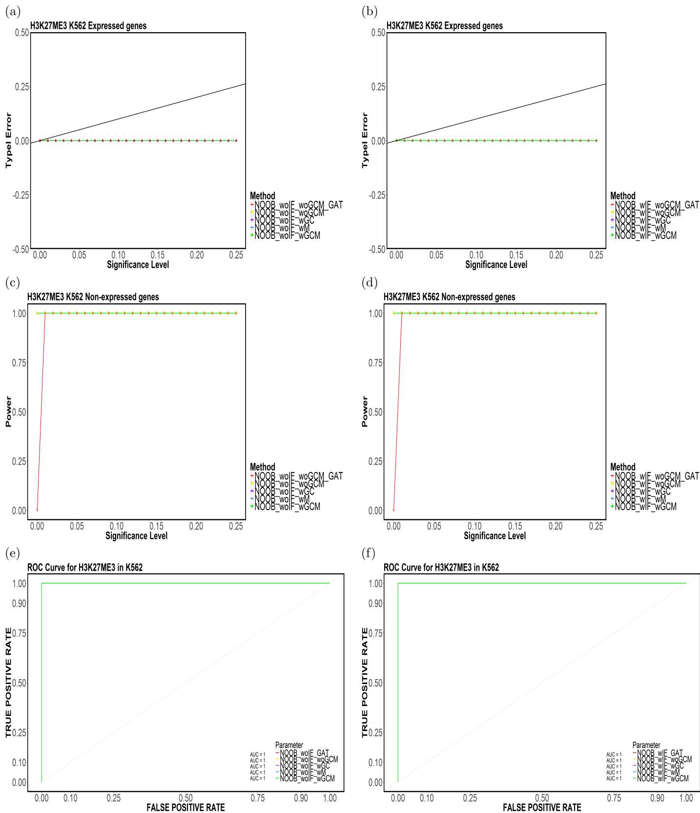
Figure 96: Element-based (a,b) Type-I Error, (c,d) Power and (e,f) ROC Curves for H3K27ME3 in K562 for (NOOB, CompletelyDiscard, Top5).
