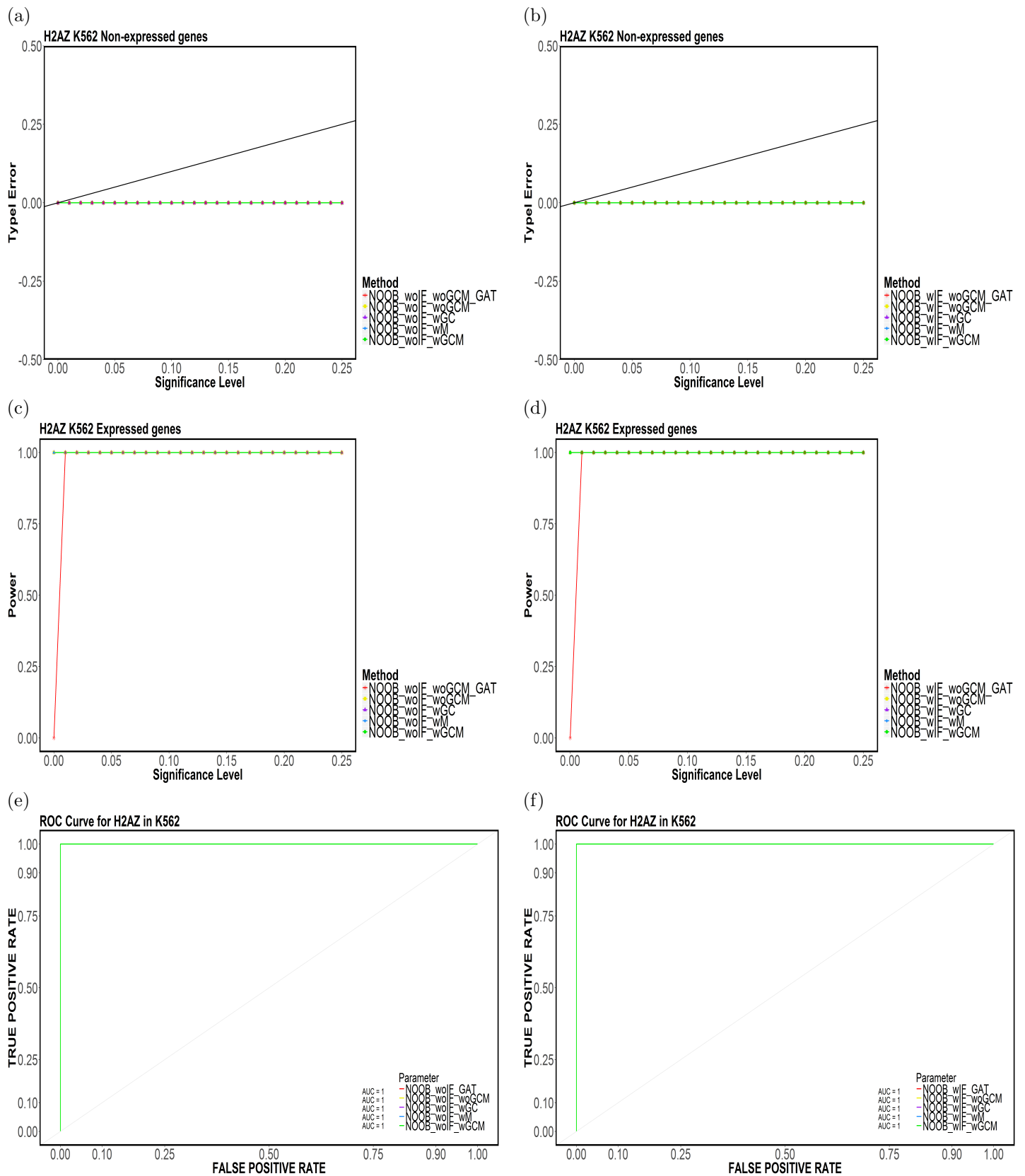
Figure 36: Element-based (a,b) Type-I Error, (c,d) Power and (e,f) ROC Curves for H2AZ in K562 for (NOOB,CompletelyDiscard,Top5).
