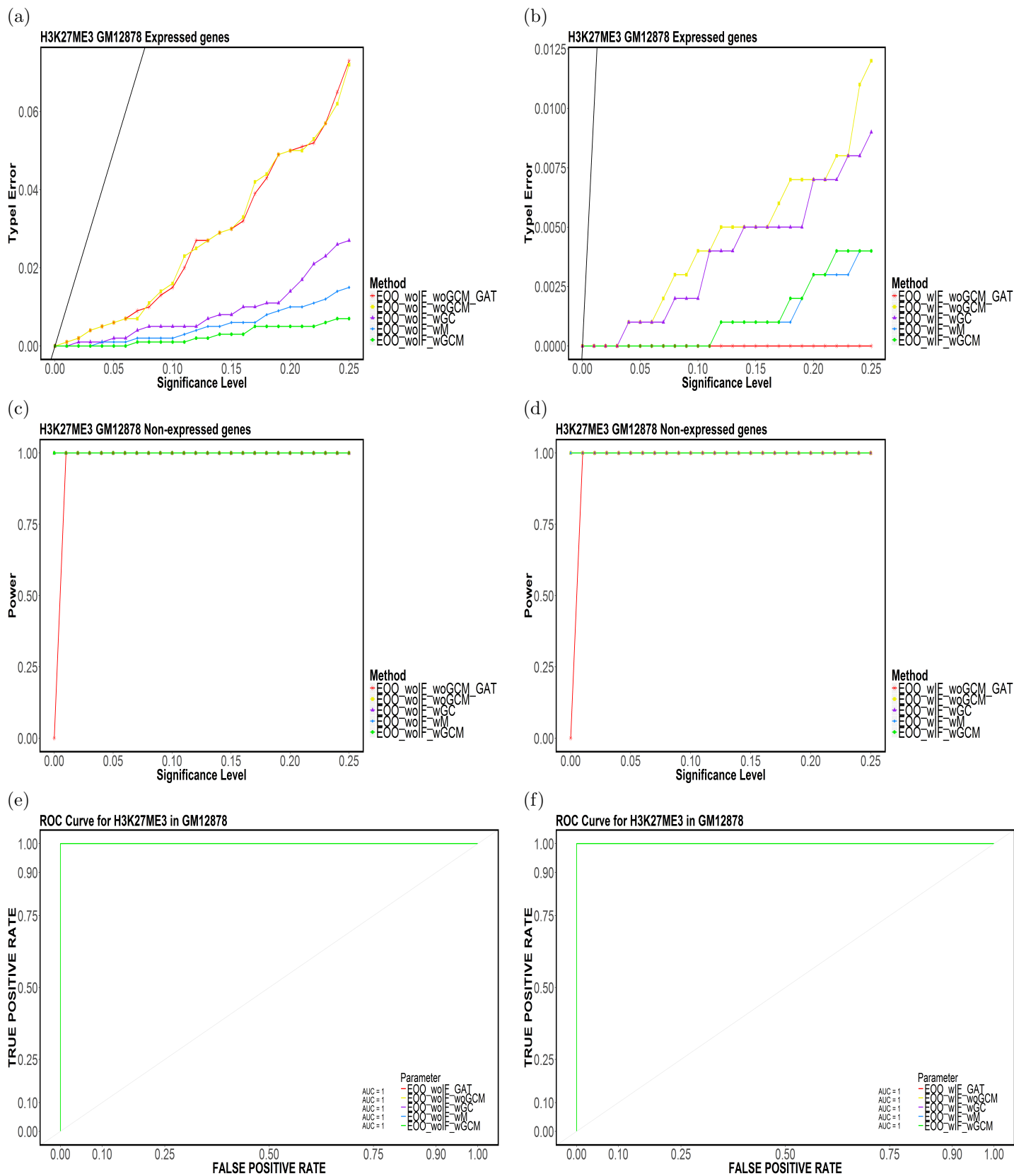
Figure 97: Element-based (a,b) Type-I Error, (c,d) Power and (e,f) ROC Curves for H3K27ME3 in GM12878 for (E00,TakeTheLongest,Top20).
