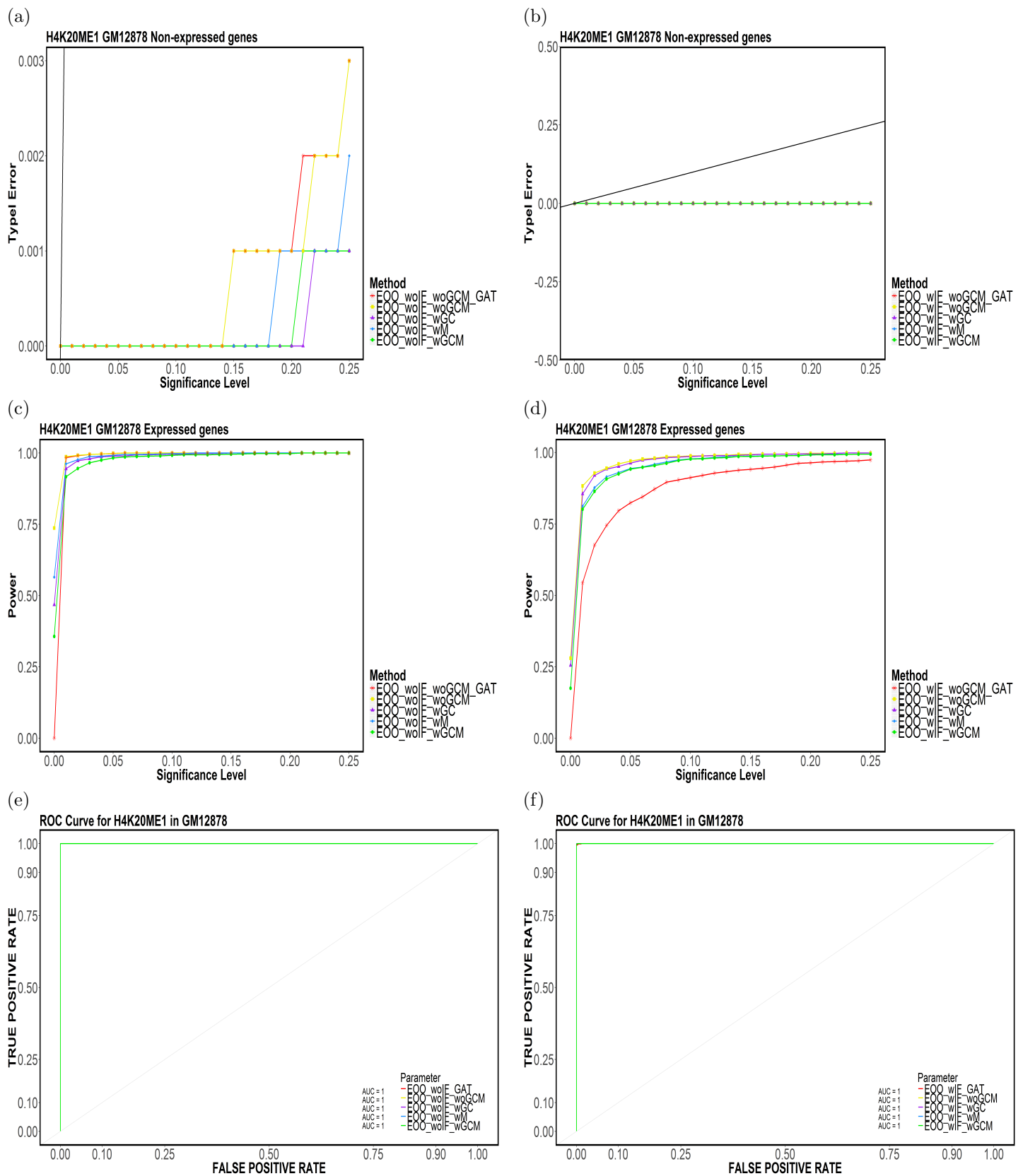
Figure 1: Element-based (a,b) Type-I Error, (c,d) Power and (e,f) ROC Curves for H4K20ME1 in GM12878 for (E00,CompletelyDiscard,Top5).
