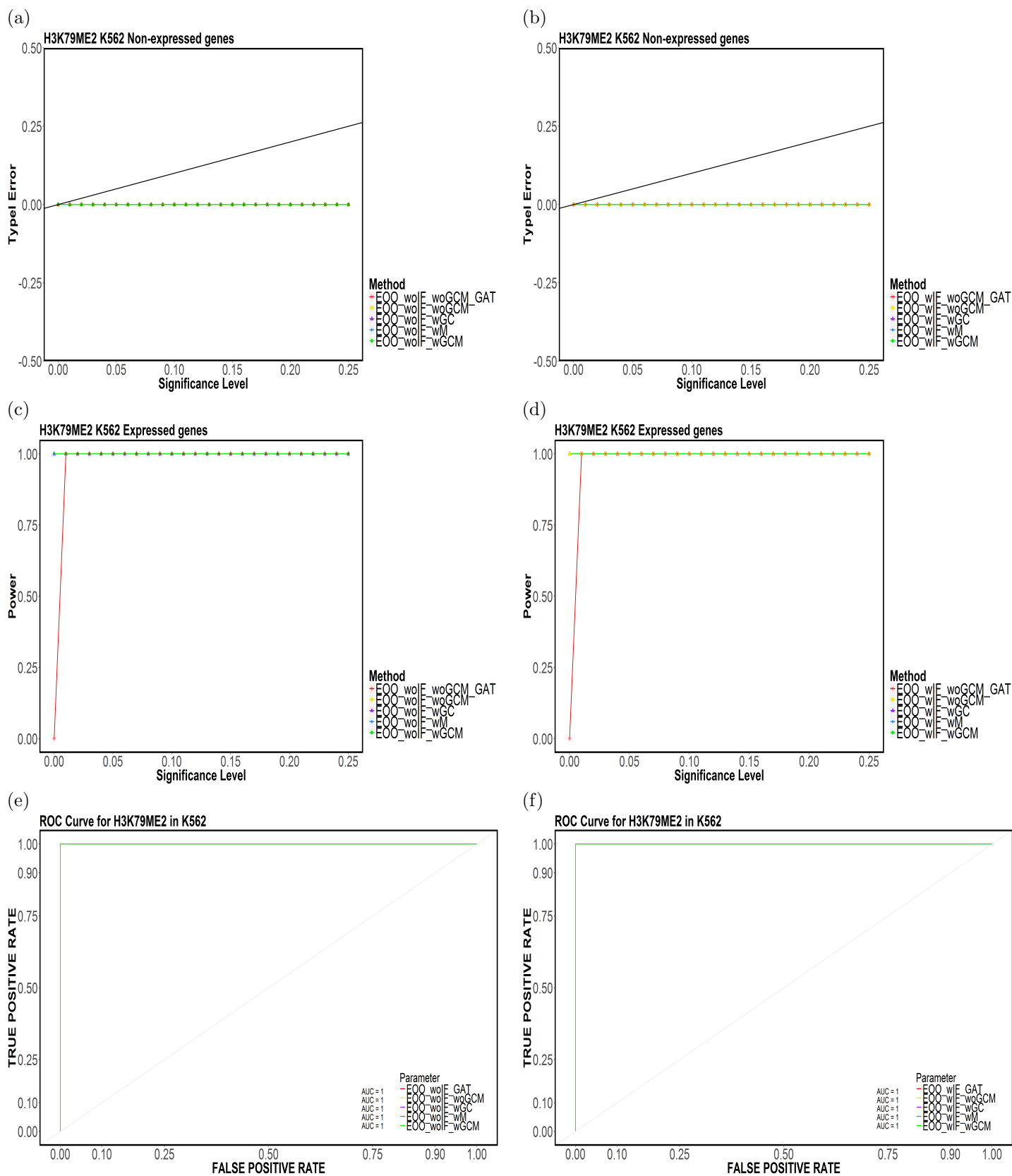
Figure 71: Element-based (a,b) Type-I Error, (c,d) Power and (e,f) ROC Curves for H3K79ME2 in K562 for (E00,TakeTheLongest,Top20).
