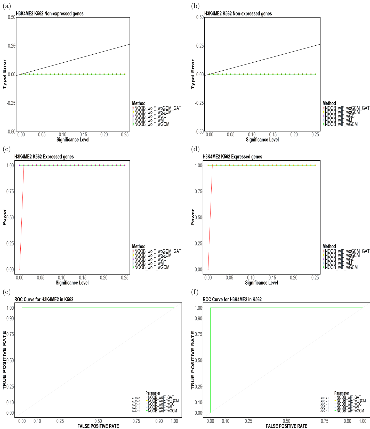
Figure 52: Element-based (a,b) Type-I Error, (c,d) Power and (e,f) ROC Curves for H3K4ME2 in K562 for (NOOB, CompletelyDiscard, Top5).
