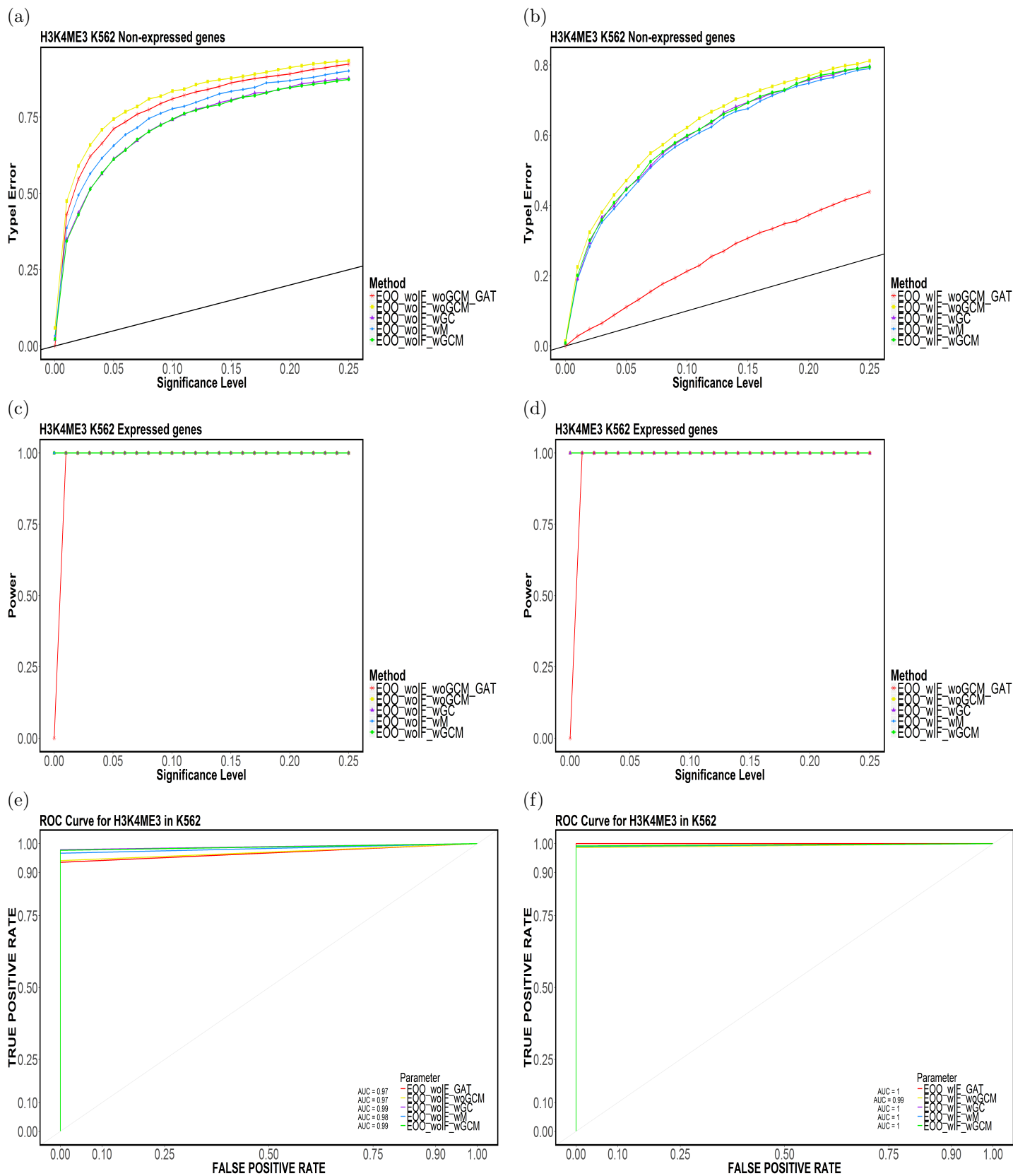
Figure 63: Element-based (a,b) Type-I Error, (c,d) Power and (e,f) ROC Curves for H3K4ME3 in K562 for (E00,TakeTheLongest,Top20).
