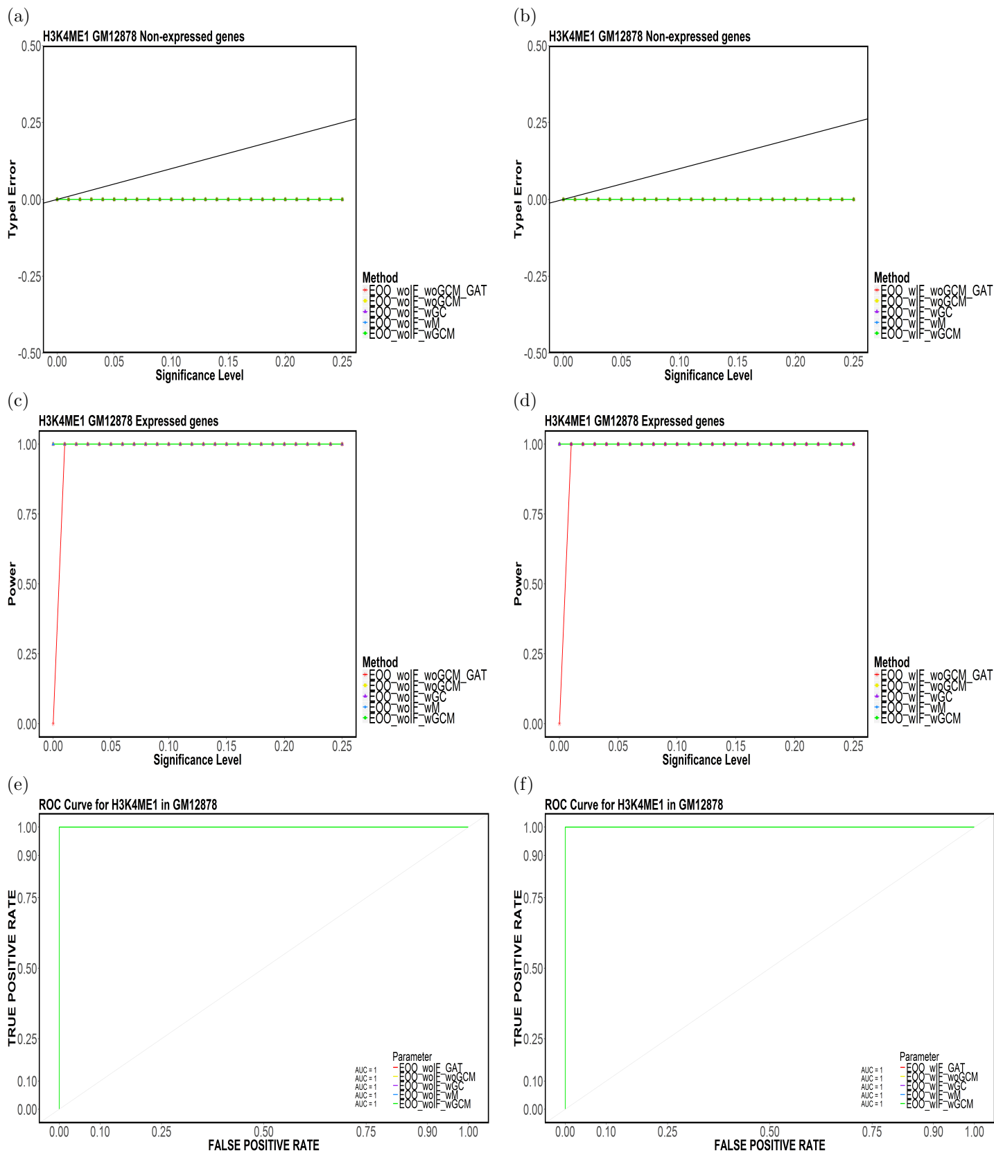
Figure 21: Element-based (a,b) Type-I Error, (c,d) Power and (e,f) ROC Curves for H3K4ME1 in GM12878 for (E00,TakeTheLongest,Top20).
