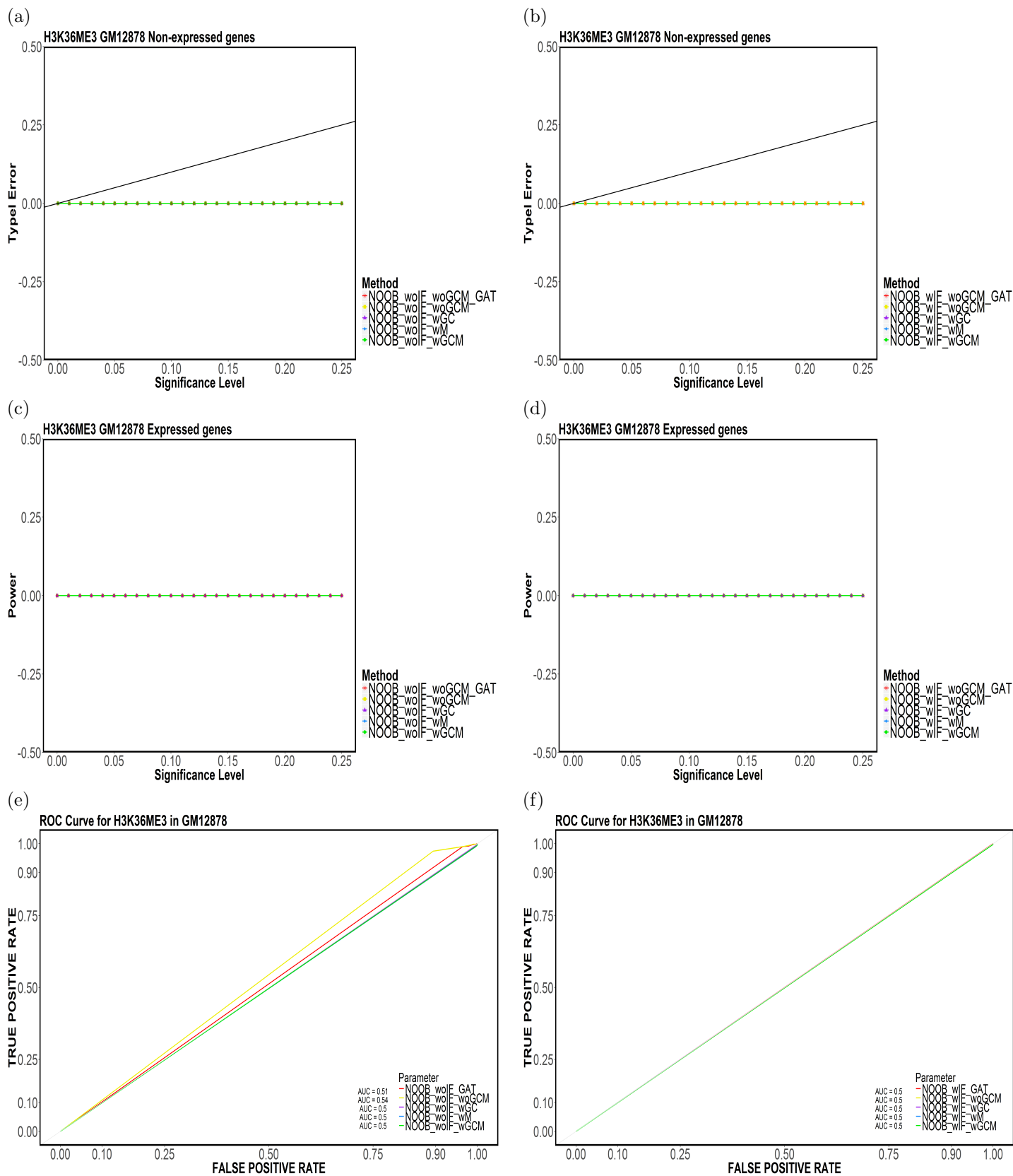
Figure 26: Element-based (a,b) Type-I Error, (c,d) Power and (e,f) ROC Curves for H3K36ME3 in GM12878 for (NOOB,CompletelyDiscard,Top5).
