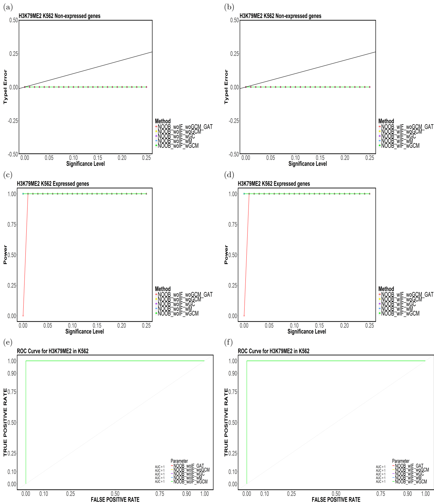
Figure 72: Element-based (a,b) Type-I Error, (c,d) Power and (e,f) ROC Curves for H3K79ME2 in K562 for (NOOB,TakeTheLongest,Top20).
