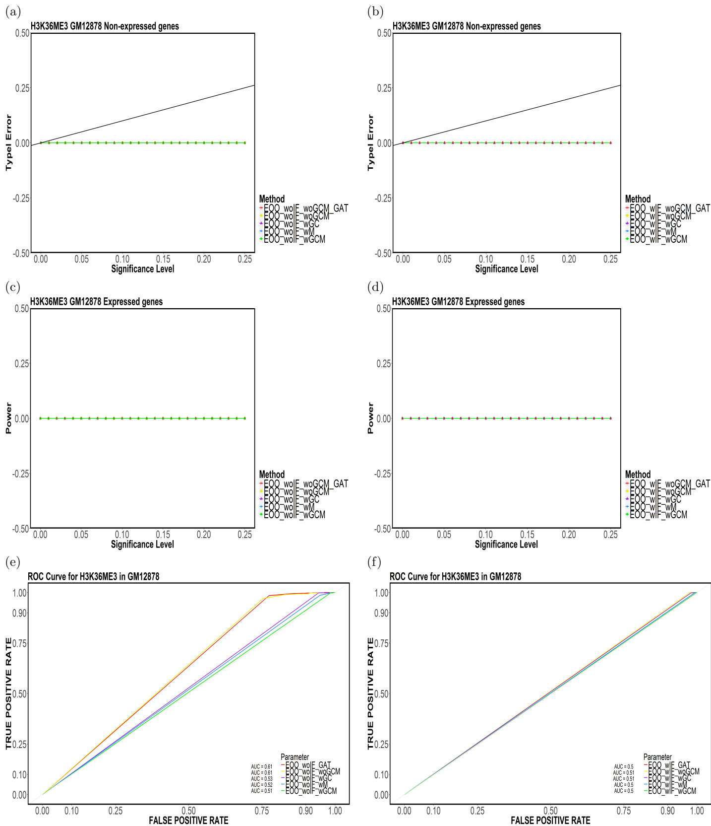
Figure 29: Element-based (a,b) Type-I Error, (c,d) Power and (e,f) ROC Curves for H3K36ME3 in GM12878 for (E00,TakeTheLongest,Top20).
