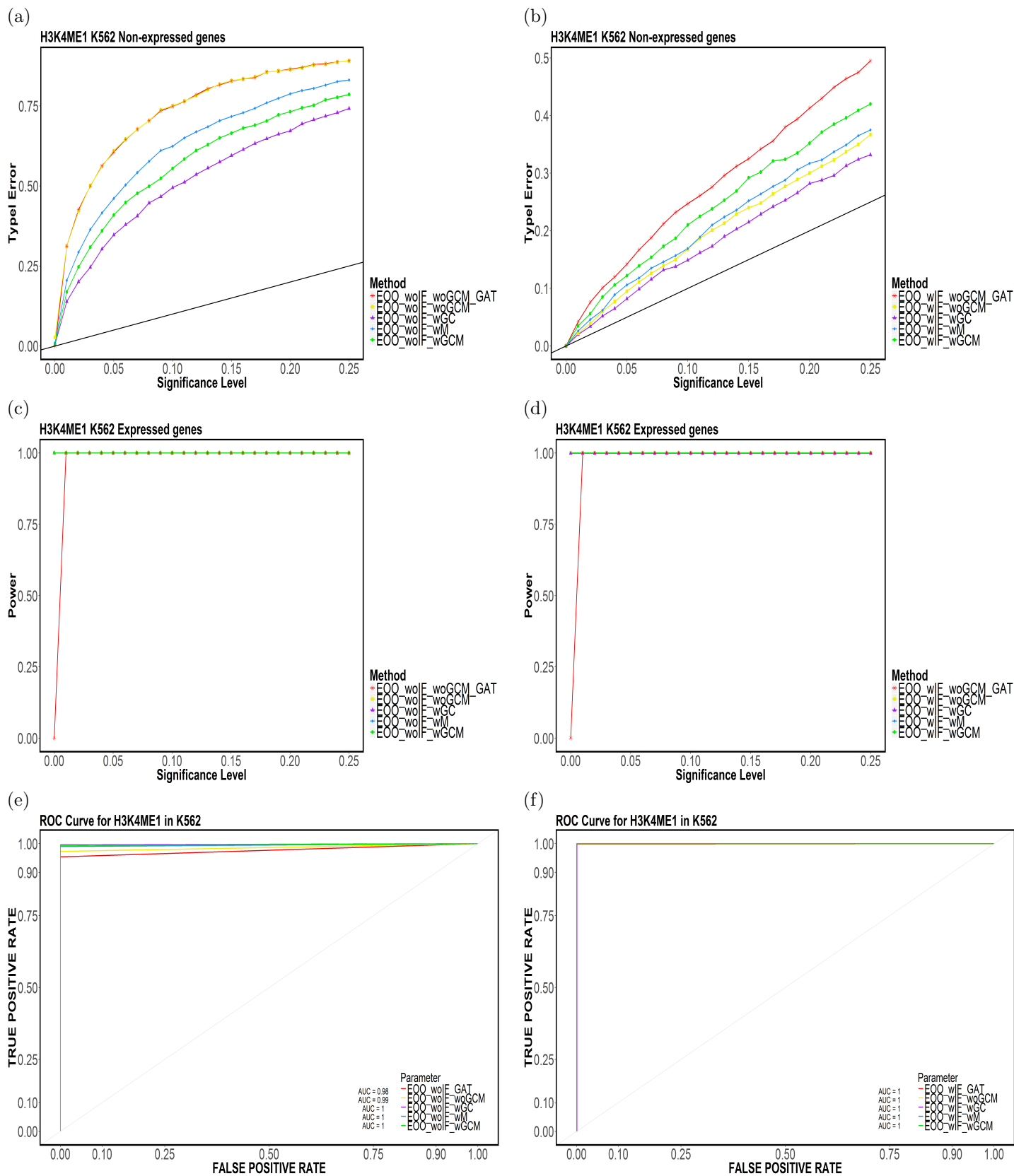
Figure 19: Element-based (a,b) Type-I Error, (c,d) Power and (e,f) ROC Curves for H3K4ME1 in K562 for (E00,CompletelyDiscard,Top5).
