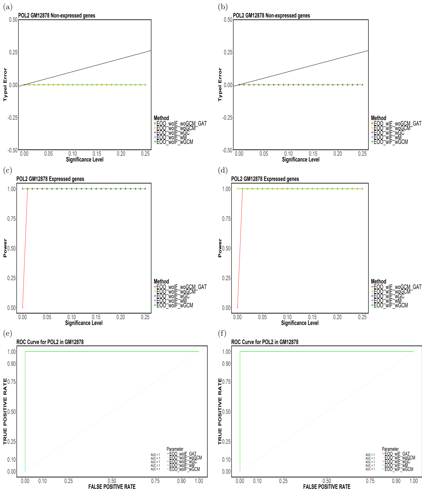
Figure 89: Element-based (a,b) Type-I Error, (c,d) Power and (e,f) ROC Curves for POL2 in GM12878 for (E00,TakeTheLongest,Top20).
