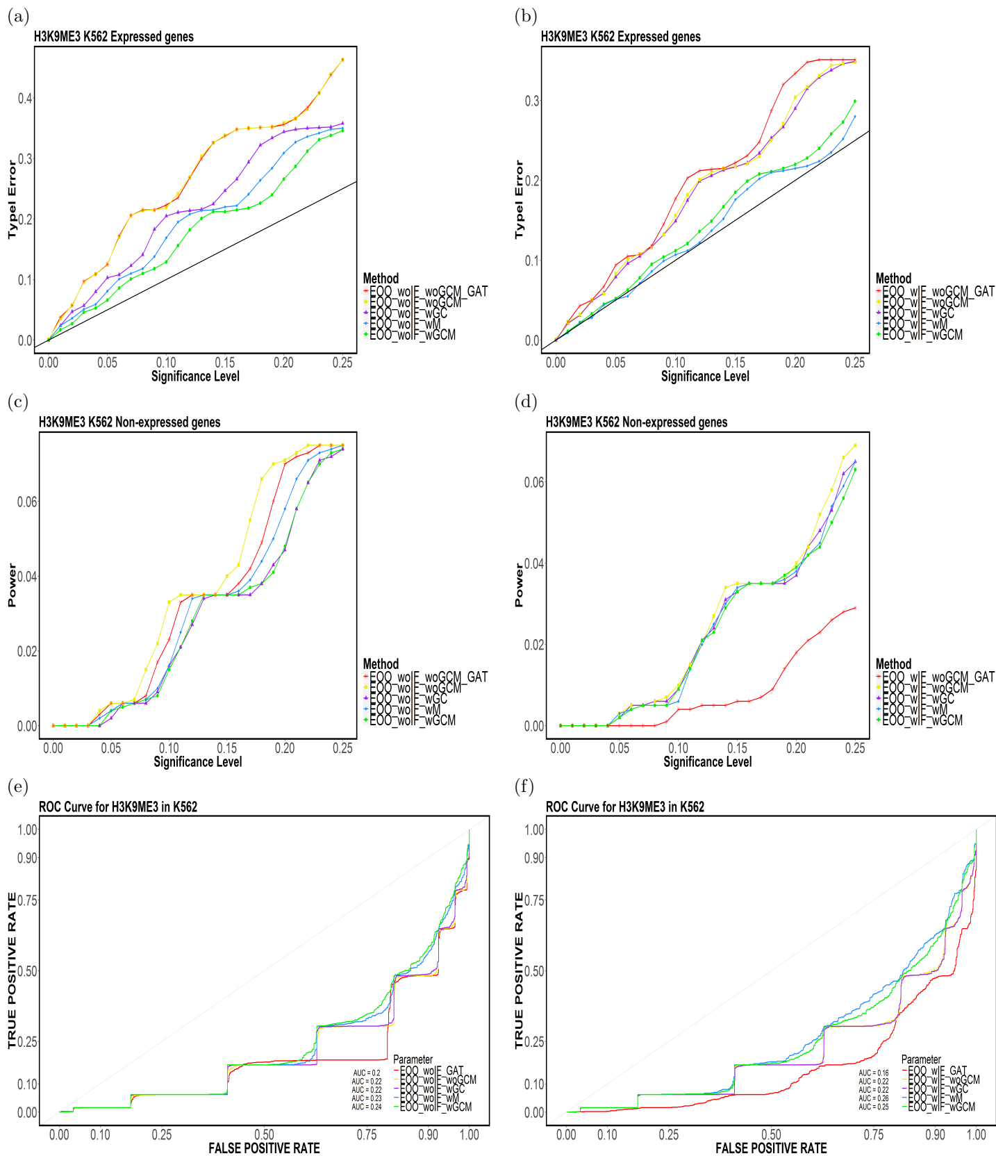
Figure 15: Element-based (a,b) Type-I Error, (c,d) Power and (e,f) ROC Curves for H3K9ME3 in K562 for (E00,TakeTheLongest,Top20).
