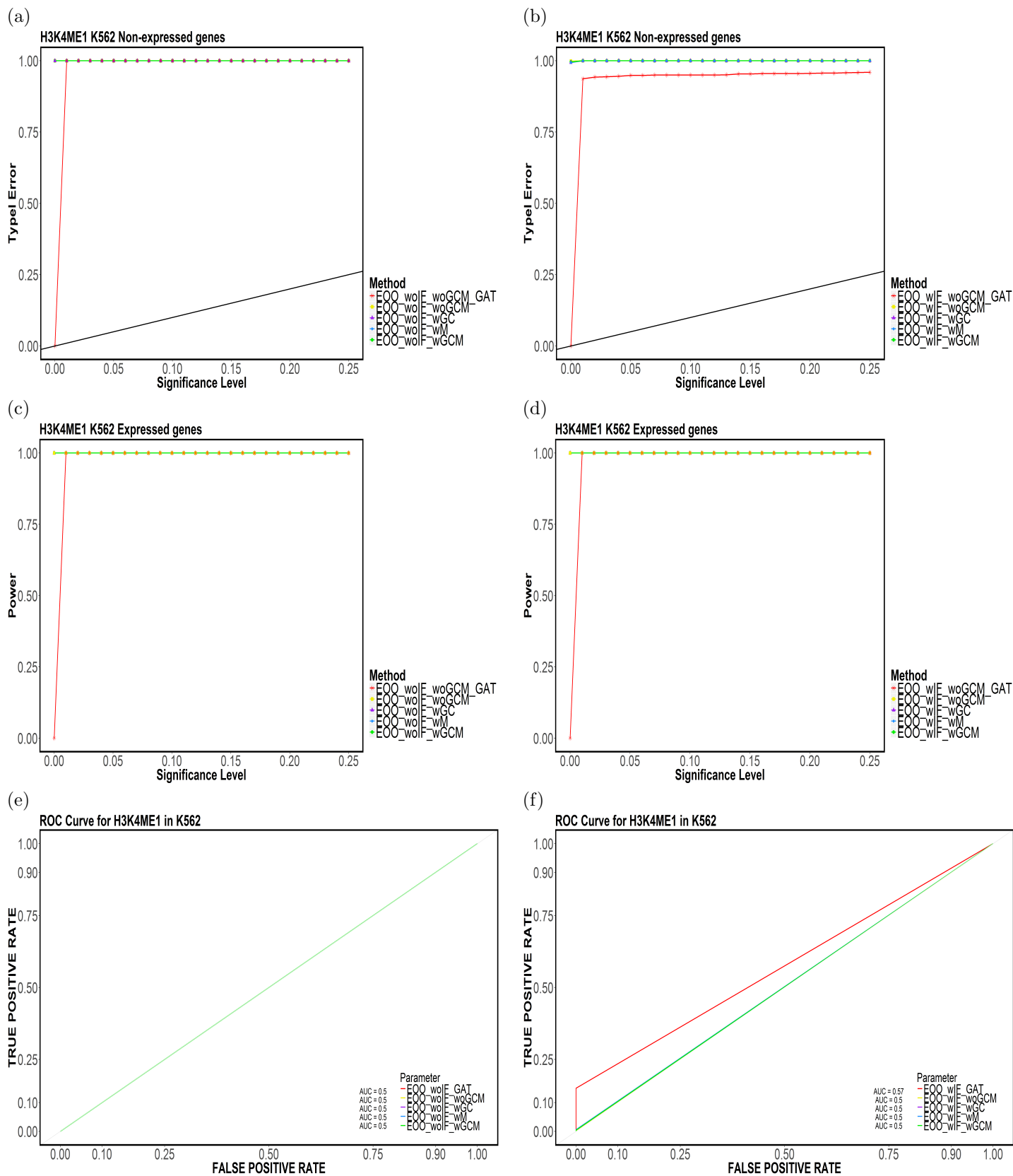
Figure 23: Element-based (a,b) Type-I Error, (c,d) Power and (e,f) ROC Curves for H3K4ME1 in K562 for (E00,TakeTheLongest,Top20).
