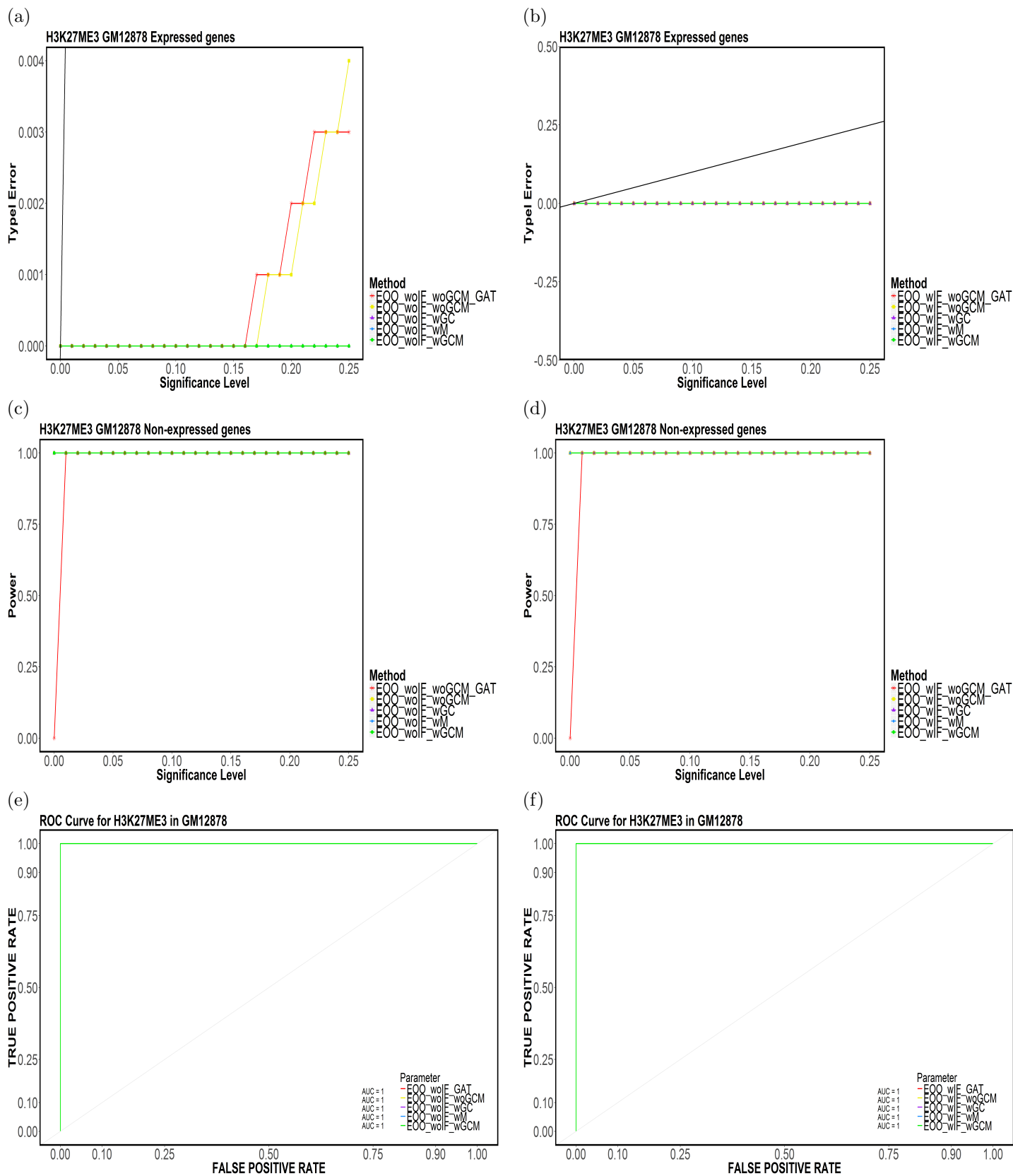
Figure 93: Element-based (a,b) Type-I Error, (c,d) Power and (e,f) ROC Curves for H3K27ME3 in GM12878 for (E00,CompletelyDiscard,Top5).
