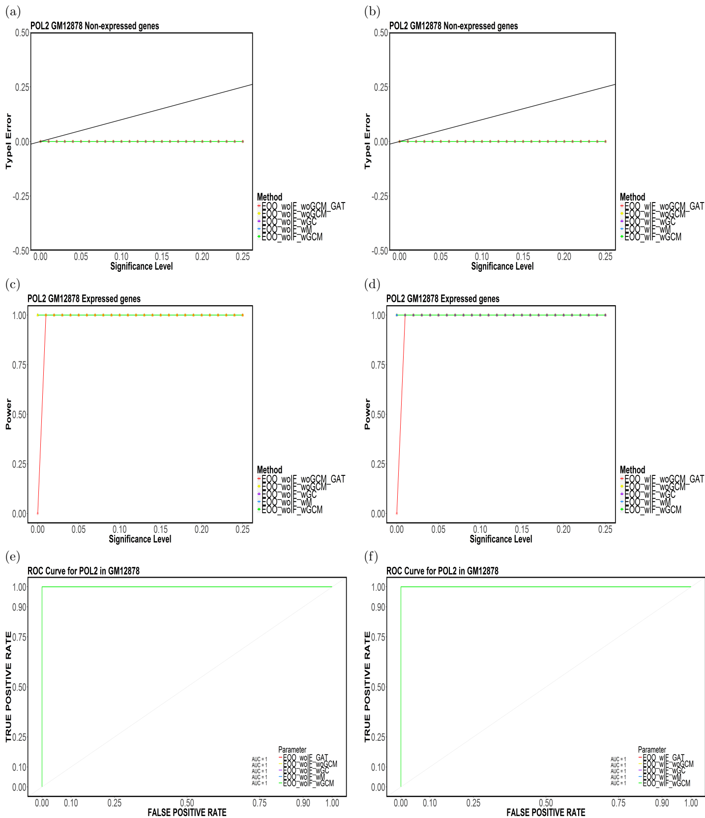
Figure 85: Element-based (a,b) Type-I Error, (c,d) Power and (e,f) ROC Curves for POL2 in GM12878 for (E00,CompletelyDiscard,Top5).
