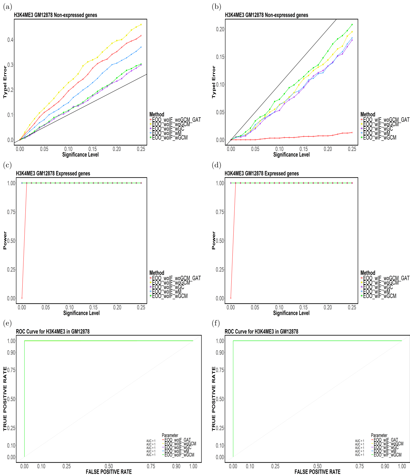
Figure 61: Element-based (a,b) Type-I Error, (c,d) Power and (e,f) ROC Curves for H3K4ME3 in GM12878 for (E00,TakeTheLongest,Top20).
