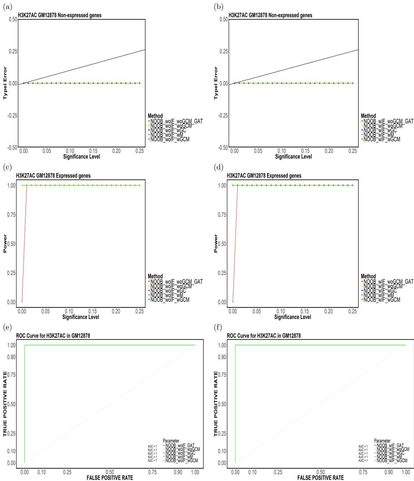
Figure 46: Element-based (a,b) Type-I Error, (c,d) Power and (e,f) ROC Curves for H3K27AC in GM12878 for (NOOB,TakeTheLongest,Top20).
