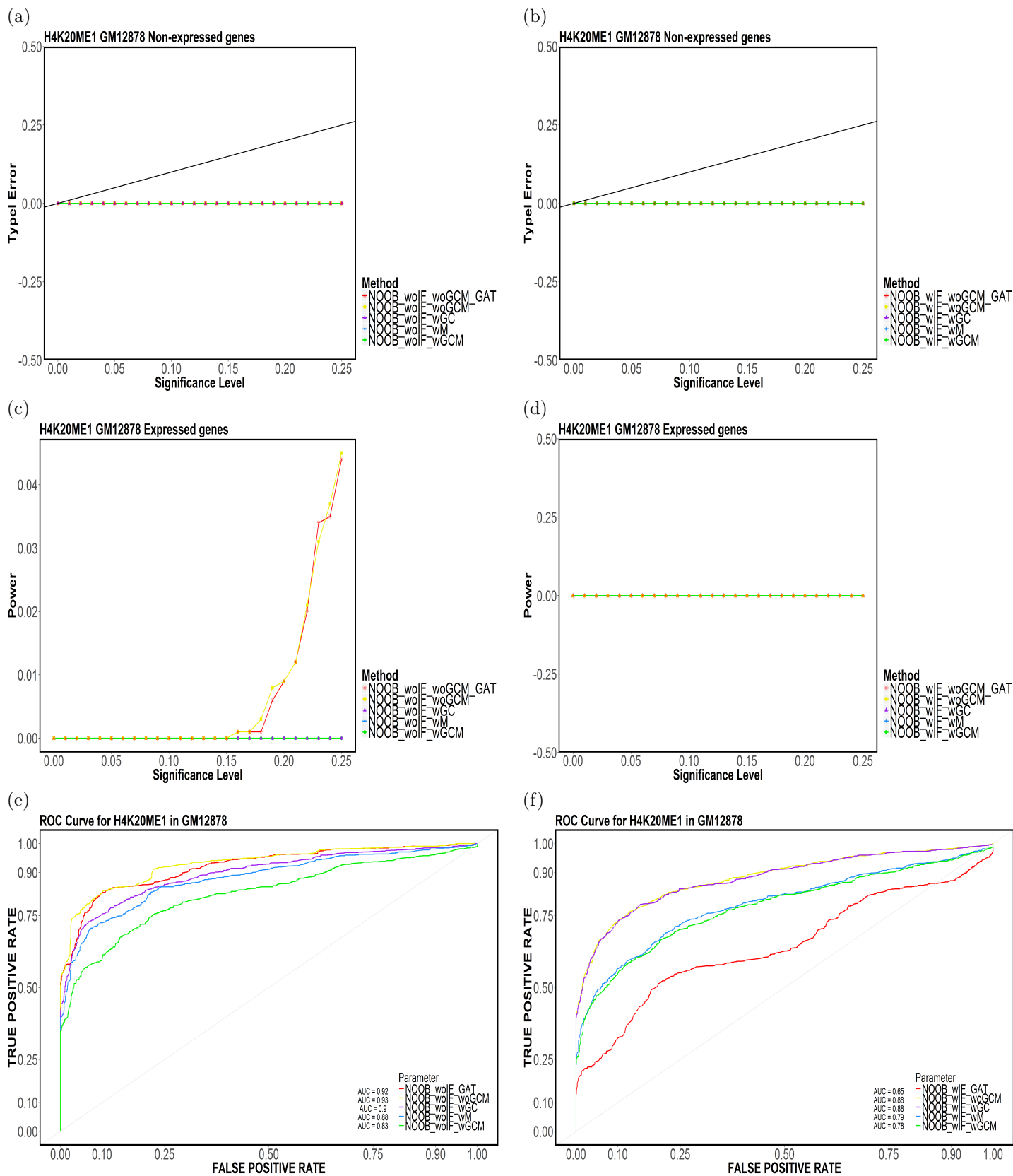
Figure 2: Element-based (a,b) Type-I Error, (c,d) Power and (e,f) ROC Curves for H4K20ME1 in GM12878 for (NOOB,CompletelyDiscard,Top5).
