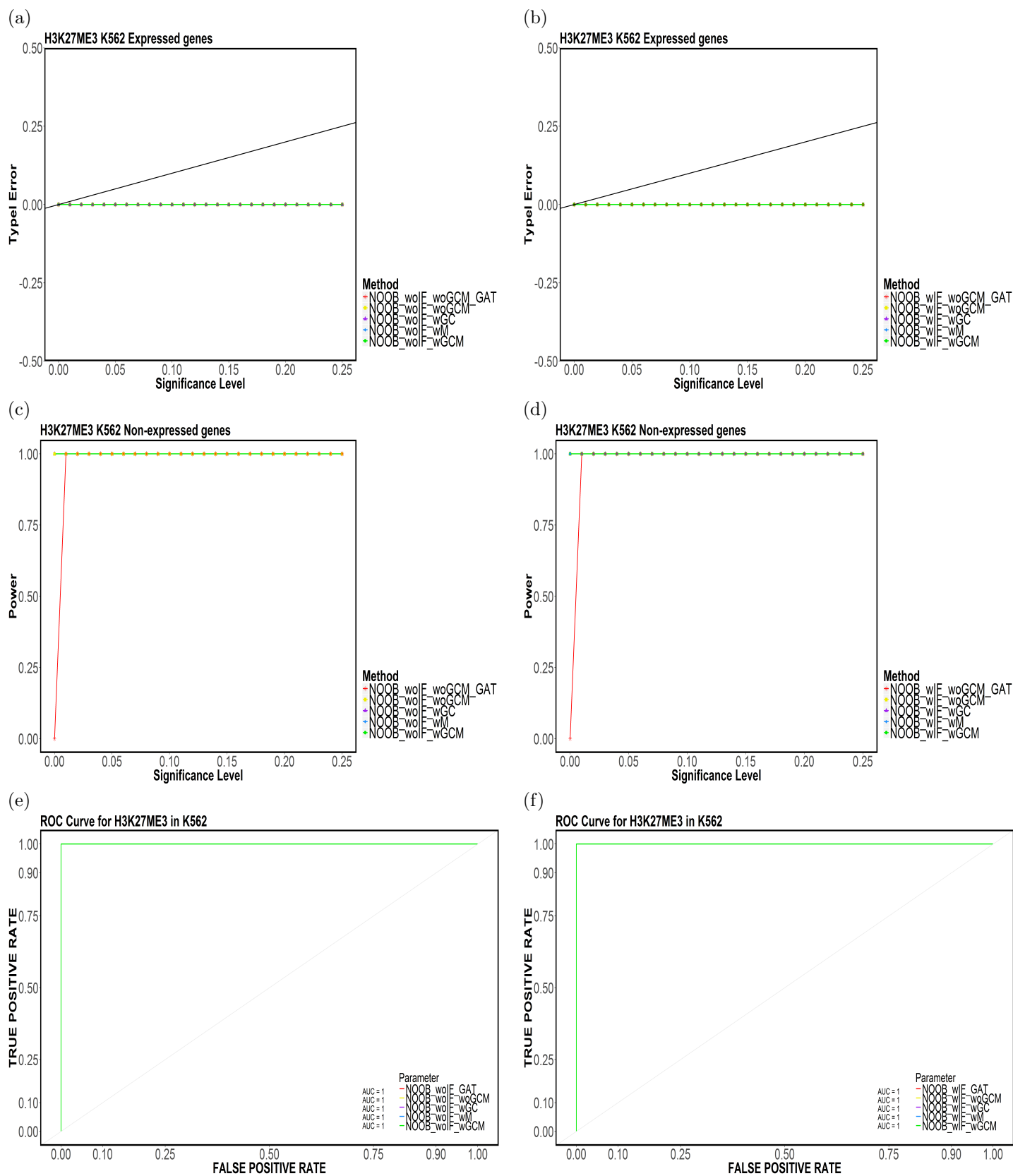
Figure 100: Element-based (a,b) Type-I Error, (c,d) Power and (e,f) ROC Curves for H3K27ME3 in K562 for (NOOB,TakeTheLongest,Top20).
