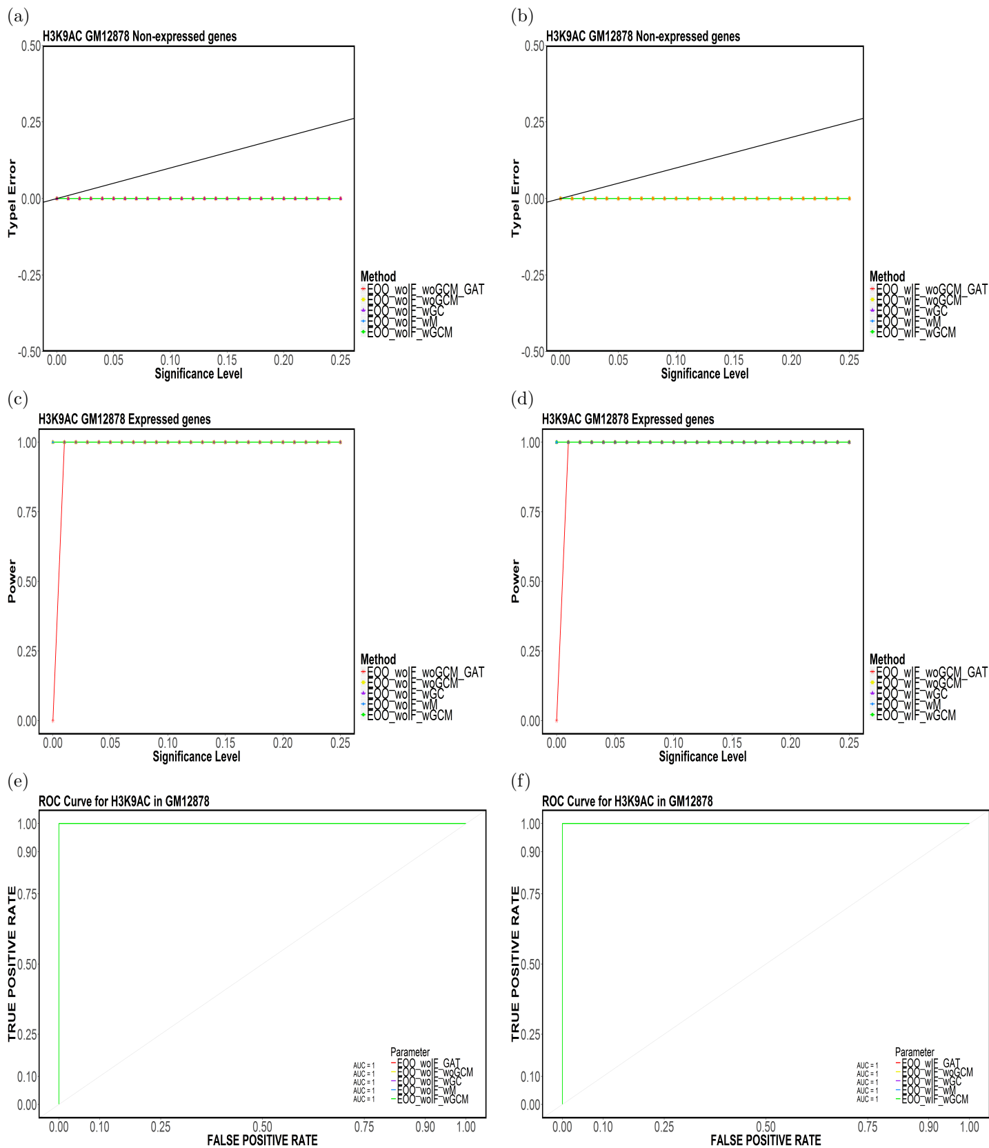
Figure 73: Element-based (a,b) Type-I Error, (c,d) Power and (e,f) ROC Curves for H3K9AC in GM12878 for (E00,CompletelyDiscard,Top5).
