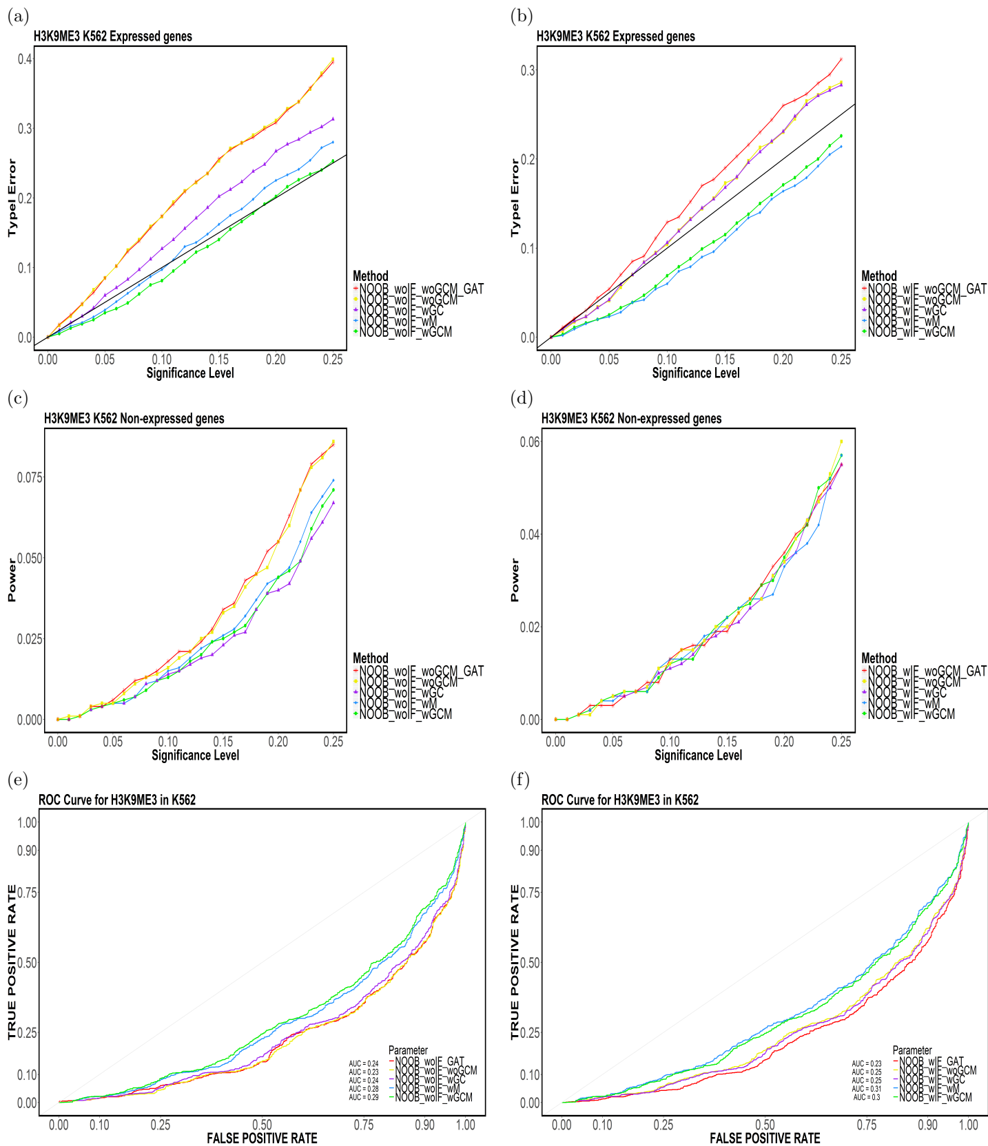
Figure 16: Element-based (a,b) Type-I Error, (c,d) Power and (e,f) ROC Curves for H3K9ME3 in K562 for (NOOB,TakeTheLongest,Top20).
