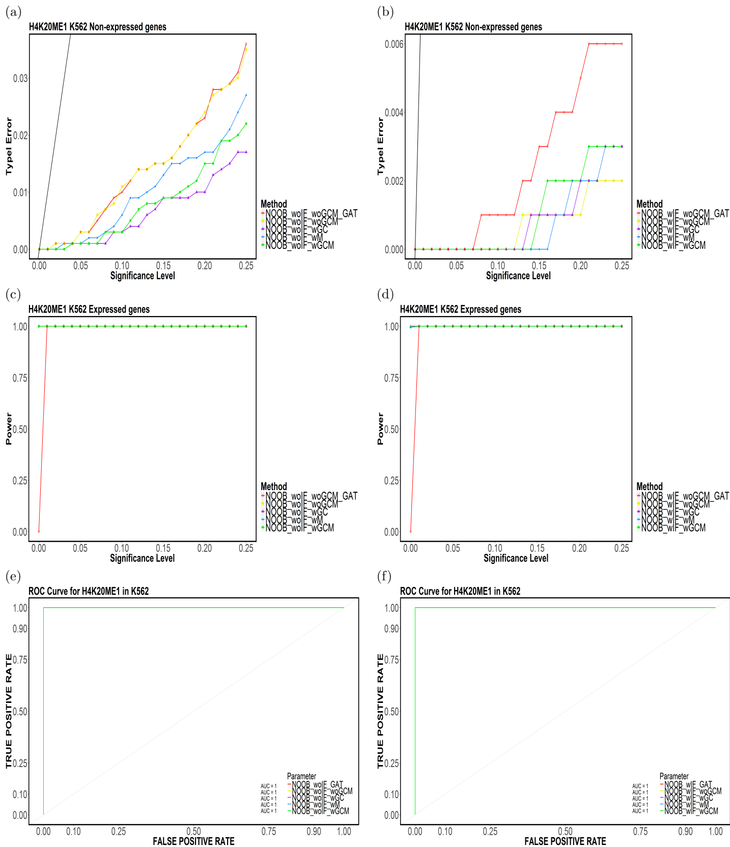
Figure 4: Element-based (a,b) Type-I Error, (c,d) Power and (e,f) ROC Curves for H4K20ME1 in K562 for (NOOB, CompletelyDiscard, Top5).
