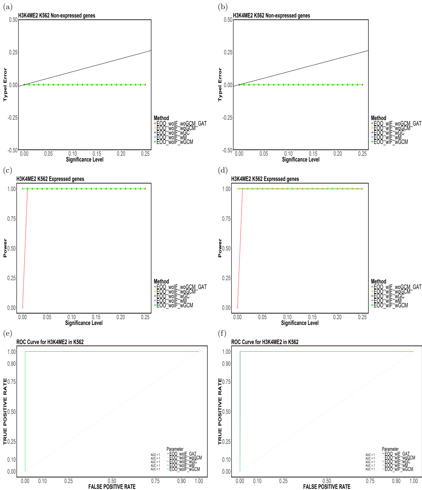
Figure 51: Element-based (a,b) Type-I Error, (c,d) Power and (e,f) ROC Curves for H3K4ME2 in K562 for (E00,CompletelyDiscard,Top5).
