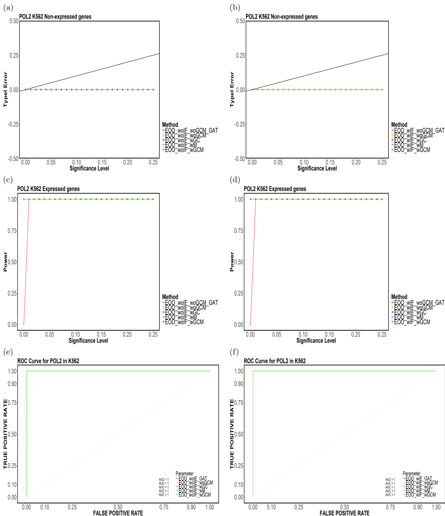
Figure 87: Element-based (a,b) Type-I Error, (c,d) Power and (e,f) ROC Curves for POL2 in K562 for (E00, CompletelyDiscard, Top5).
