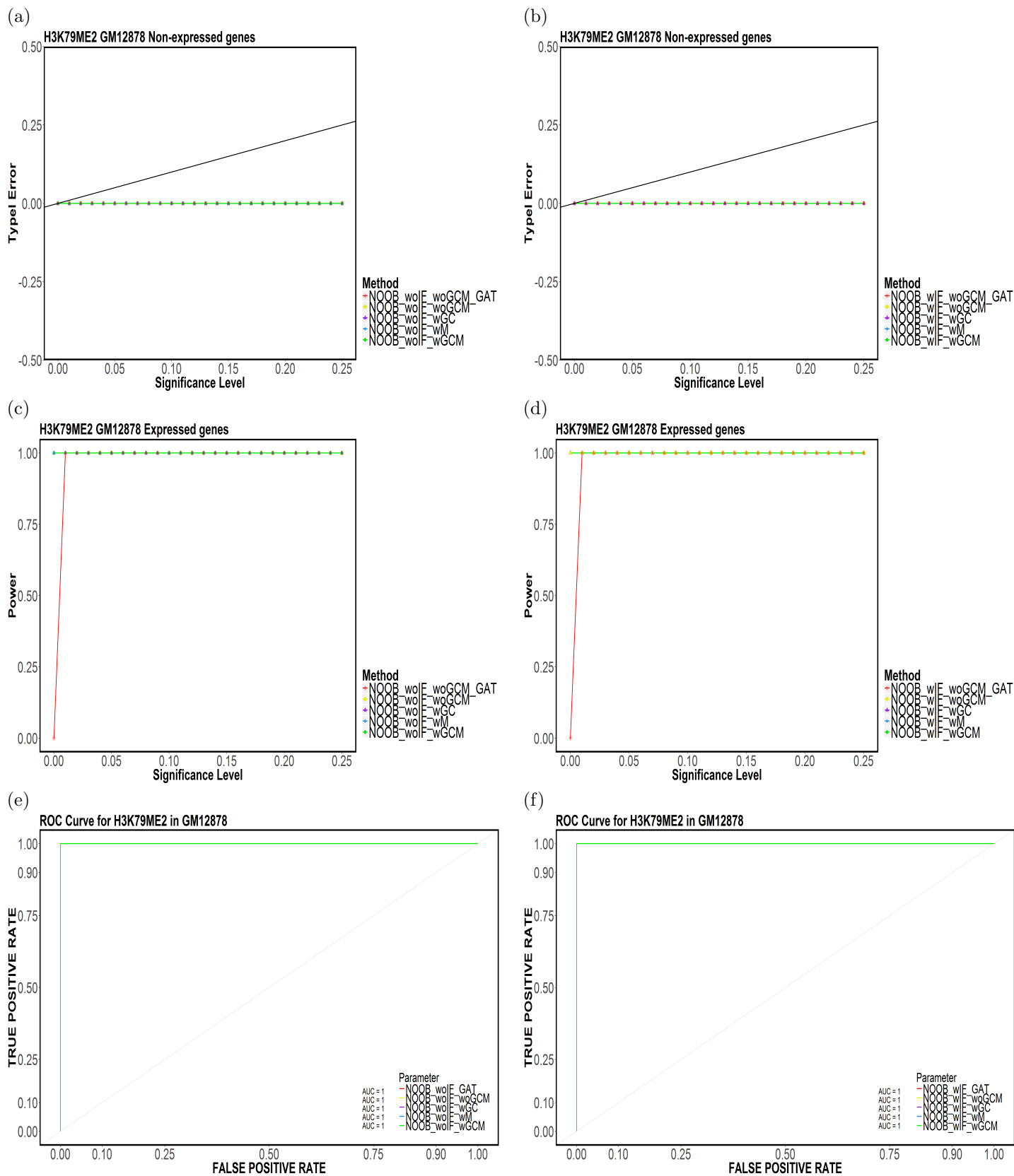
Figure 70: Element-based (a,b) Type-I Error, (c,d) Power and (e,f) ROC Curves for H3K79ME2 in GM12878 for (NOOB,TakeTheLongest,Top20).
