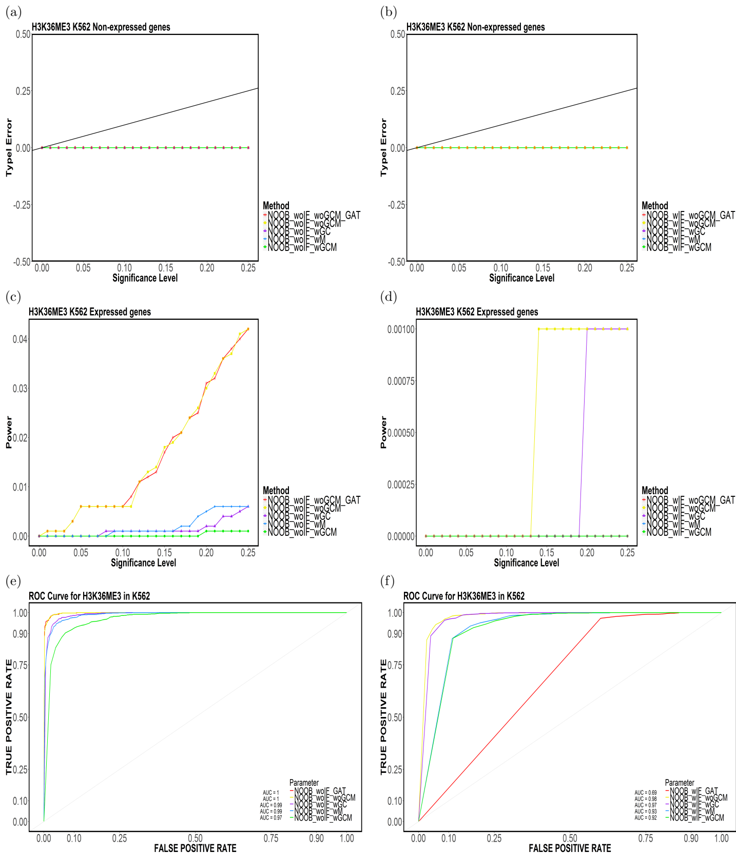
Figure 32: Element-based (a,b) Type-I Error, (c,d) Power and (e,f) ROC Curves for H3K36ME3 in K562 for (NOOB,TakeTheLongest,Top20).
