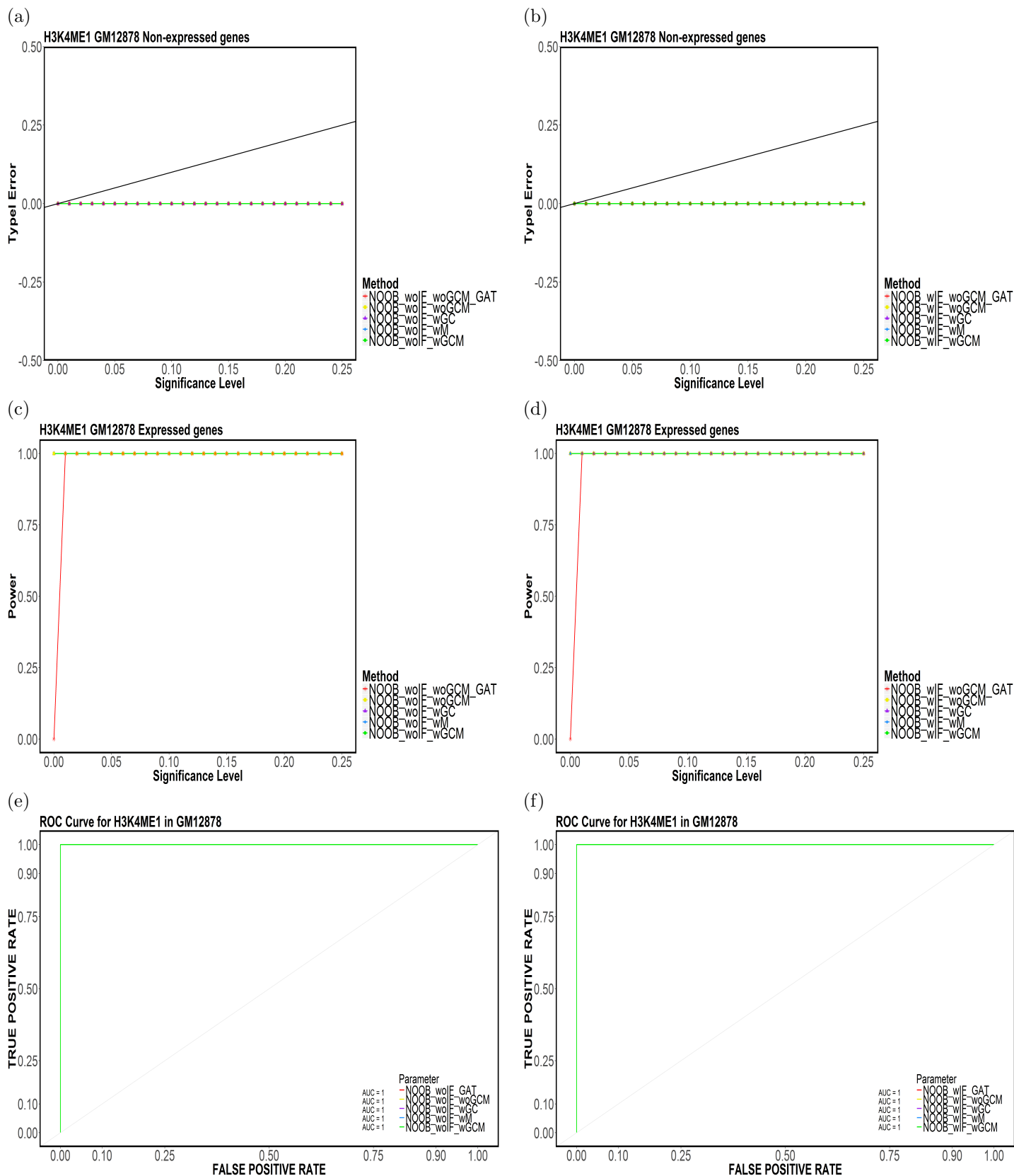
Figure 18: Element-based (a,b) Type-I Error, (c,d) Power and (e,f) ROC Curves for H3K4ME1 in GM12878 for (NOOB, CompletelyDiscard, Top5).
