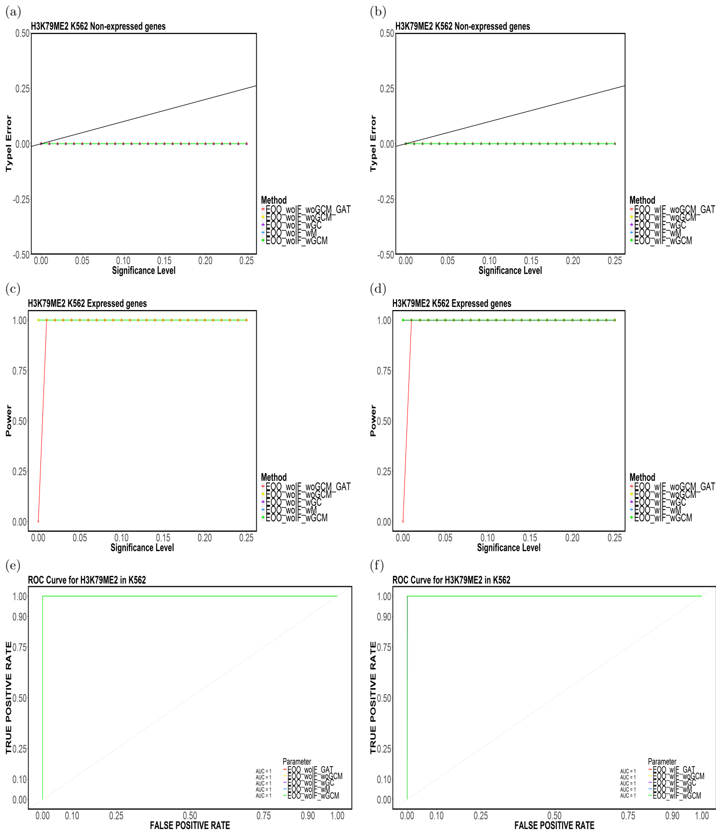
Figure 67: Element-based (a,b) Type-I Error, (c,d) Power and (e,f) ROC Curves for H3K79ME2 in K562 for (E00,CompletelyDiscard,Top5).
