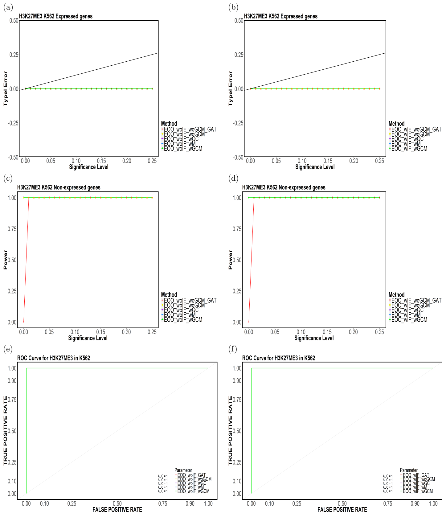
Figure 95: Element-based (a,b) Type-I Error, (c,d) Power and (e,f) ROC Curves for H3K27ME3 in K562 for (E00,CompletelyDiscard,Top5).
