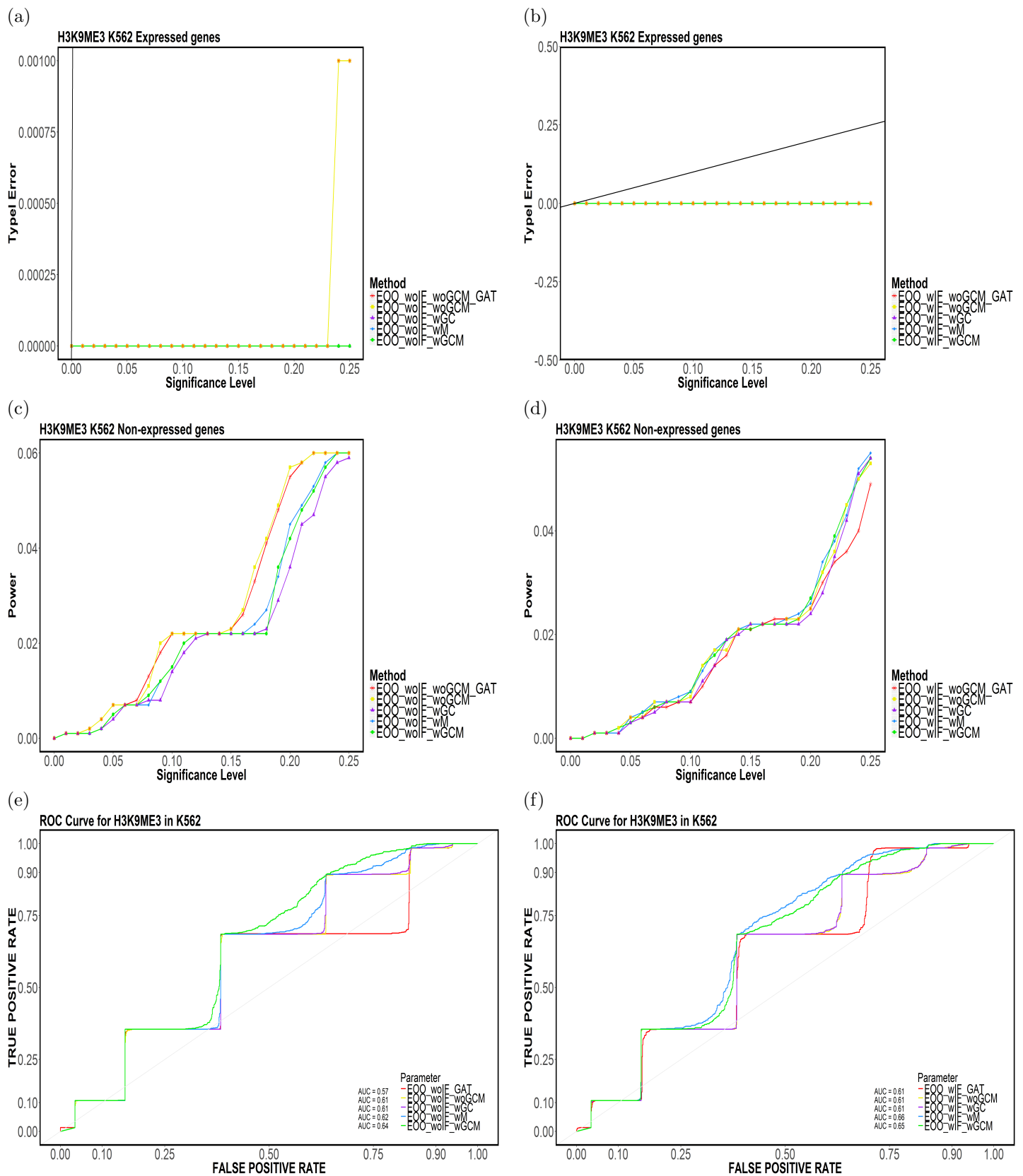
Figure 11: Element-based (a,b) Type-I Error, (c,d) Power and (e,f) ROC Curves for H3K9ME3 in K562 for (E00,CompletelyDiscard,Top5).
