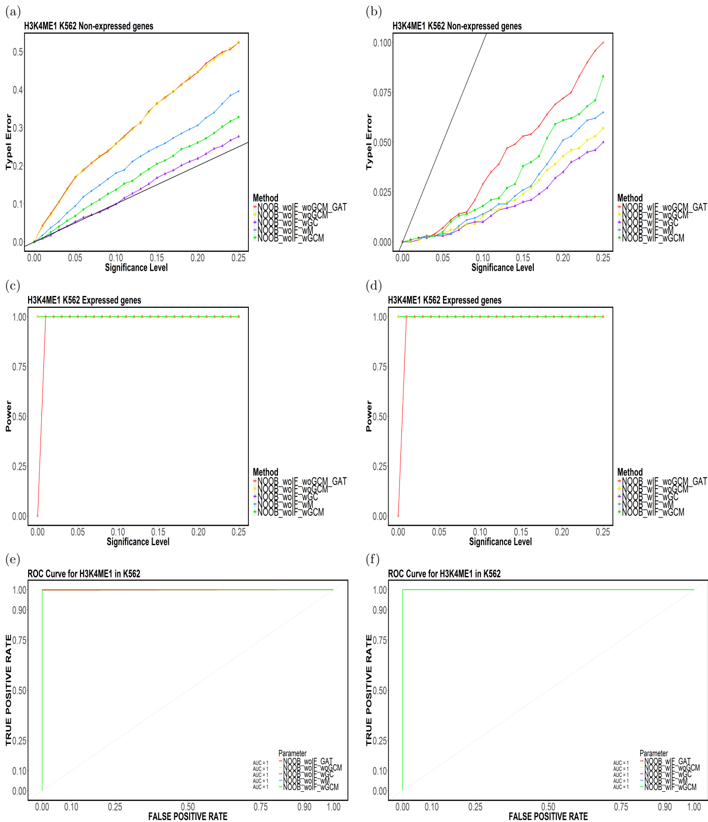
Figure 20: Element-based (a,b) Type-I Error, (c,d) Power and (e,f) ROC Curves for H3K4ME1 in K562 for (NOOB, CompletelyDiscard, Top5).
