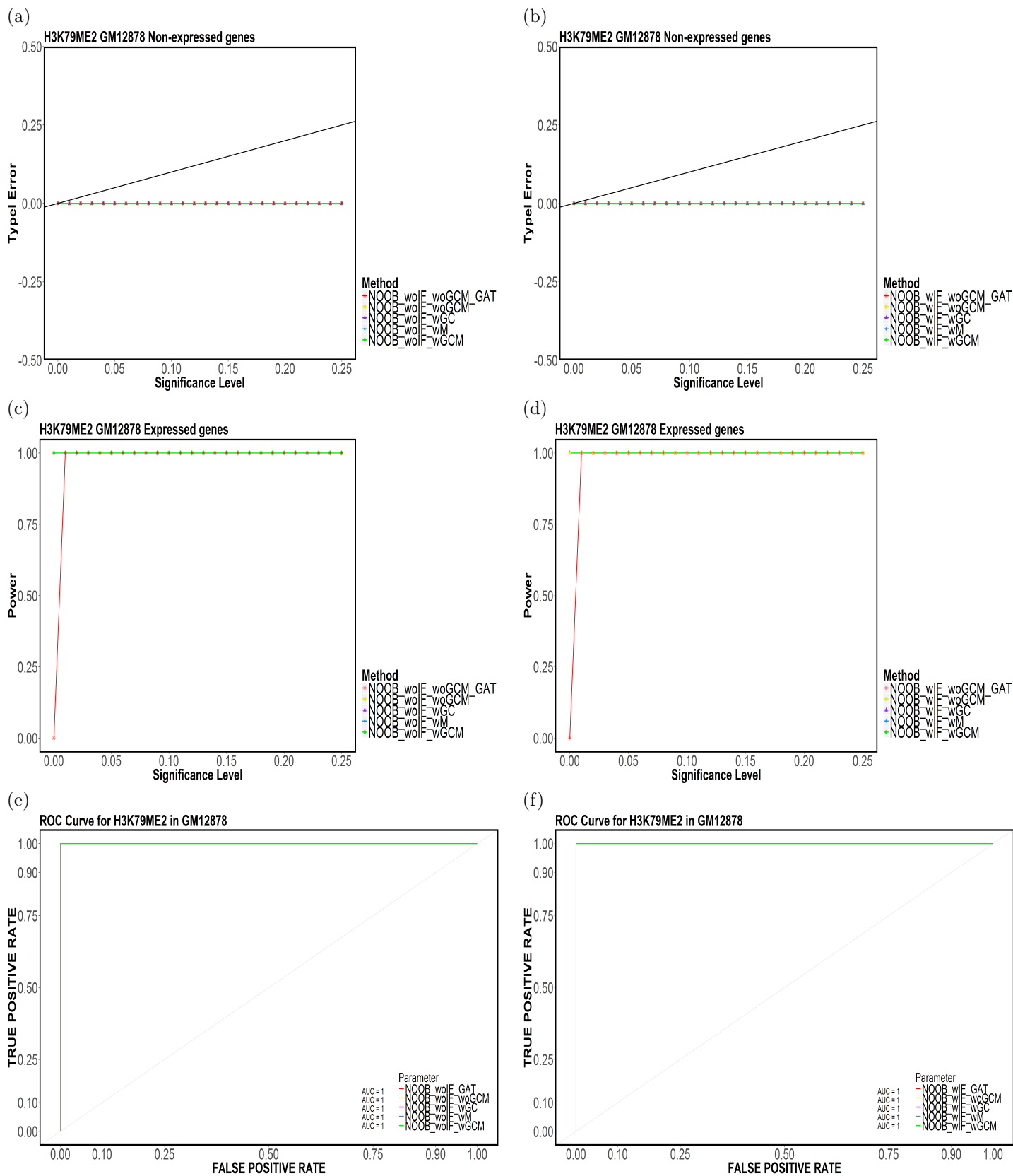
Figure 66: Element-based (a,b) Type-I Error, (c,d) Power and (e,f) ROC Curves for H3K79ME2 in GM12878 for (NOOB,CompletelyDiscard,Top5).
