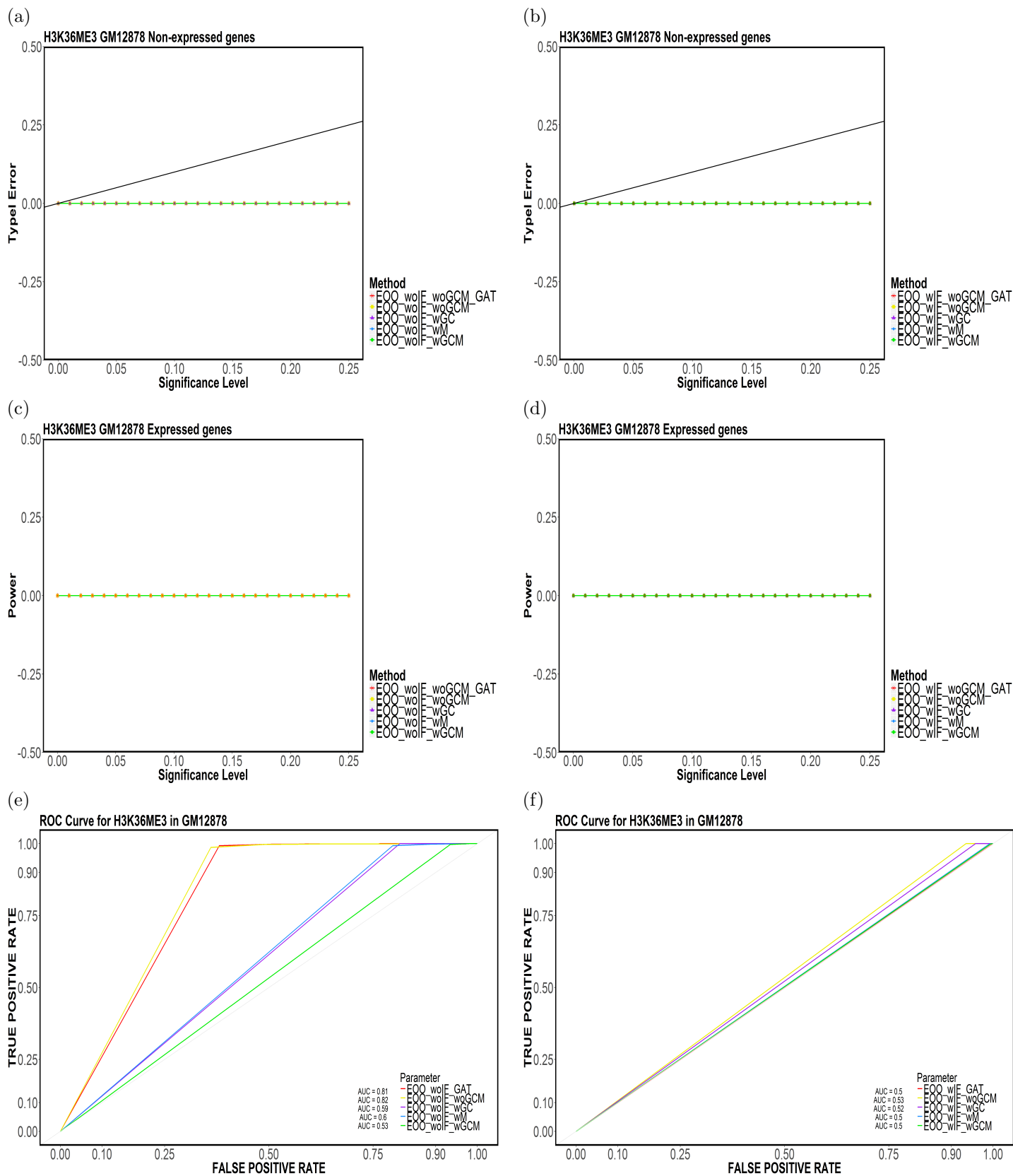
Figure 25: Element-based (a,b) Type-I Error, (c,d) Power and (e,f) ROC Curves for H3K36ME3 in GM12878 for (E00,CompletelyDiscard,Top5).
