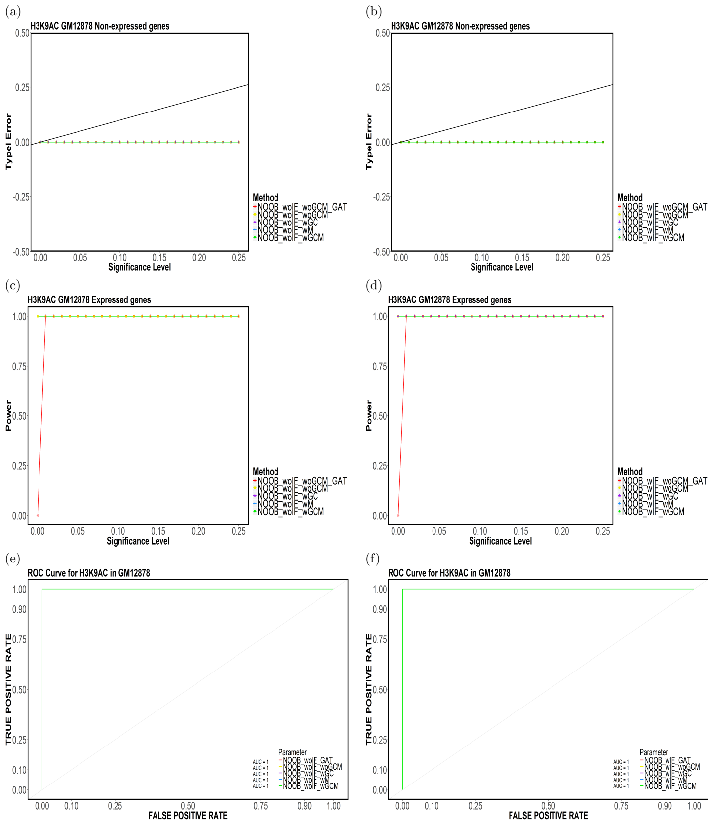
Figure 74: Element-based (a,b) Type-I Error, (c,d) Power and (e,f) ROC Curves for H3K9AC in GM12878 for (NOOB, CompletelyDiscard, Top5).
