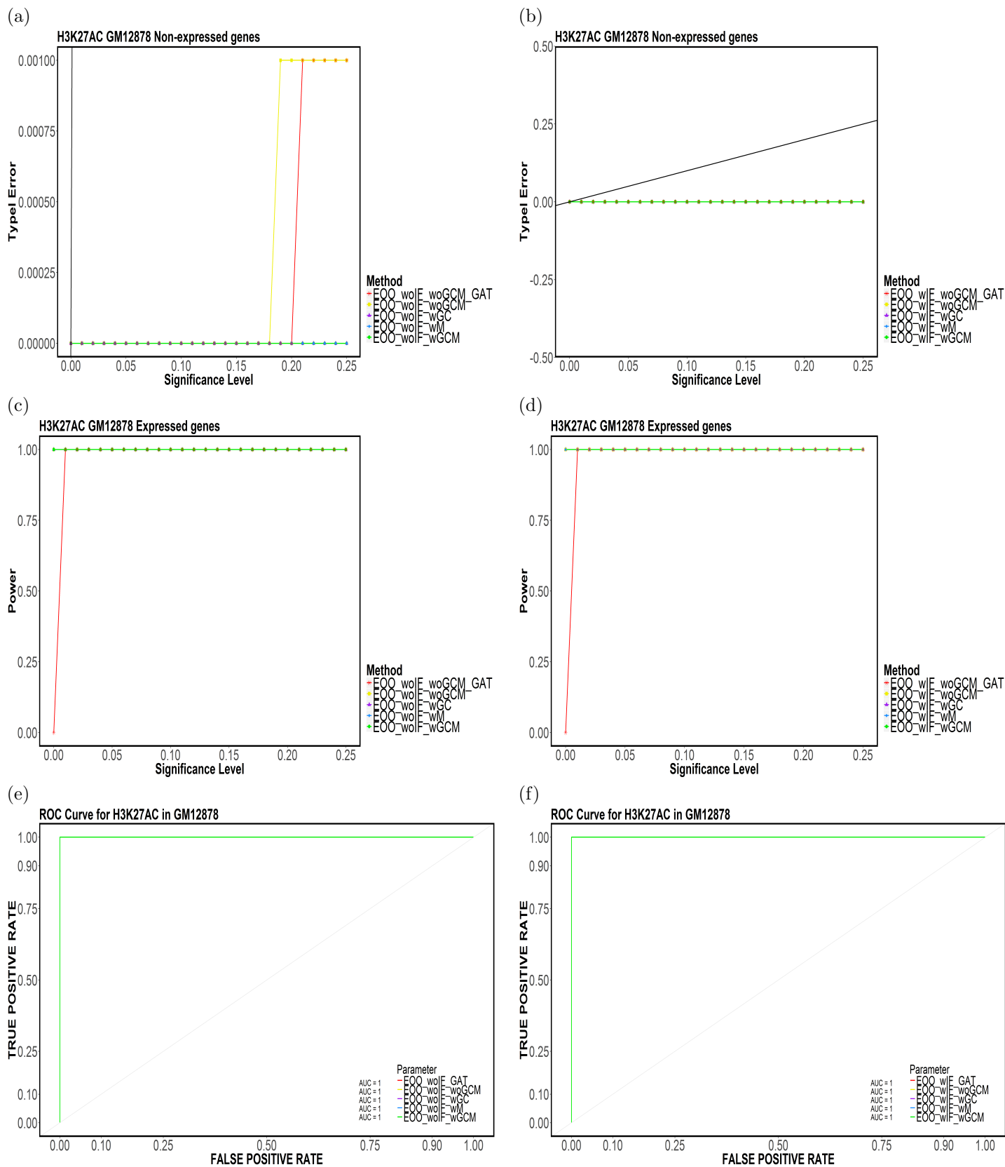
Figure 45: Element-based (a,b) Type-I Error, (c,d) Power and (e,f) ROC Curves for H3K27AC in GM12878 for (E00,TakeTheLongest,Top20).
