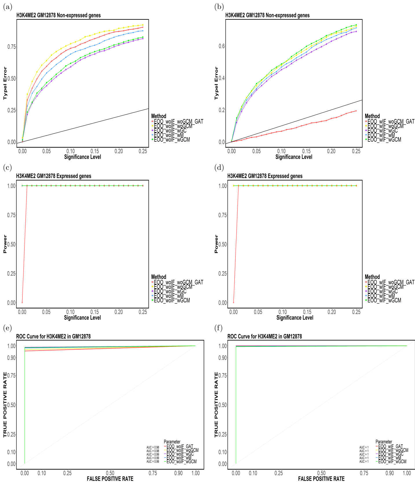
Figure 53: Element-based (a,b) Type-I Error, (c,d) Power and (e,f) ROC Curves for H3K4ME2 in GM12878 for (E00,TakeTheLongest,Top20).
