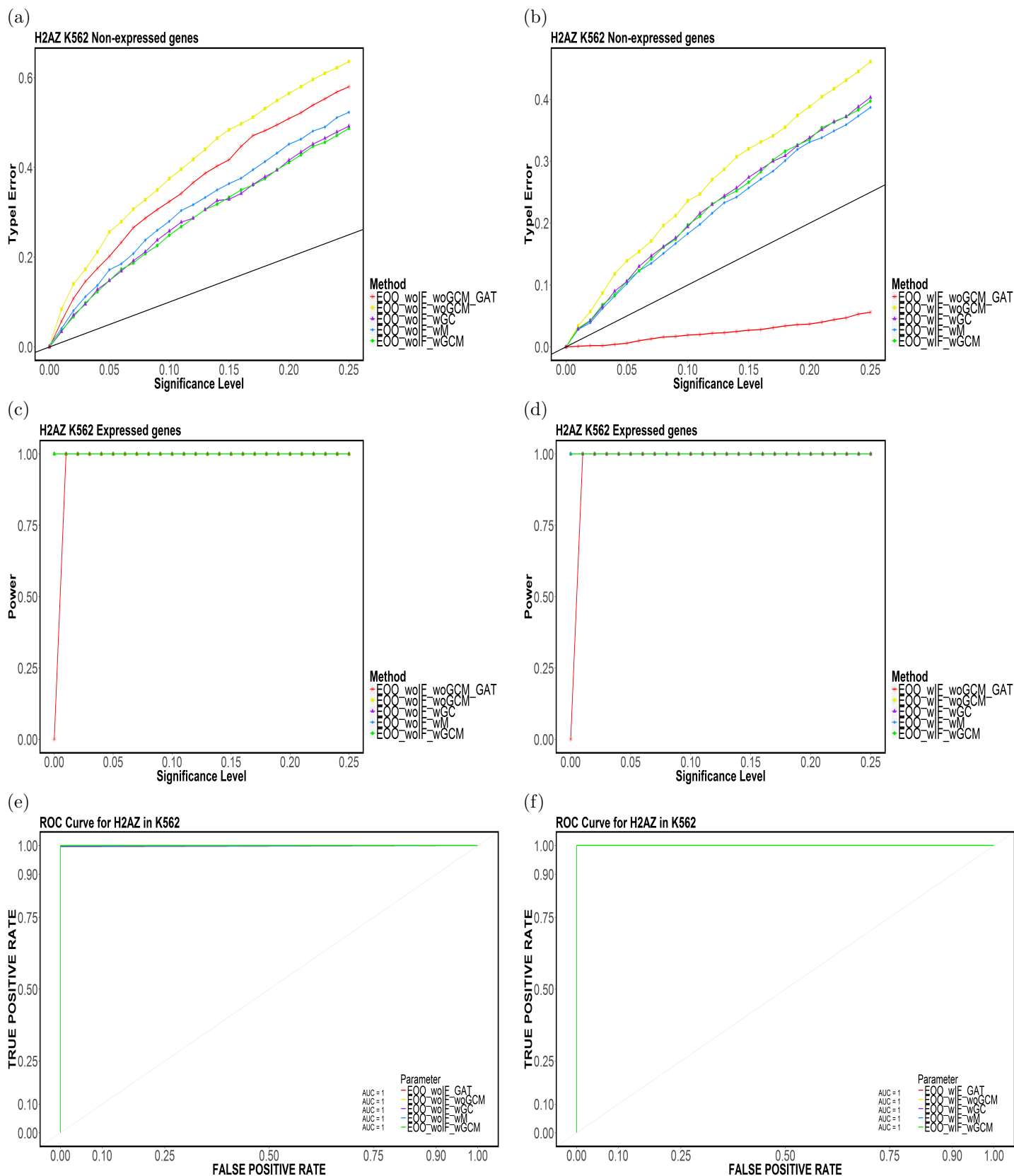
Figure 39: Element-based (a,b) Type-I Error, (c,d) Power and (e,f) ROC Curves for H2AZ in K562 for (EOO,TakeTheLongest,Top20).
