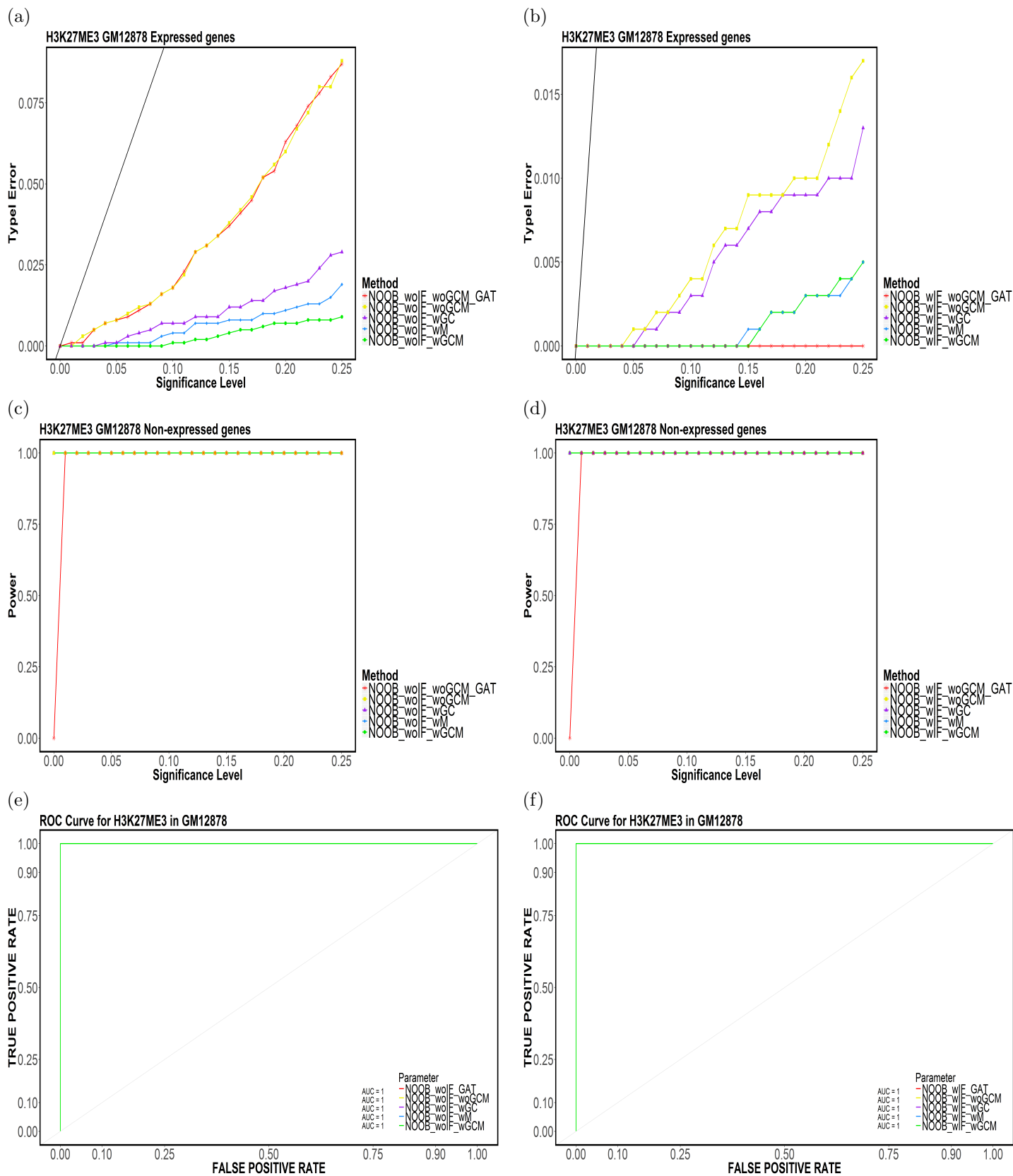
Figure 98: Element-based (a,b) Type-I Error, (c,d) Power and (e,f) ROC Curves for H3K27ME3 in GM12878 for (NOOB,TakeTheLongest,Top20).
