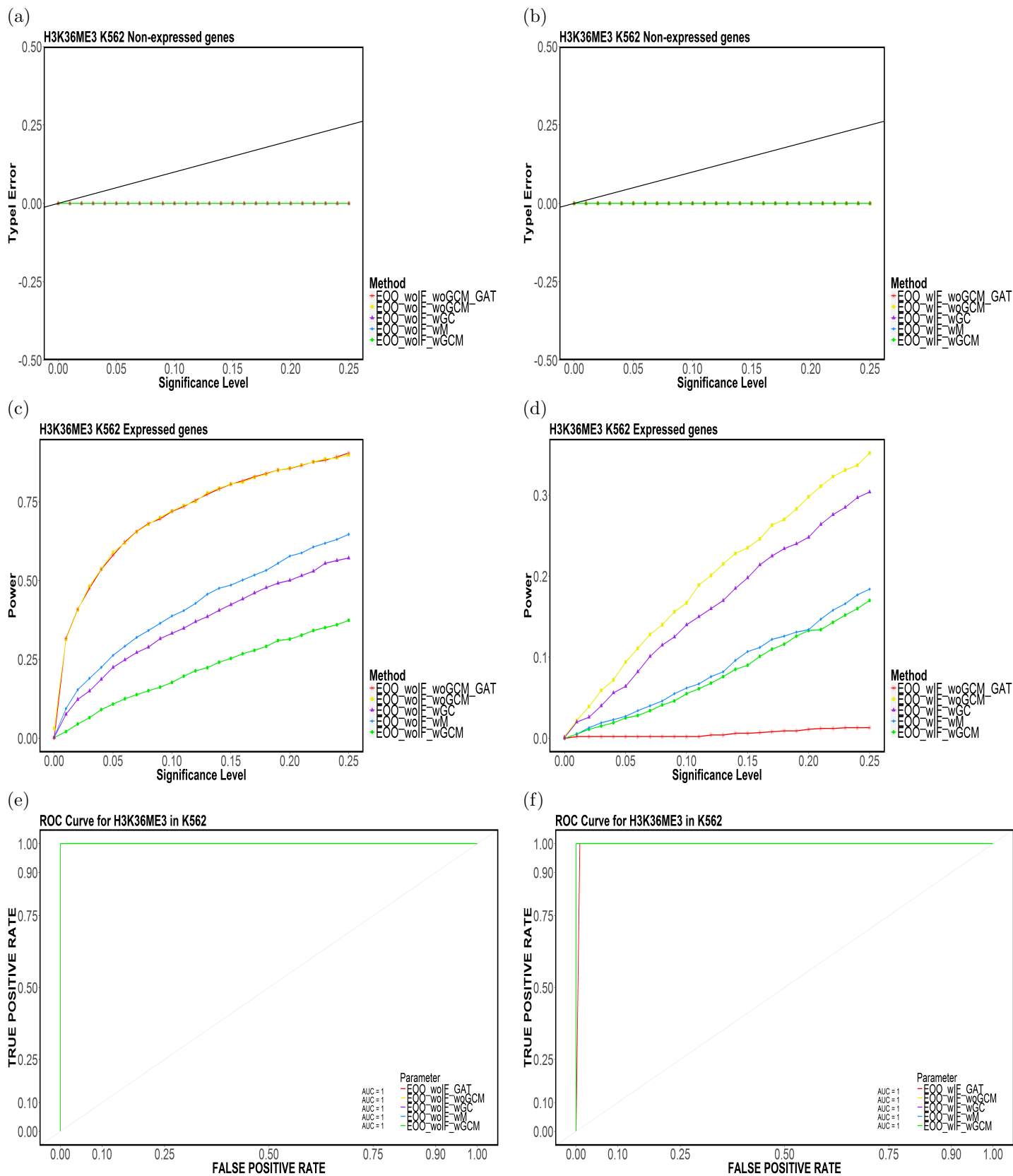
Figure 31: Element-based (a,b) Type-I Error, (c,d) Power and (e,f) ROC Curves for H3K36ME3 in K562 for (EOO,TakeTheLongest,Top20).
