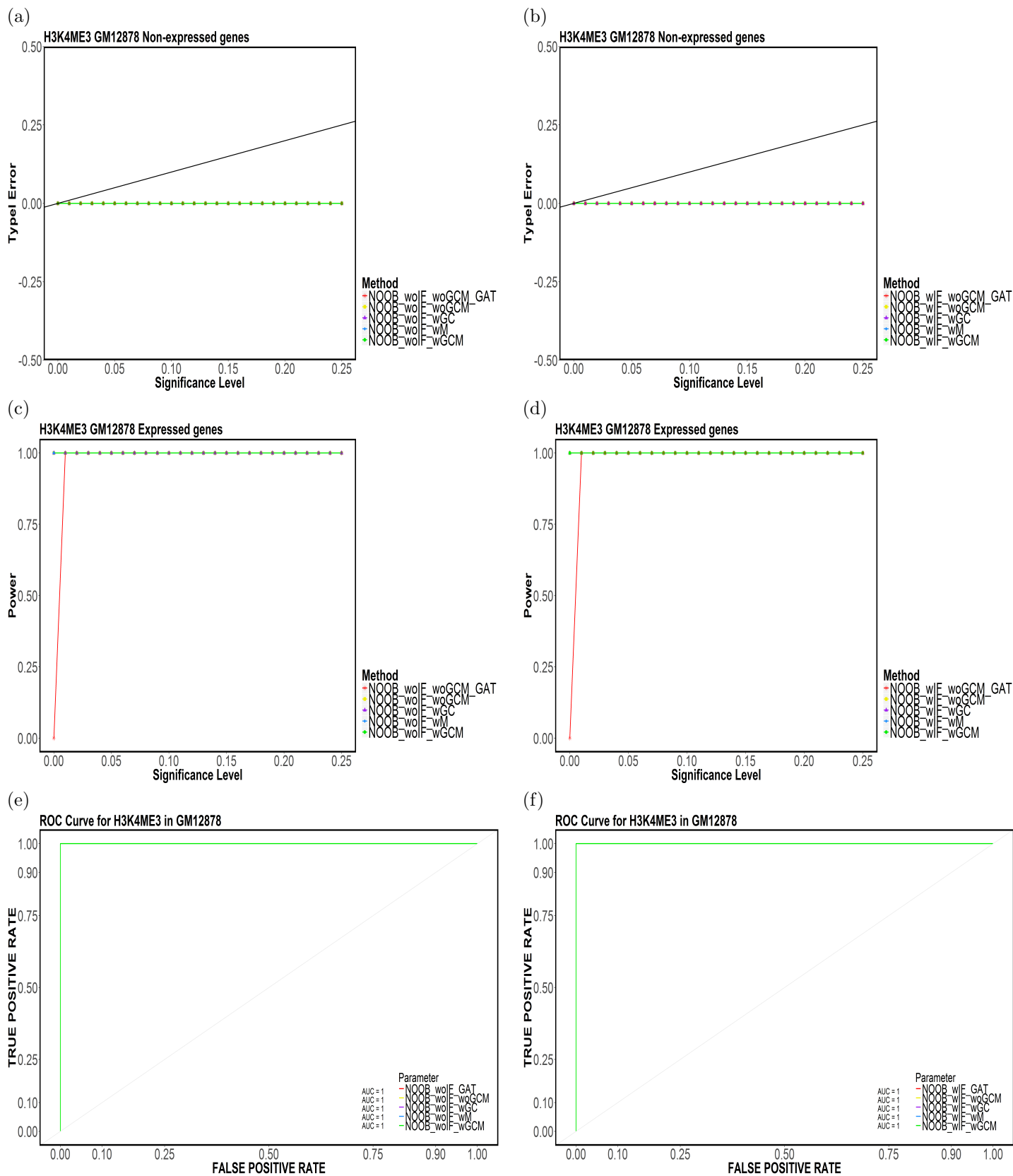
Figure 58: Element-based (a,b) Type-I Error, (c,d) Power and (e,f) ROC Curves for H3K4ME3 in GM12878 for (NOOB,CompletelyDiscard,Top5).
