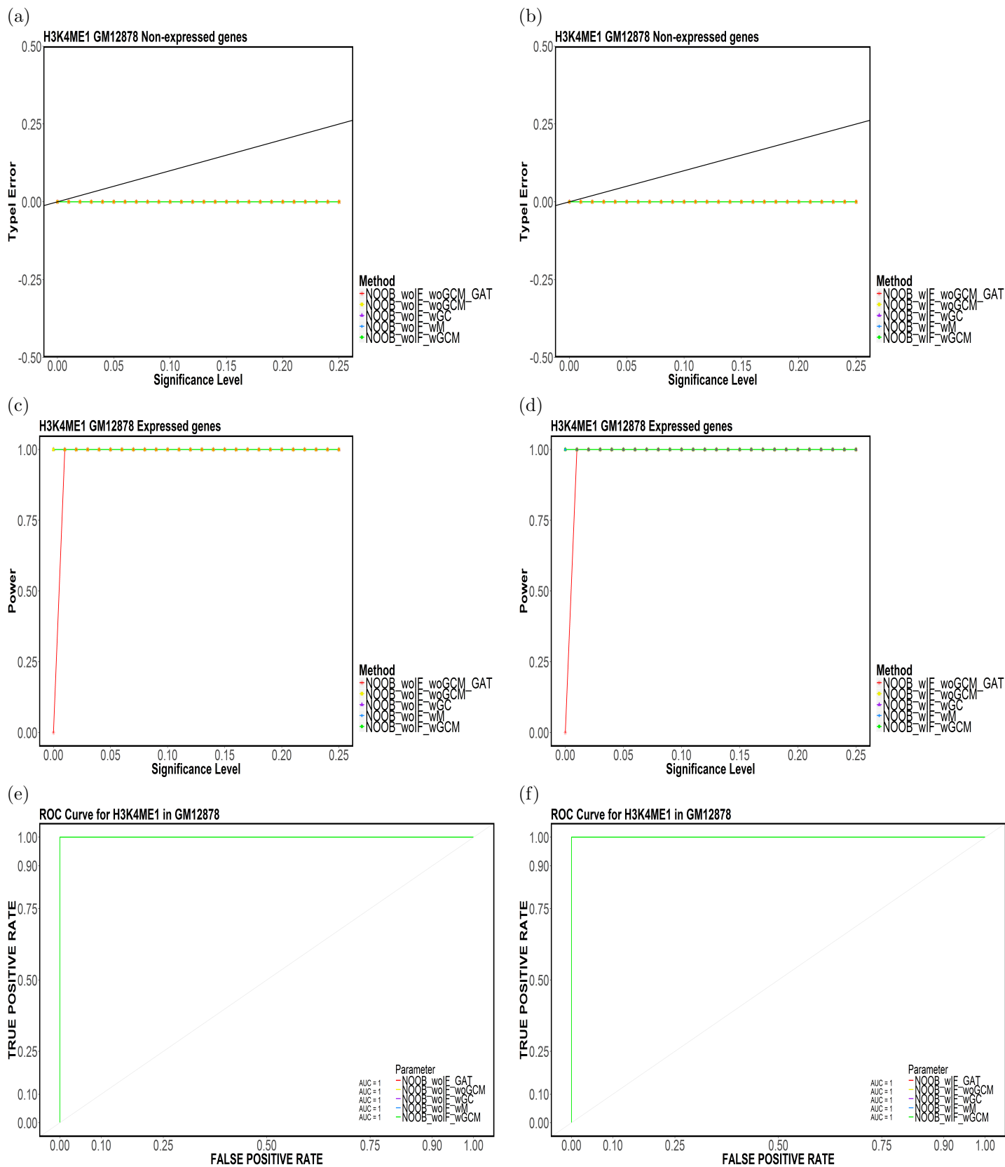
Figure 22: Element-based (a,b) Type-I Error, (c,d) Power and (e,f) ROC Curves for H3K4ME1 in GM12878 for (NOOB,TakeTheLongest,Top20).
