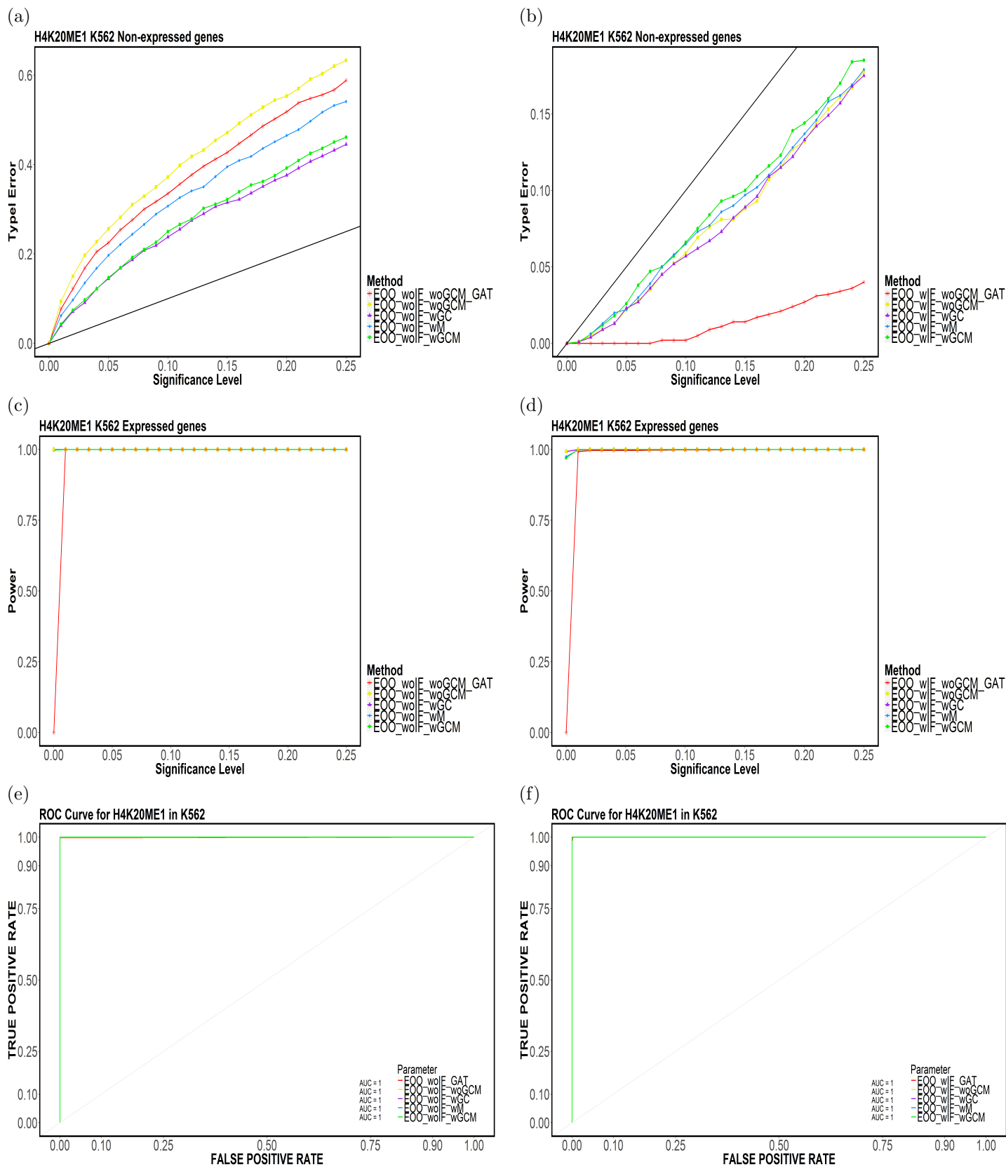
Figure 7: Element-based (a,b) Type-I Error, (c,d) Power and (e,f) ROC Curves for H4K20ME1 in K562 for (E00,TakeTheLongest,Top20).
