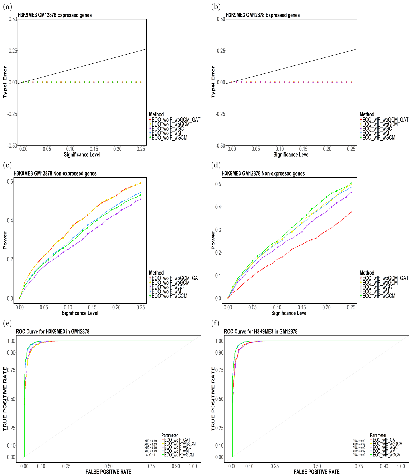
Figure 9: Element-based (a,b) Type-I Error, (c,d) Power and (e,f) ROC Curves for H3K9ME3 in GM12878 for (E00, CompletelyDiscard, Top5).
