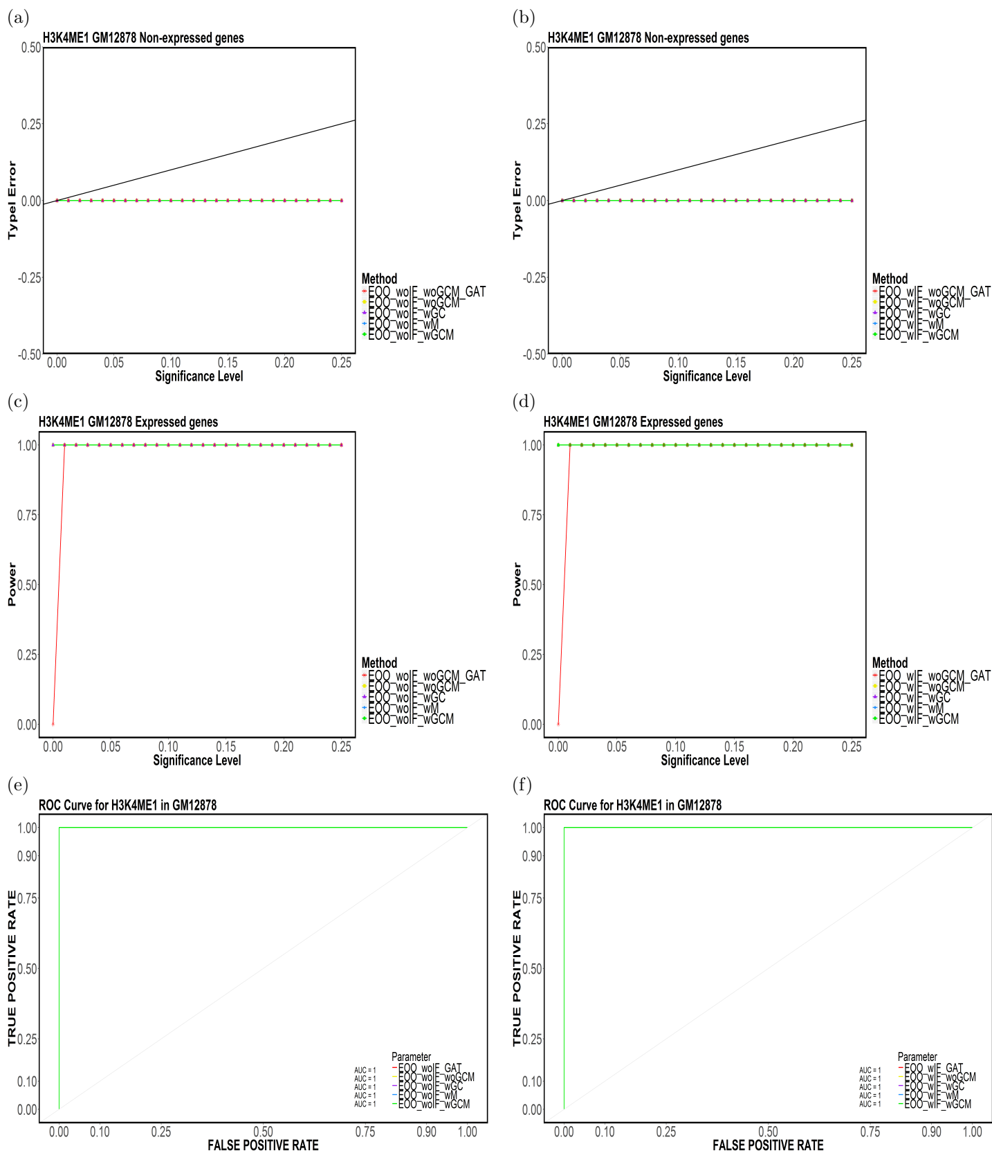
Figure 17: Element-based (a,b) Type-I Error, (c,d) Power and (e,f) ROC Curves for H3K4ME1 in GM12878 for (E00,CompletelyDiscard,Top5).
