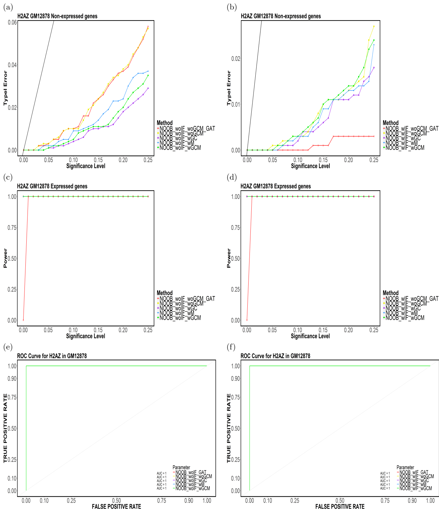
Figure 38: Element-based (a,b) Type-I Error, (c,d) Power and (e,f) ROC Curves for H2AZ in GM12878 for (NOOB,TakeTheLongest,Top20).
