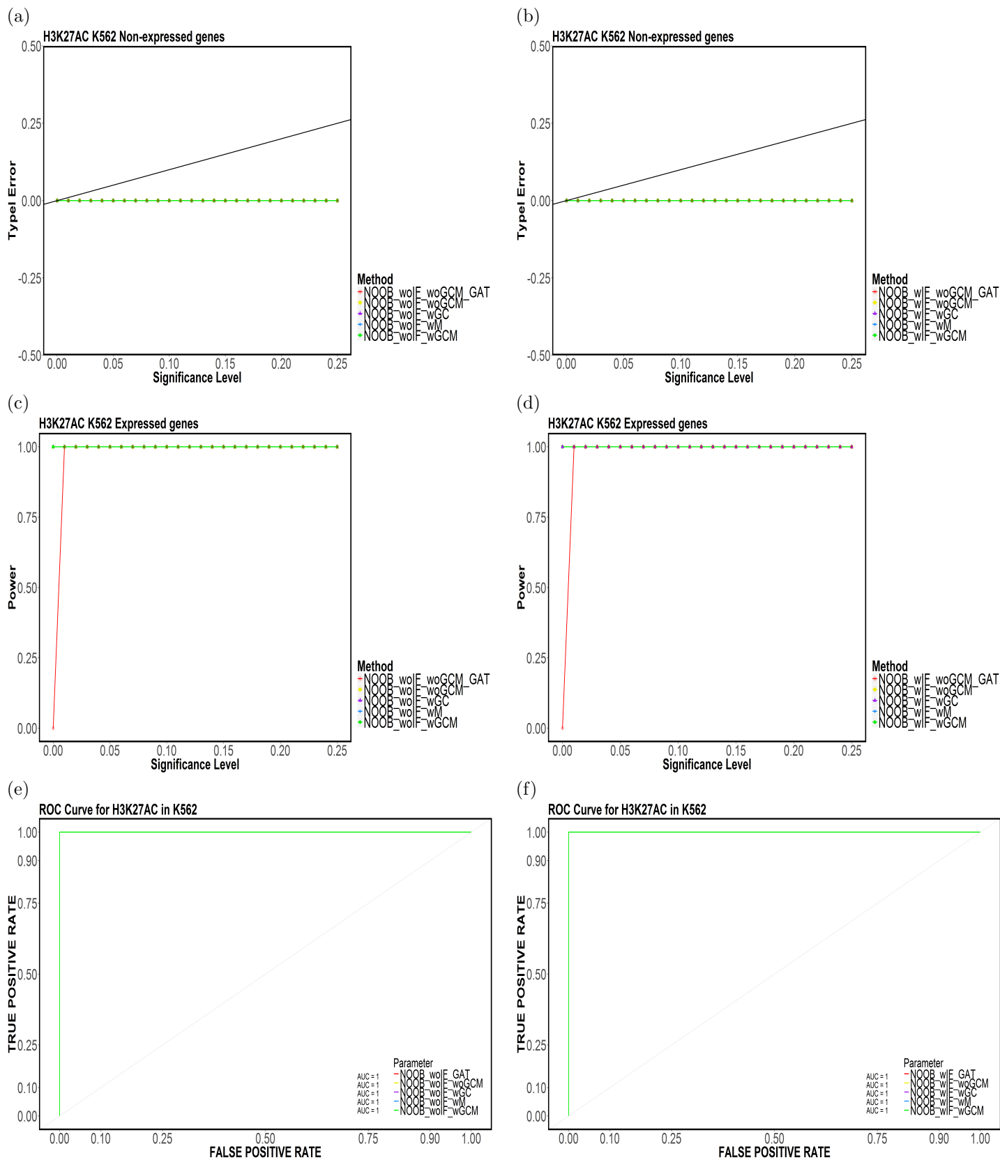
Figure 48: Element-based (a,b) Type-I Error, (c,d) Power and (e,f) ROC Curves for H3K27AC in K562 for (NOOB,TakeTheLongest,Top20).
