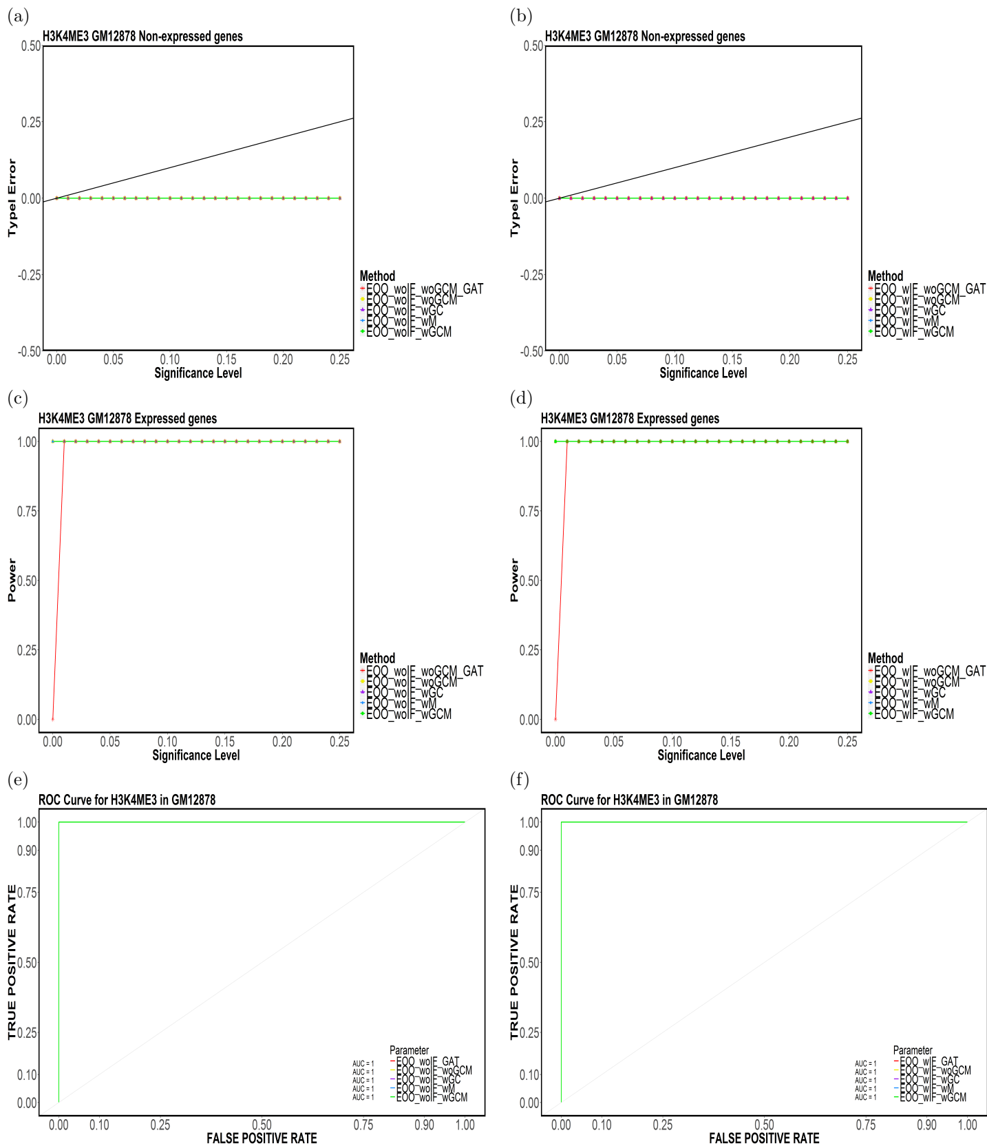
Figure 57: Element-based (a,b) Type-I Error, (c,d) Power and (e,f) ROC Curves for H3K4ME3 in GM12878 for (E00,CompletelyDiscard,Top5).
