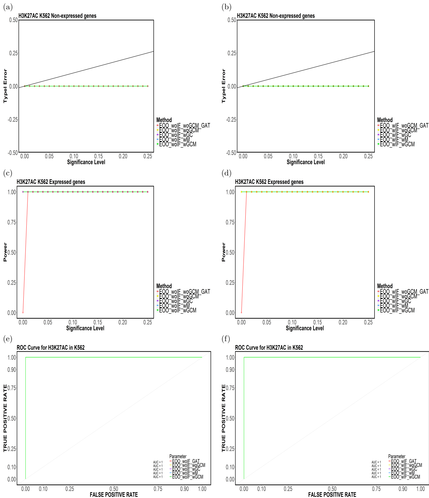
Figure 43: Element-based (a,b) Type-I Error, (c,d) Power and (e,f) ROC Curves for H3K27AC in K562 for (E00,CompletelyDiscard,Top5).
