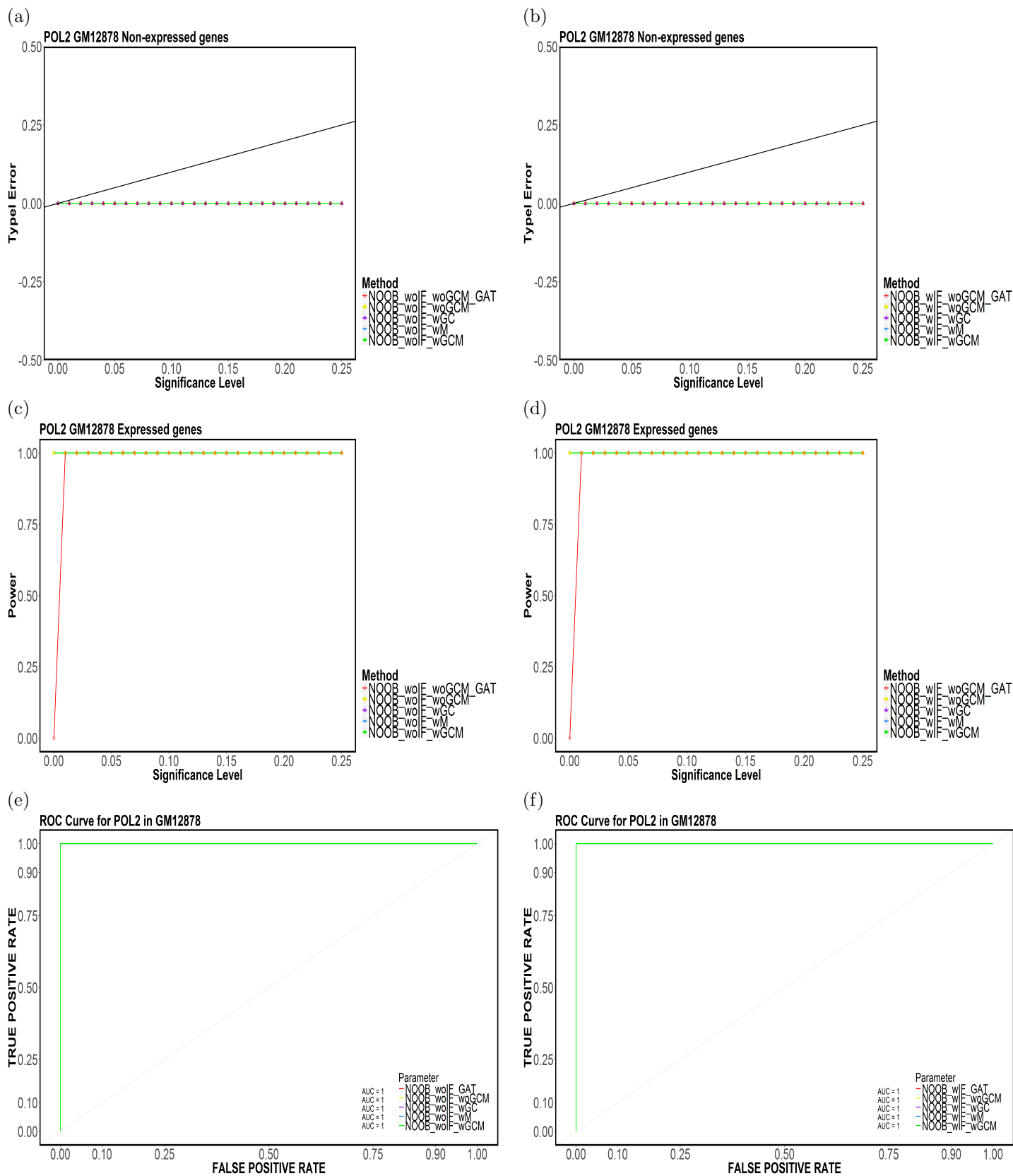
Figure 90: Element-based (a,b) Type-I Error, (c,d) Power and (e,f) ROC Curves for POL2 in GM12878 for (NOOB,TakeTheLongest,Top20).
