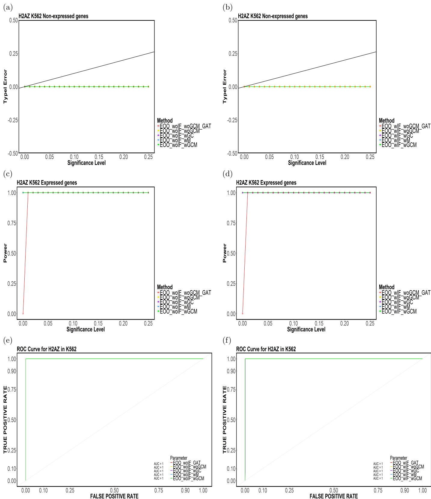
Figure 35: Element-based (a,b) Type-I Error, (c,d) Power and (e,f) ROC Curves for H2AZ in K562 for (E00,CompletelyDiscard,Top5).
