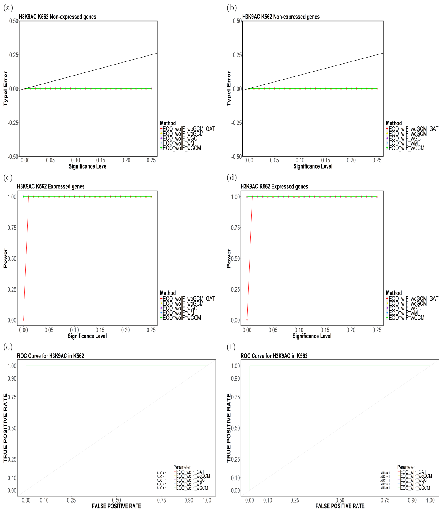
Figure 75: Element-based (a,b) Type-I Error, (c,d) Power and (e,f) ROC Curves for H3K9AC in K562 for (E00,CompletelyDiscard,Top5).
