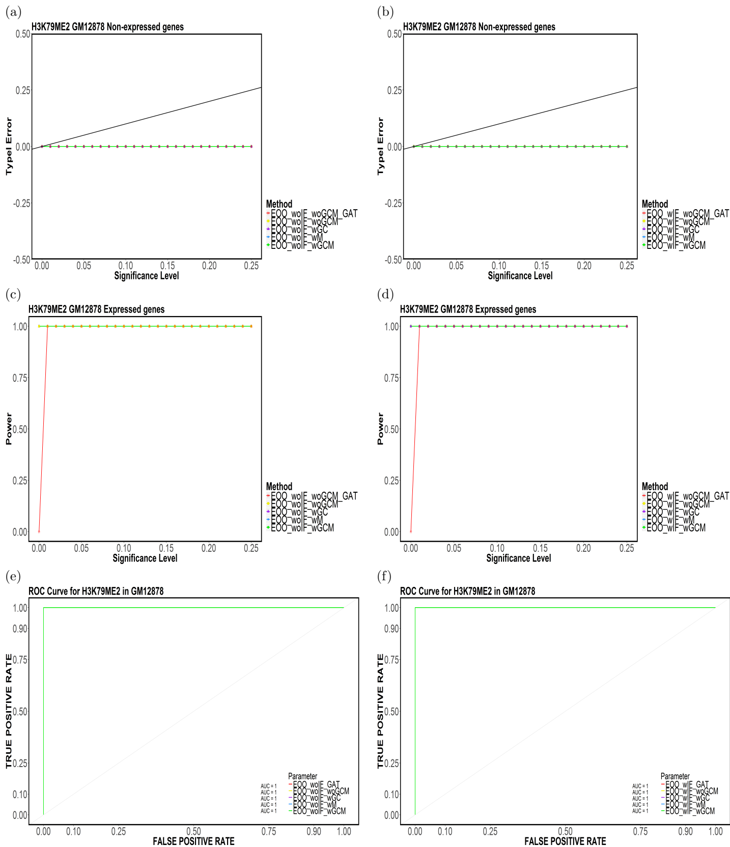
Figure 69: Element-based (a,b) Type-I Error, (c,d) Power and (e,f) ROC Curves for H3K79ME2 in GM12878 for (E00,TakeTheLongest,Top20).
