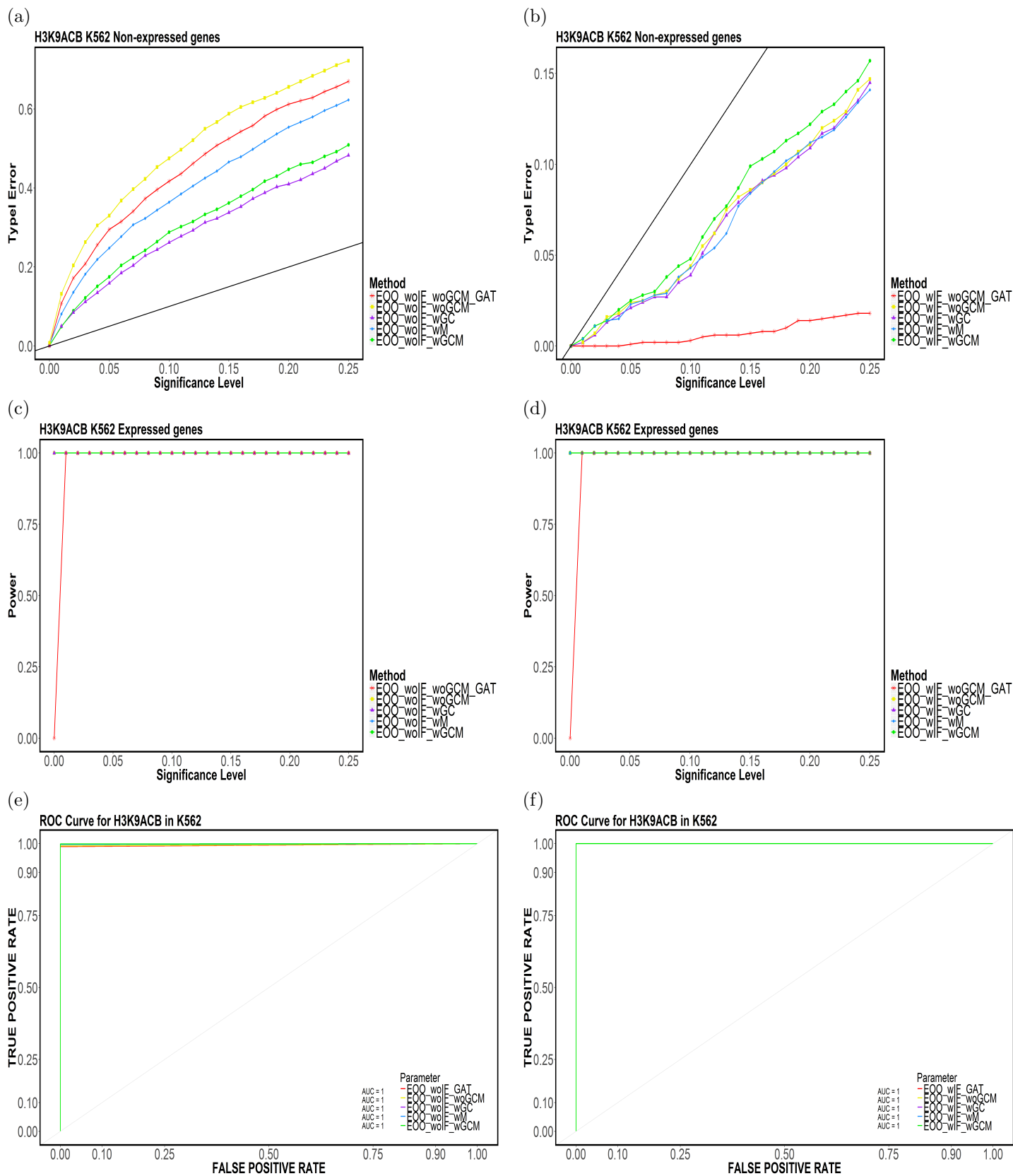
Figure 83: Element-based (a,b) Type-I Error, (c,d) Power and (e,f) ROC Curves for H3K9ACB in K562 for (E00,TakeTheLongest,Top20).
