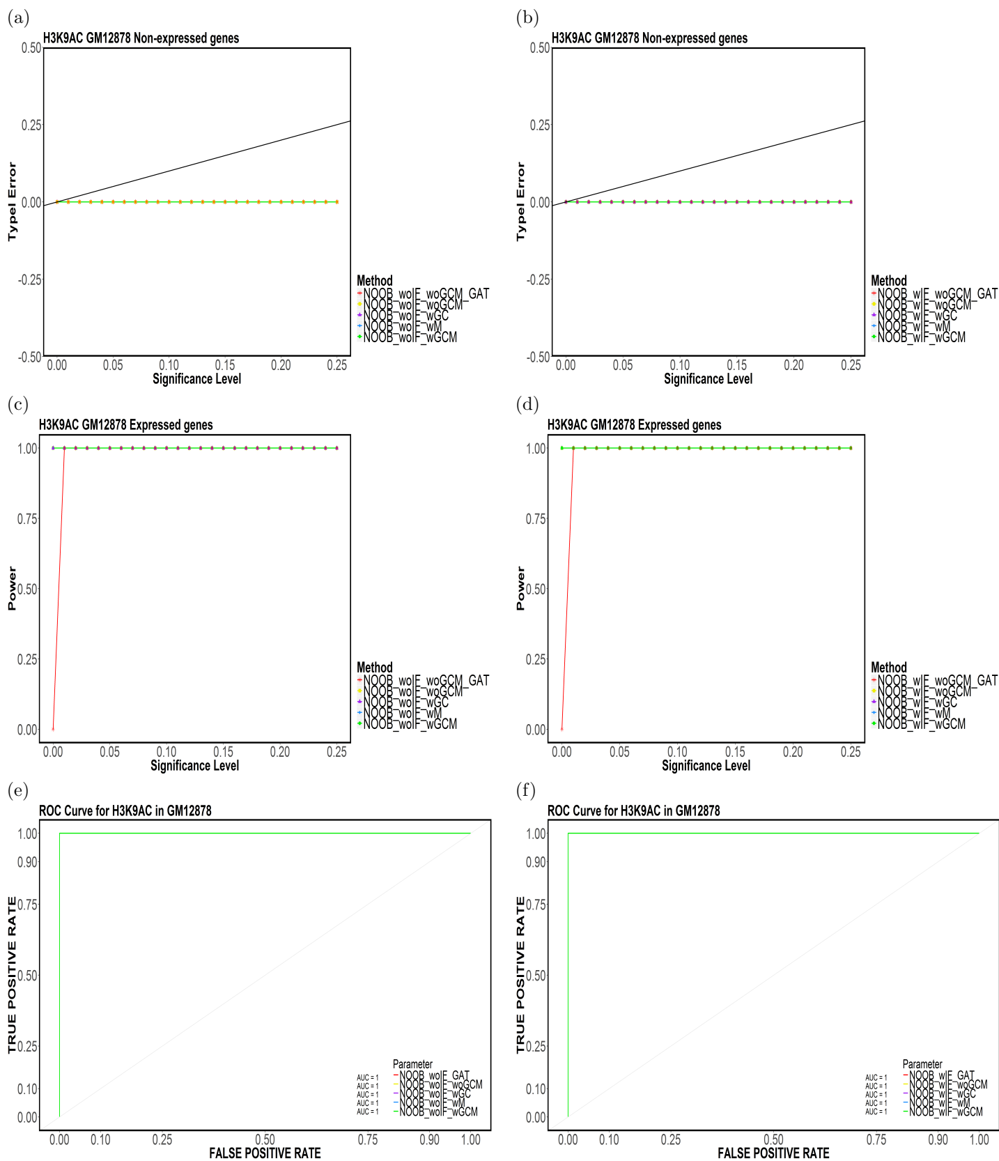
Figure 78: Element-based (a,b) Type-I Error, (c,d) Power and (e,f) ROC Curves for H3K9AC in GM12878 for (NOOB,TakeTheLongest,Top20).
