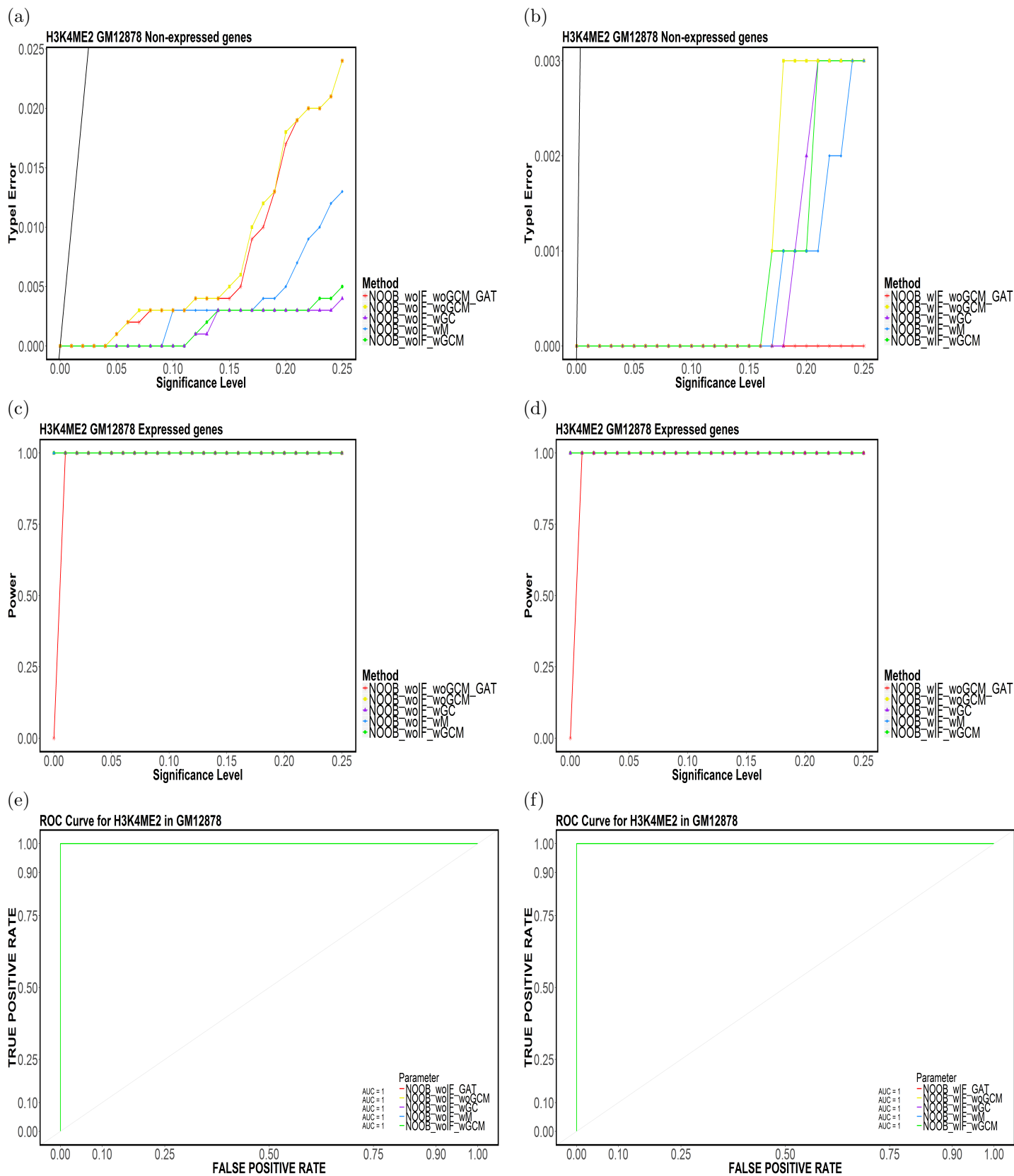
Figure 54: Element-based (a,b) Type-I Error, (c,d) Power and (e,f) ROC Curves for H3K4ME2 in GM12878 for (NOOB,TakeTheLongest,Top20).
