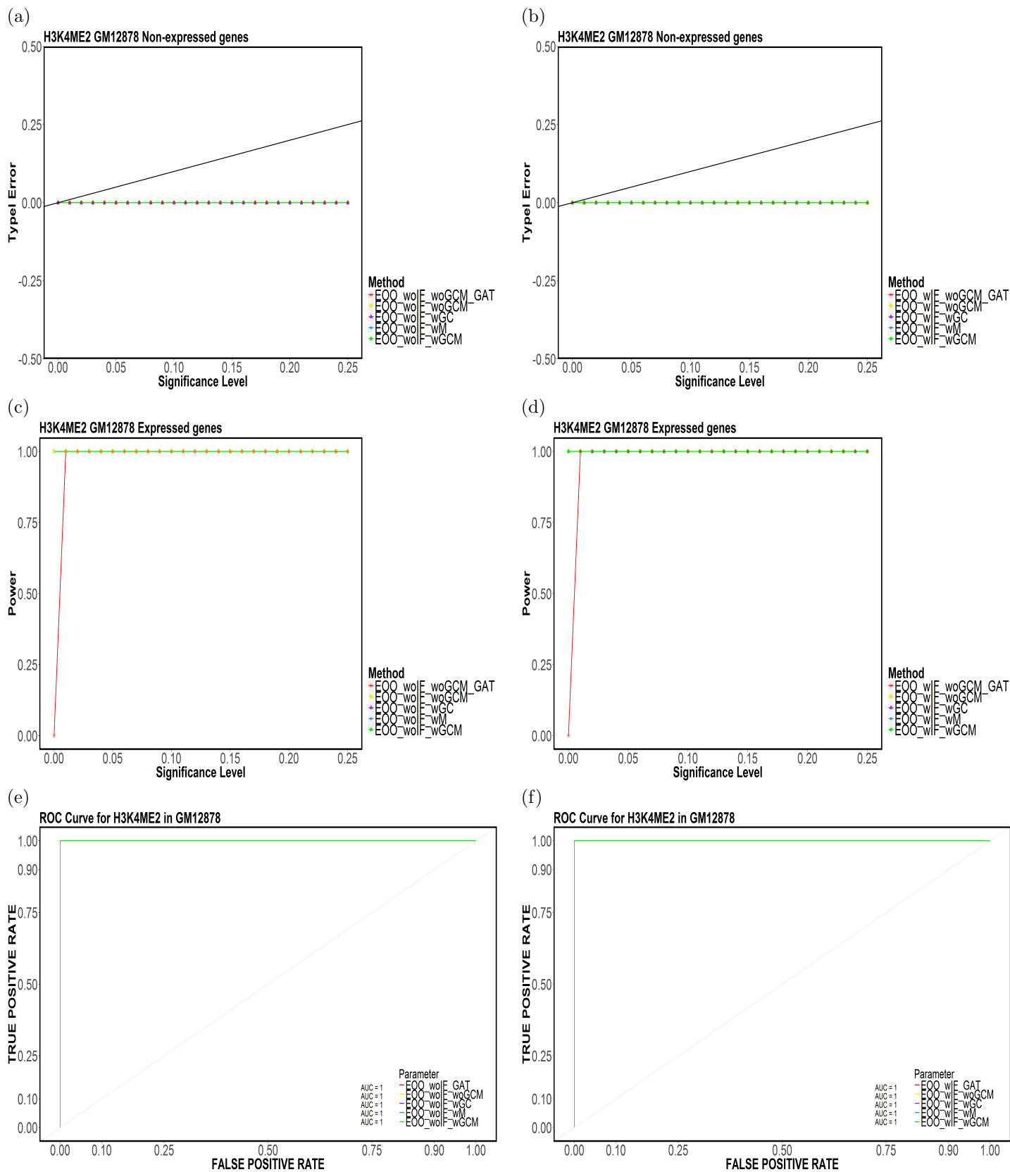
Figure 49: Element-based (a,b) Type-I Error, (c,d) Power and (e,f) ROC Curves for H3K4ME2 in GM12878 for (E00,CompletelyDiscard,Top5).
