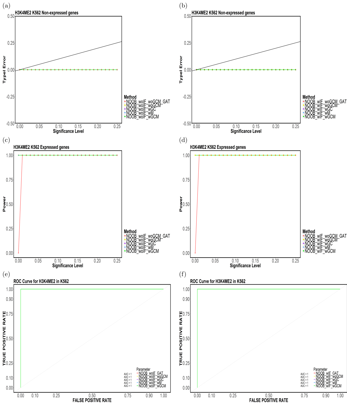
Figure 56: Element-based (a,b) Type-I Error, (c,d) Power and (e,f) ROC Curves for H3K4ME2 in K562 for (NOOB,TakeTheLongest,Top20).
