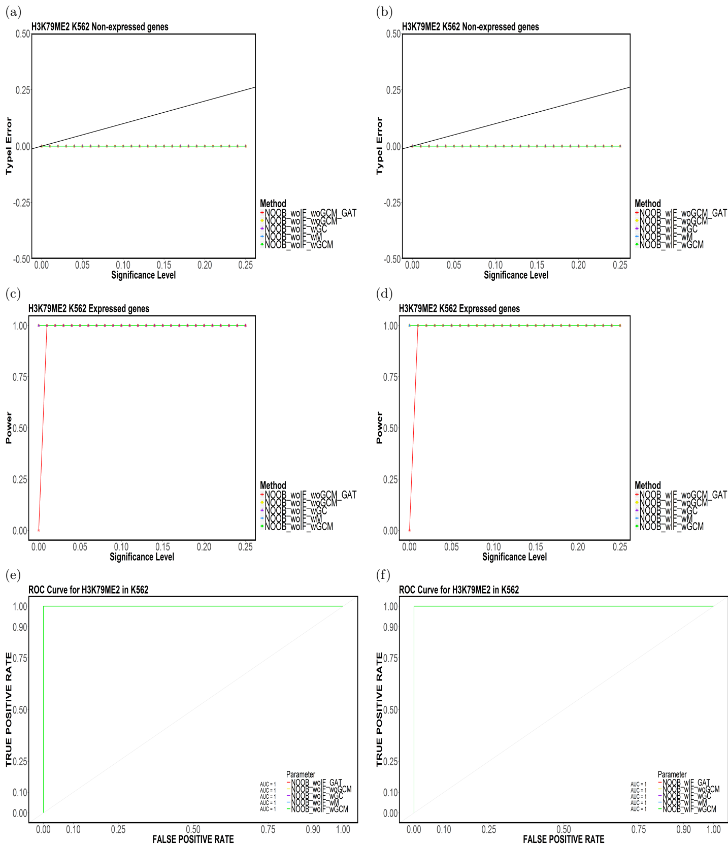
Figure 68: Element-based (a,b) Type-I Error, (c,d) Power and (e,f) ROC Curves for H3K79ME2 in K562 for (NOOB, CompletelyDiscard, Top5).
