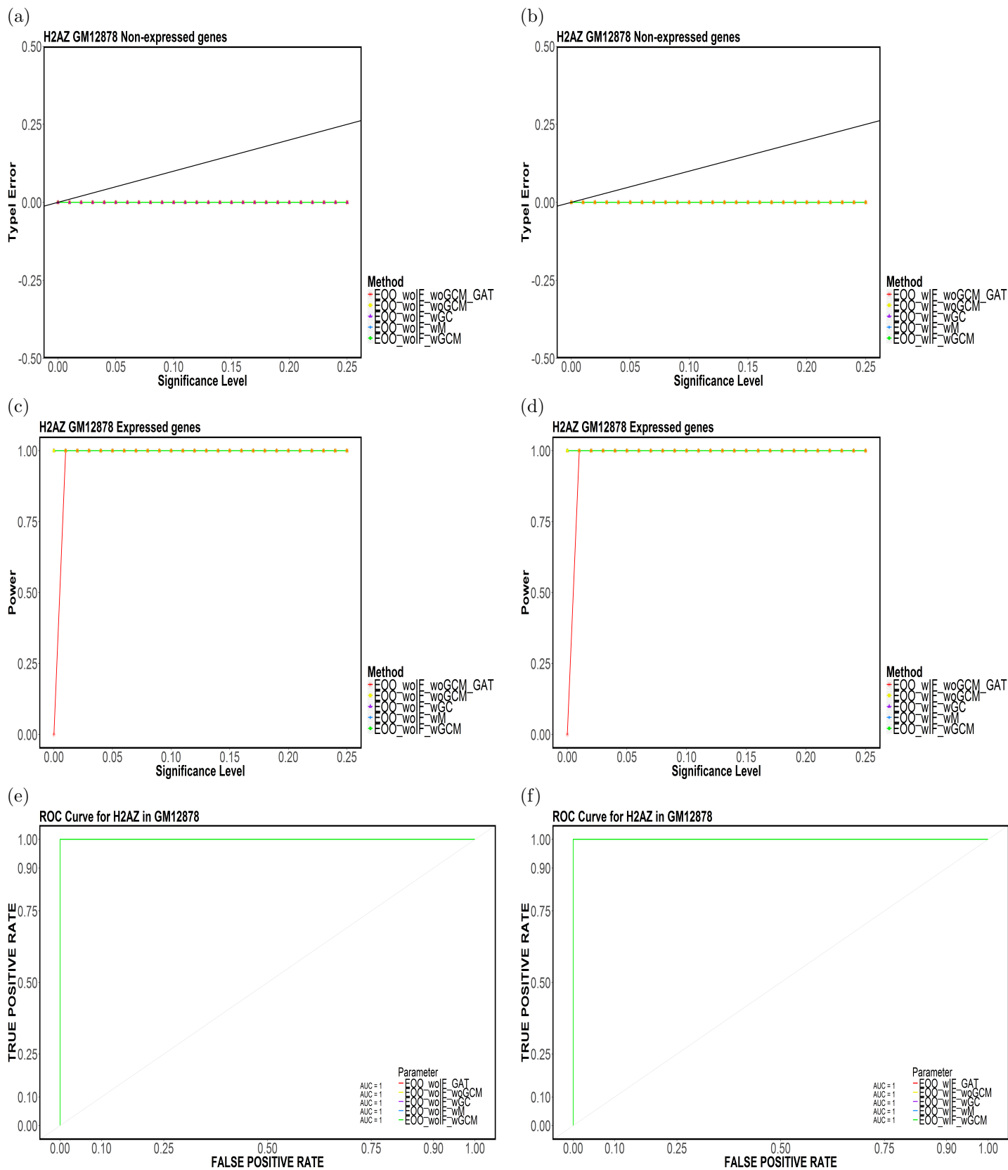
Figure 33: Element-based (a,b) Type-I Error, (c,d) Power and (e,f) ROC Curves for H2AZ in GM12878 for (E00,CompletelyDiscard,Top5).
