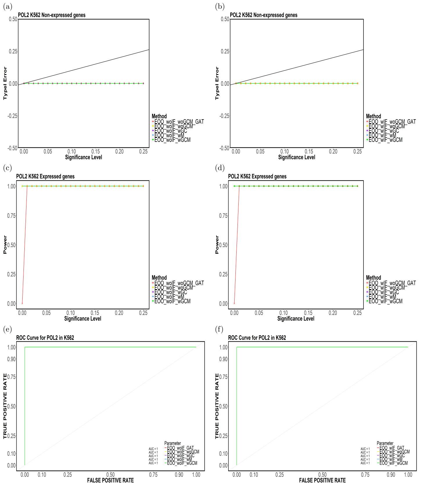
Figure 91: Element-based (a,b) Type-I Error, (c,d) Power and (e,f) ROC Curves for POL2 in K562 for (E00, TakeTheLongest, Top20).
