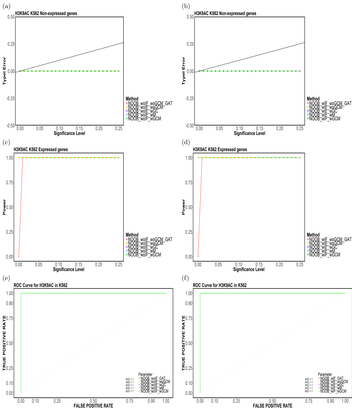
Figure 76: Element-based (a,b) Type-I Error, (c,d) Power and (e,f) ROC Curves for H3K9AC in K562 for (NOOB, CompletelyDiscard, Top5).
