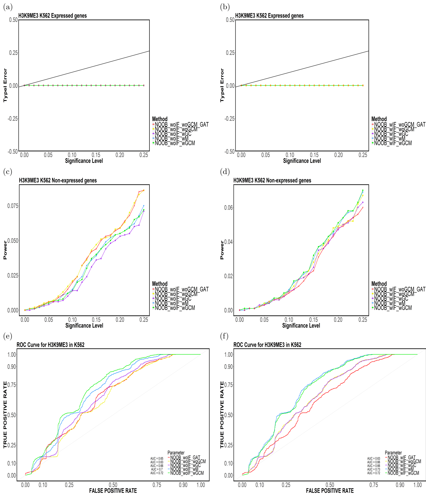
Figure 12: Element-based (a,b) Type-I Error, (c,d) Power and (e,f) ROC Curves for H3K9ME3 in K562 for (NOOB, CompletelyDiscard, Top5).
