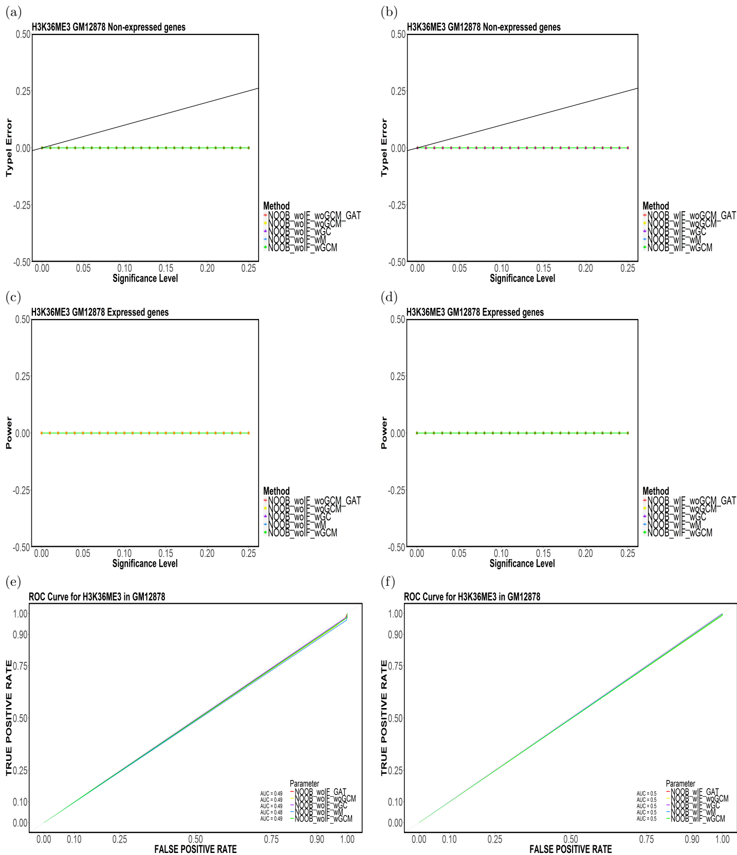
Figure 30: Element-based (a,b) Type-I Error, (c,d) Power and (e,f) ROC Curves for H3K36ME3 in GM12878 for (NOOB,TakeTheLongest,Top20).
