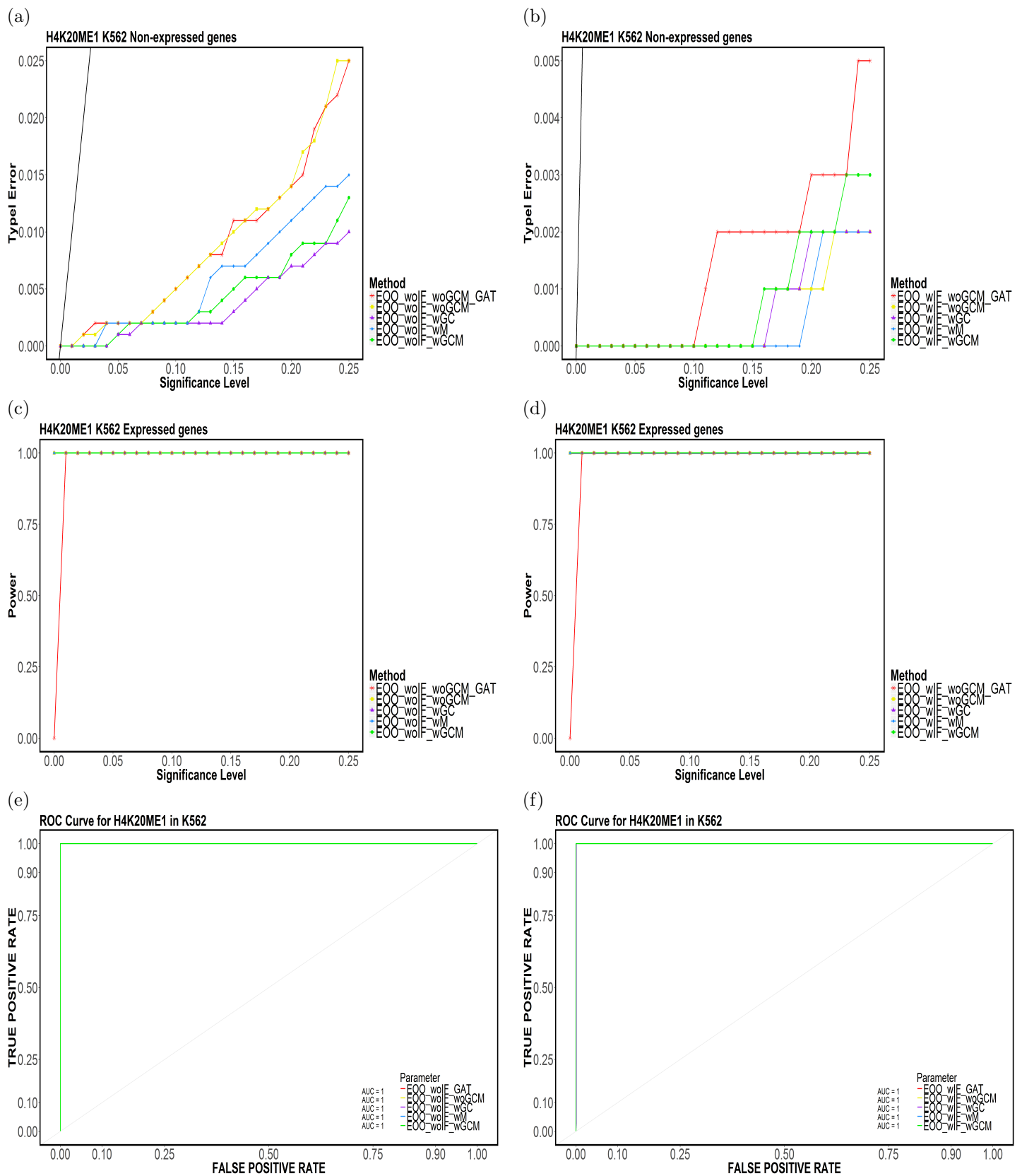
Figure 3: Element-based (a,b) Type-I Error, (c,d) Power and (e,f) ROC Curves for H4K20ME1 in K562 for (E00,CompletelyDiscard,Top5).
