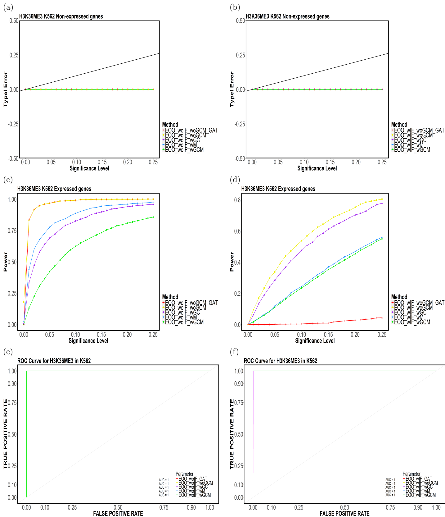
Figure 27: Element-based (a,b) Type-I Error, (c,d) Power and (e,f) ROC Curves for H3K36ME3 in K562 for (E00,CompletelyDiscard,Top5).
