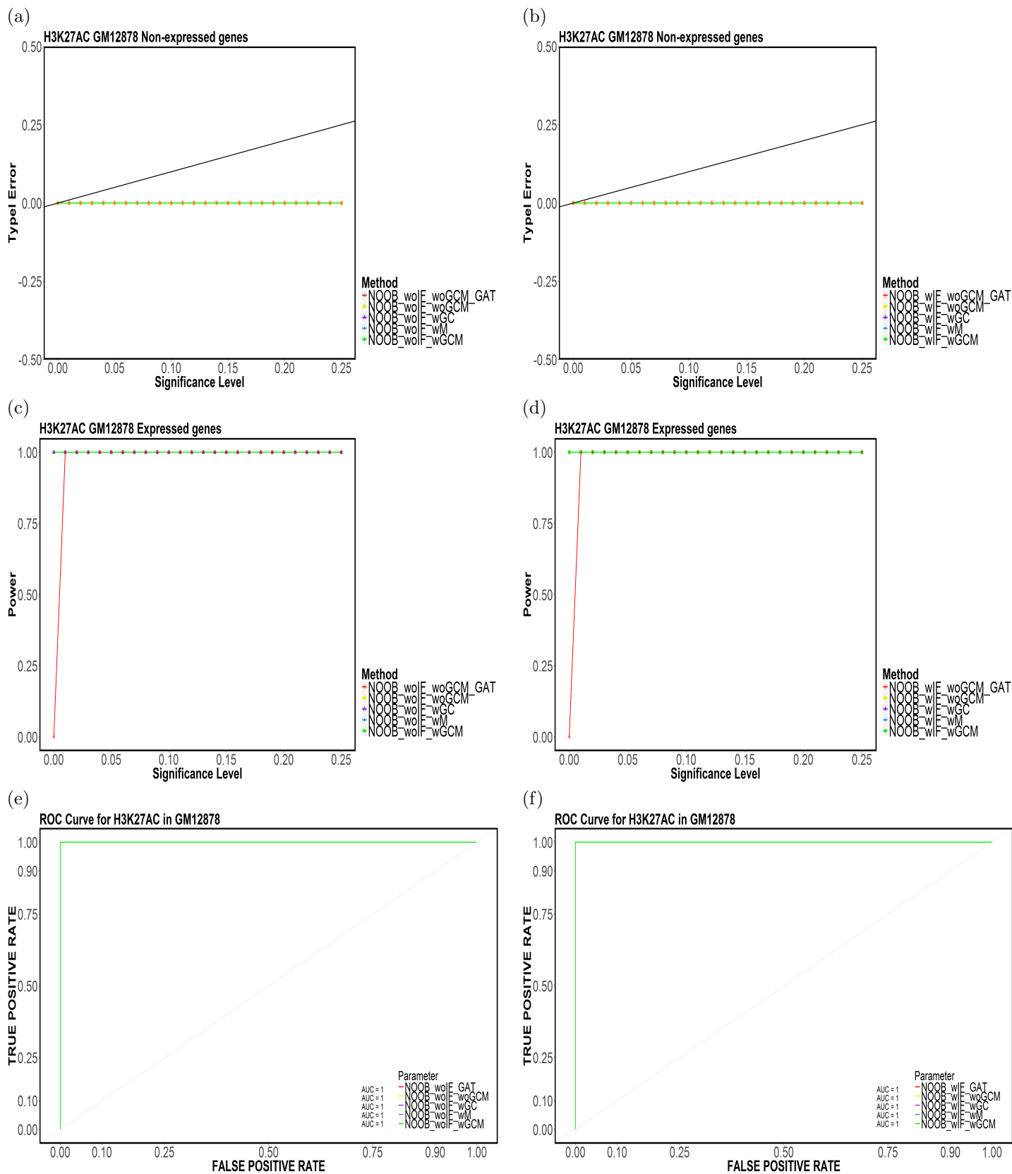
Figure 42: Element-based (a,b) Type-I Error, (c,d) Power and (e,f) ROC Curves for H3K27AC in GM12878 for (NOOB, CompletelyDiscard, Top5).
