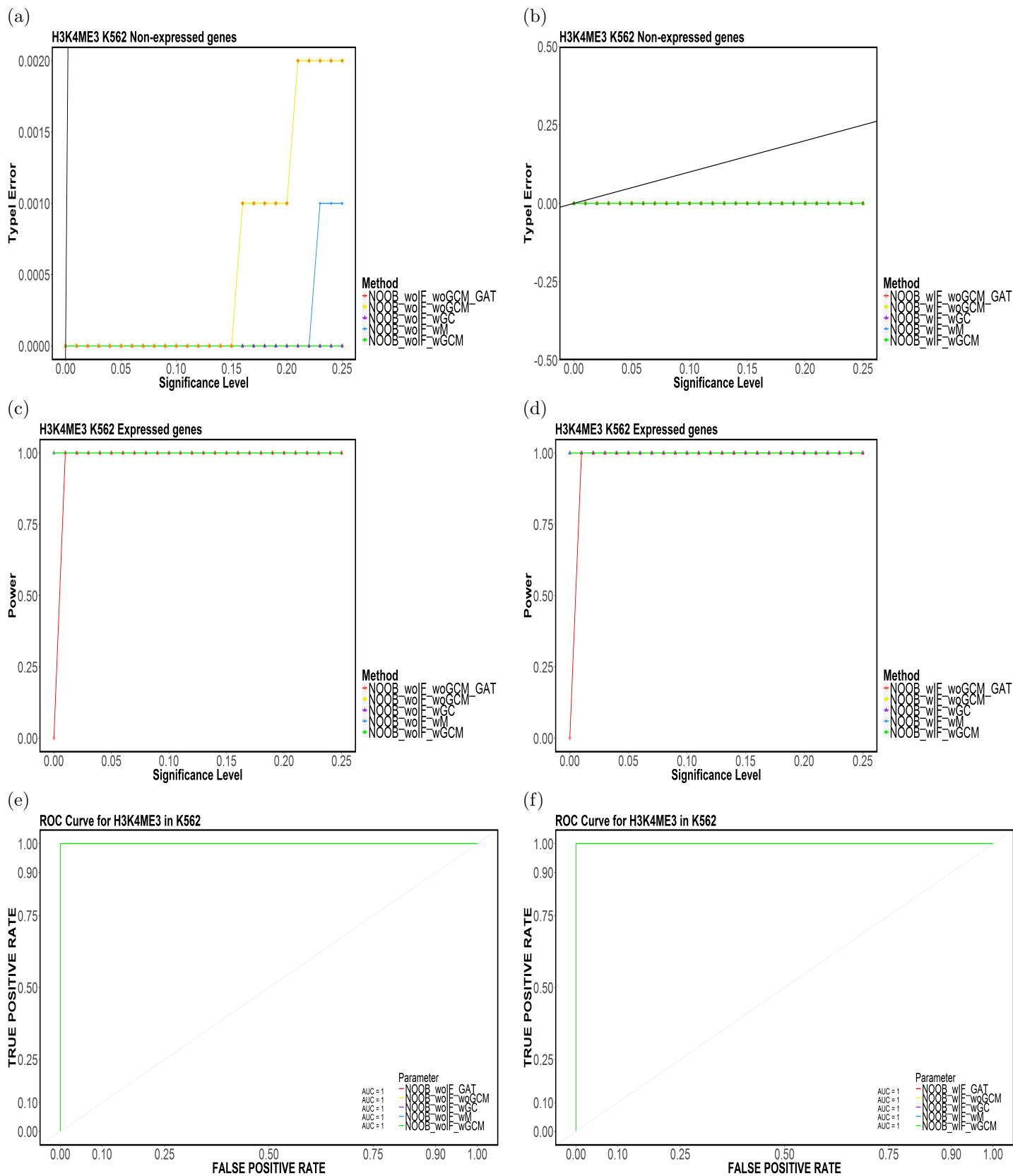
Figure 64: Element-based (a,b) Type-I Error, (c,d) Power and (e,f) ROC Curves for H3K4ME3 in K562 for (NOOB,TakeTheLongest,Top20).
