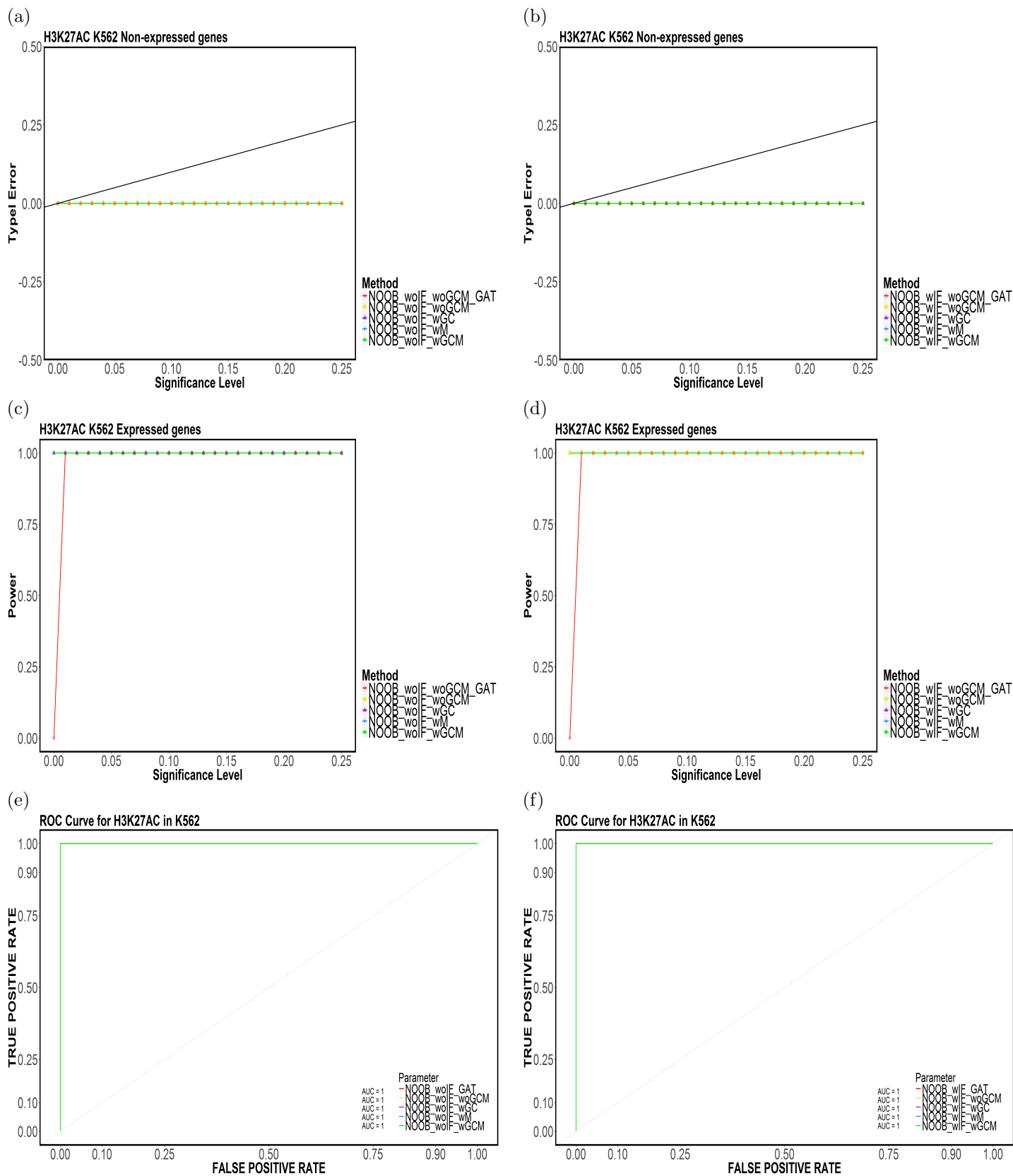
Figure 44: Element-based (a,b) Type-I Error, (c,d) Power and (e,f) ROC Curves for H3K27AC in K562 for (NOOB, CompletelyDiscard, Top5).
