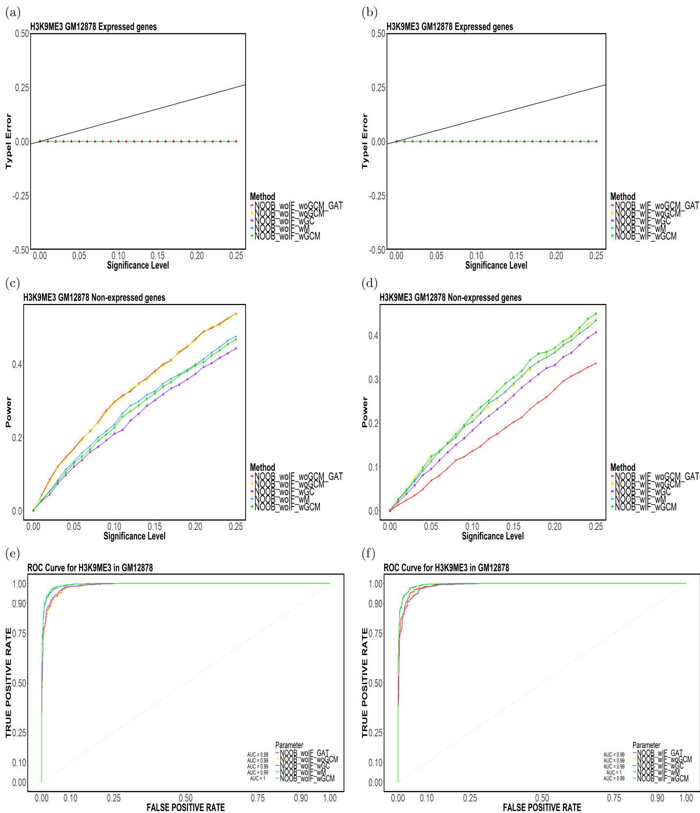
Figure 14: Element-based (a,b) Type-I Error, (c,d) Power and (e,f) ROC Curves for H3K9ME3 in GM12878 for (NOOB,TakeTheLongest,Top20).
