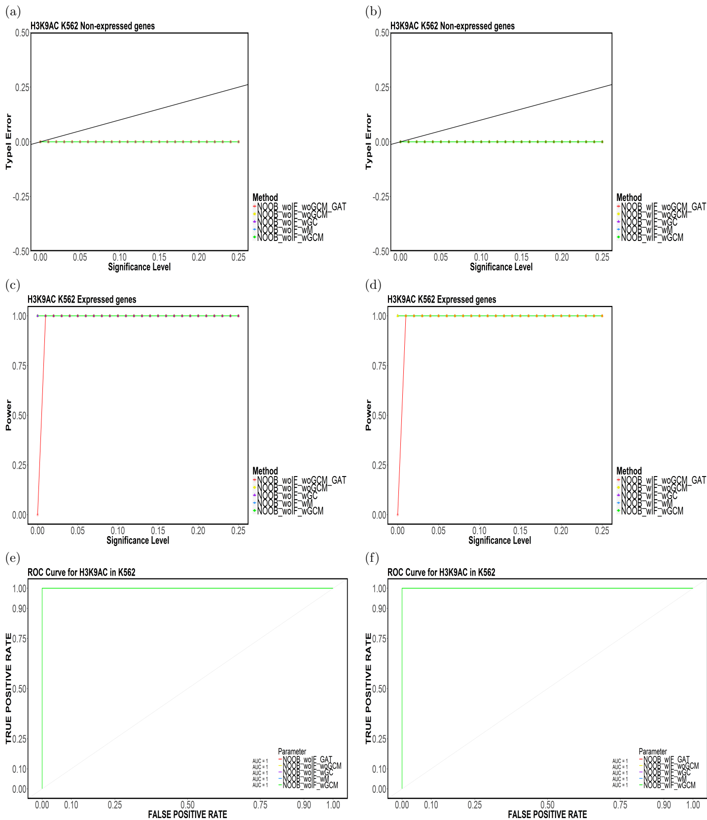
Figure 80: Element-based (a,b) Type-I Error, (c,d) Power and (e,f) ROC Curves for H3K9AC in K562 for (NOOB,TakeTheLongest,Top20).
