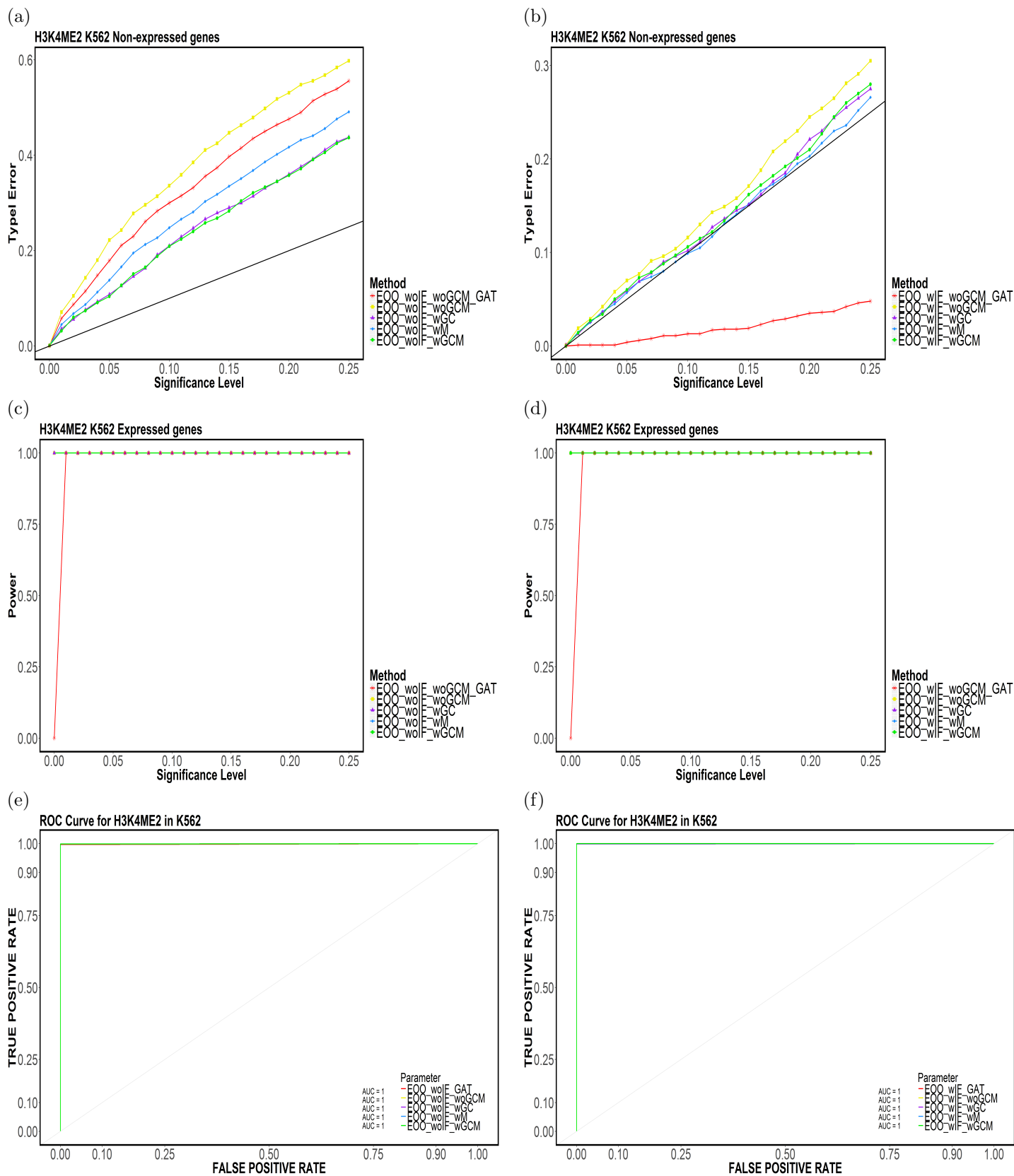
Figure 55: Element-based (a,b) Type-I Error, (c,d) Power and (e,f) ROC Curves for H3K4ME2 in K562 for (E00,TakeTheLongest,Top20).
