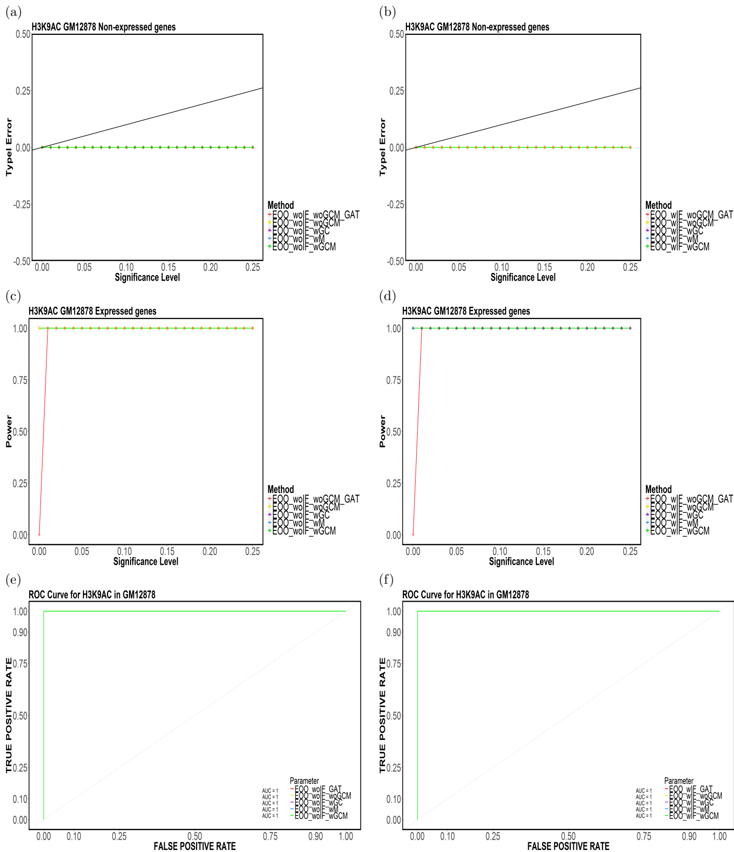
Figure 77: Element-based (a,b) Type-I Error, (c,d) Power and (e,f) ROC Curves for H3K9AC in GM12878 for (E00,TakeTheLongest,Top20).
