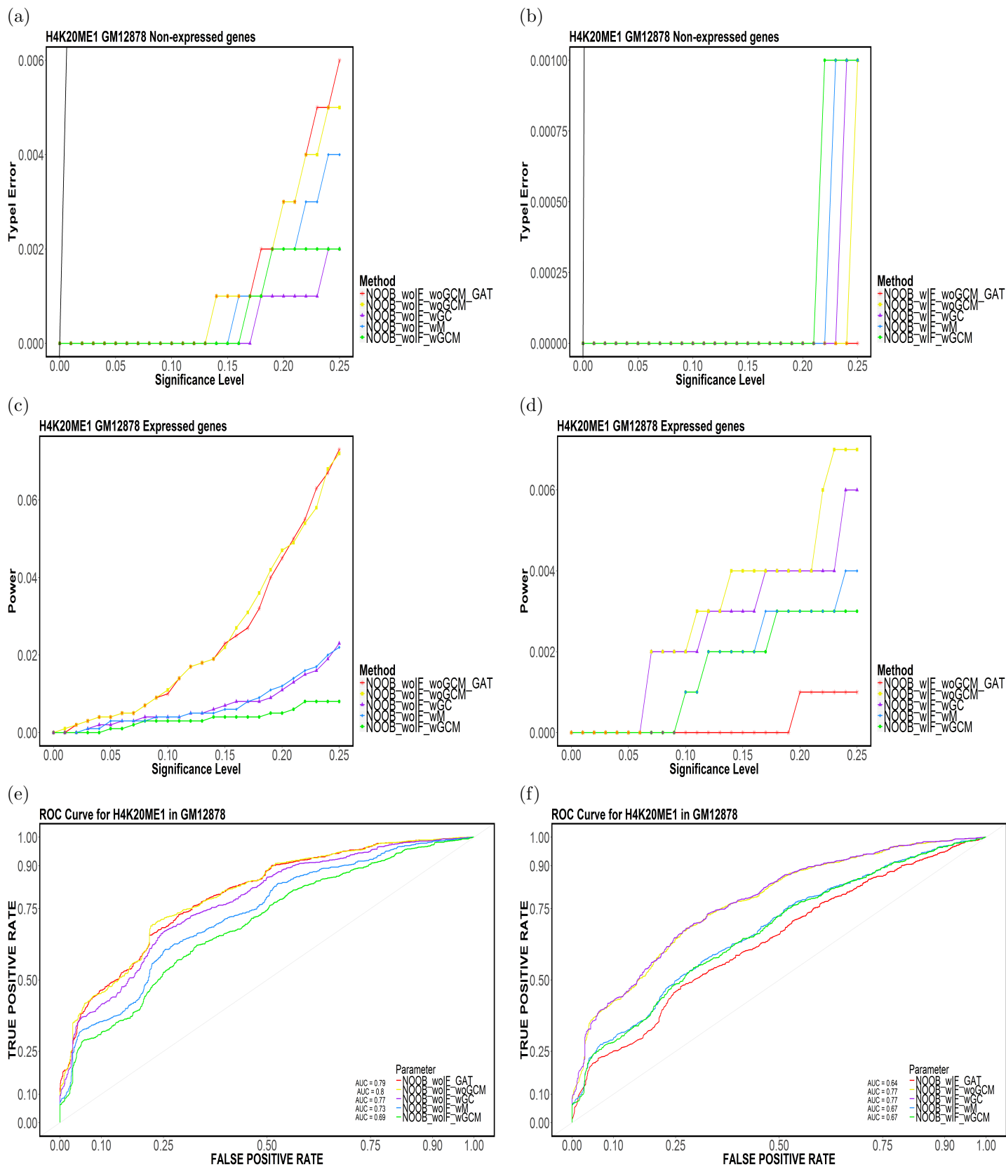
Figure 6: Element-based (a,b) Type-I Error, (c,d) Power and (e,f) ROC Curves for H4K20ME1 in GM12878 for (NOOB,TakeTheLongest,Top20).
