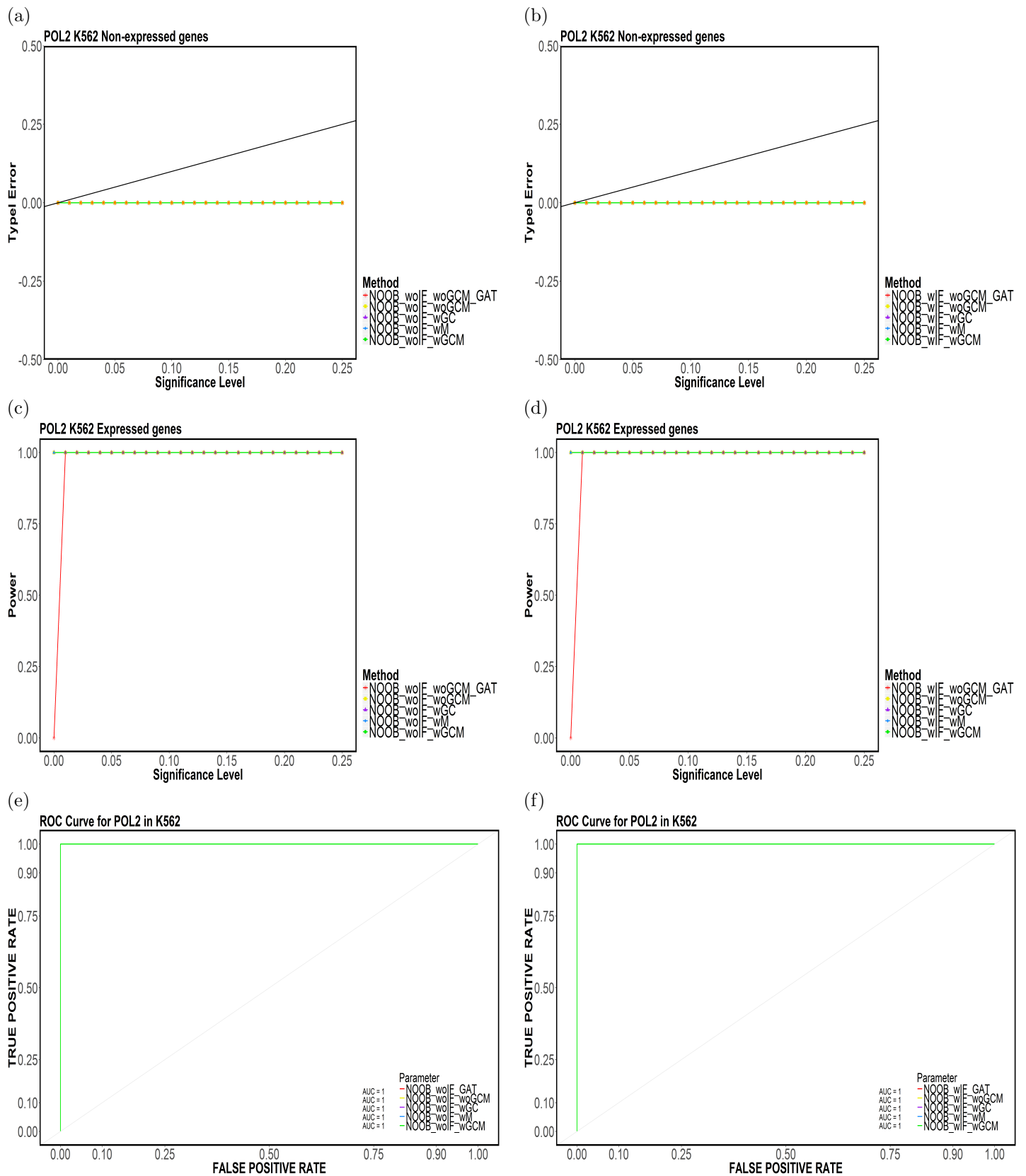
Figure 88: Element-based (a,b) Type-I Error, (c,d) Power and (e,f) ROC Curves for POL2 in K562 for (NOOB,CompletelyDiscard,Top5).
