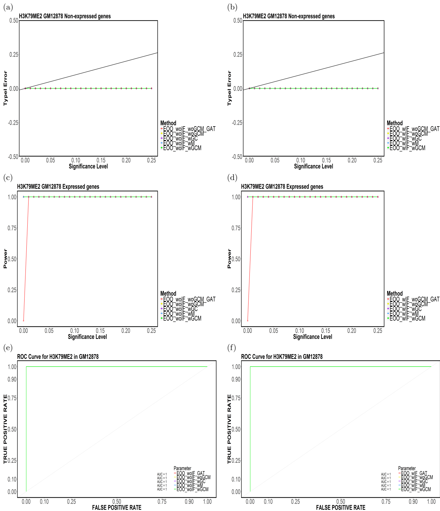
Figure 65: Element-based (a,b) Type-I Error, (c,d) Power and (e,f) ROC Curves for H3K79ME2 in GM12878 for (E00,CompletelyDiscard,Top5).
