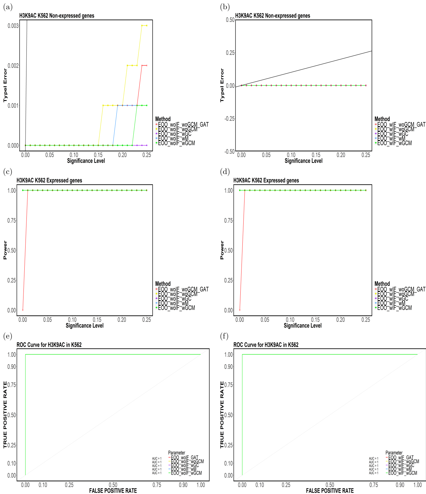
Figure 79: Element-based (a,b) Type-I Error, (c,d) Power and (e,f) ROC Curves for H3K9AC in K562 for (E00,TakeTheLongest,Top20).
