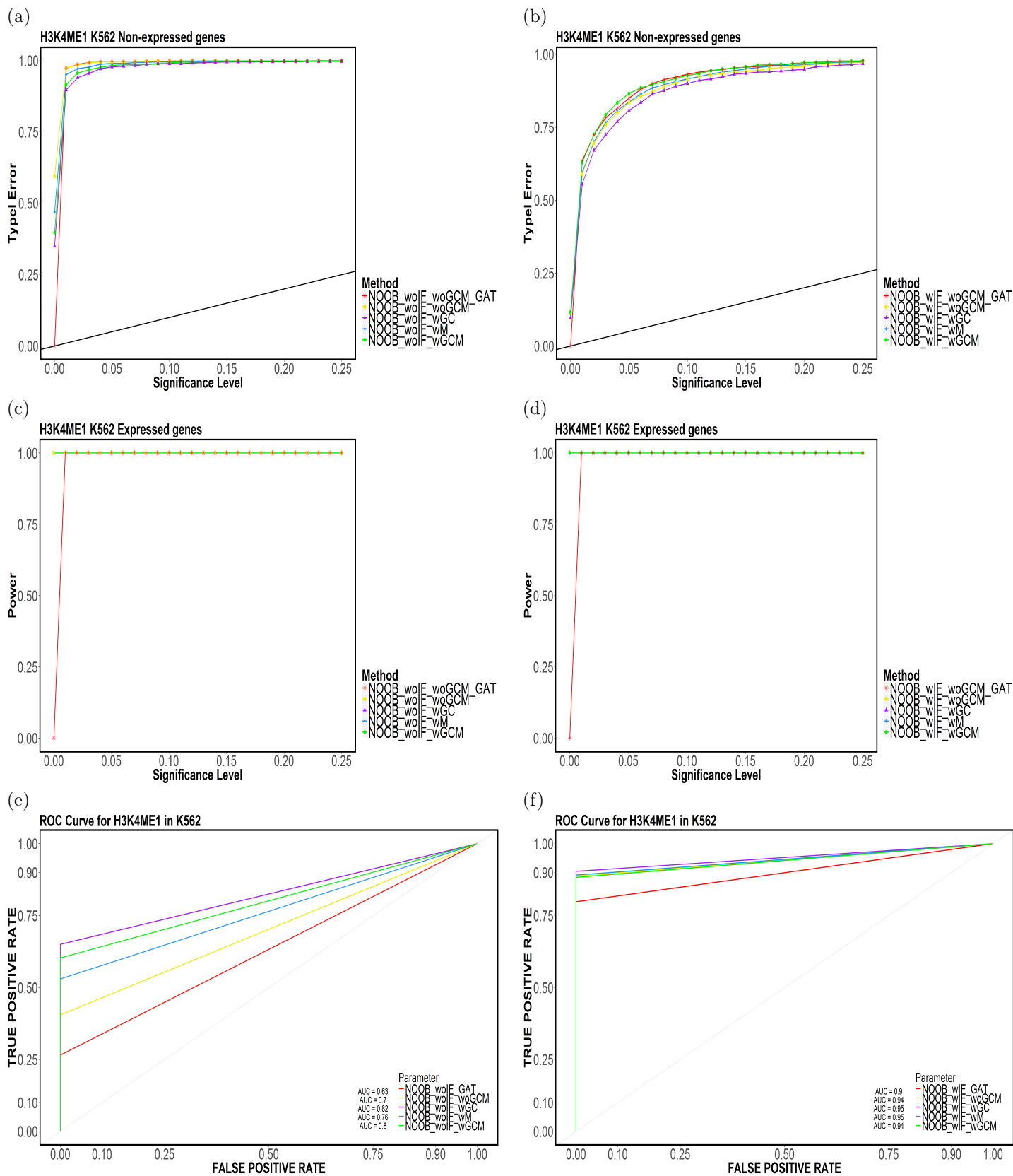
Figure 24: Element-based (a,b) Type-I Error, (c,d) Power and (e,f) ROC Curves for H3K4ME1 in K562 for (NOOB,TakeTheLongest,Top20).
