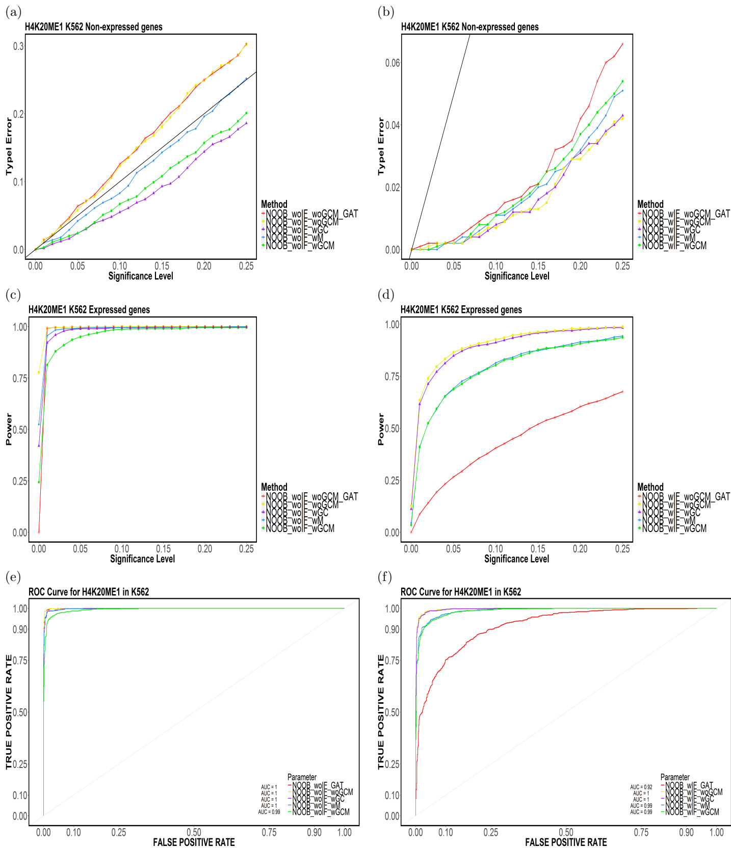
Figure 8: Element-based (a,b) Type-I Error, (c,d) Power and (e,f) ROC Curves for H4K20ME1 in K562 for (NOOB,TakeTheLongest,Top20).
