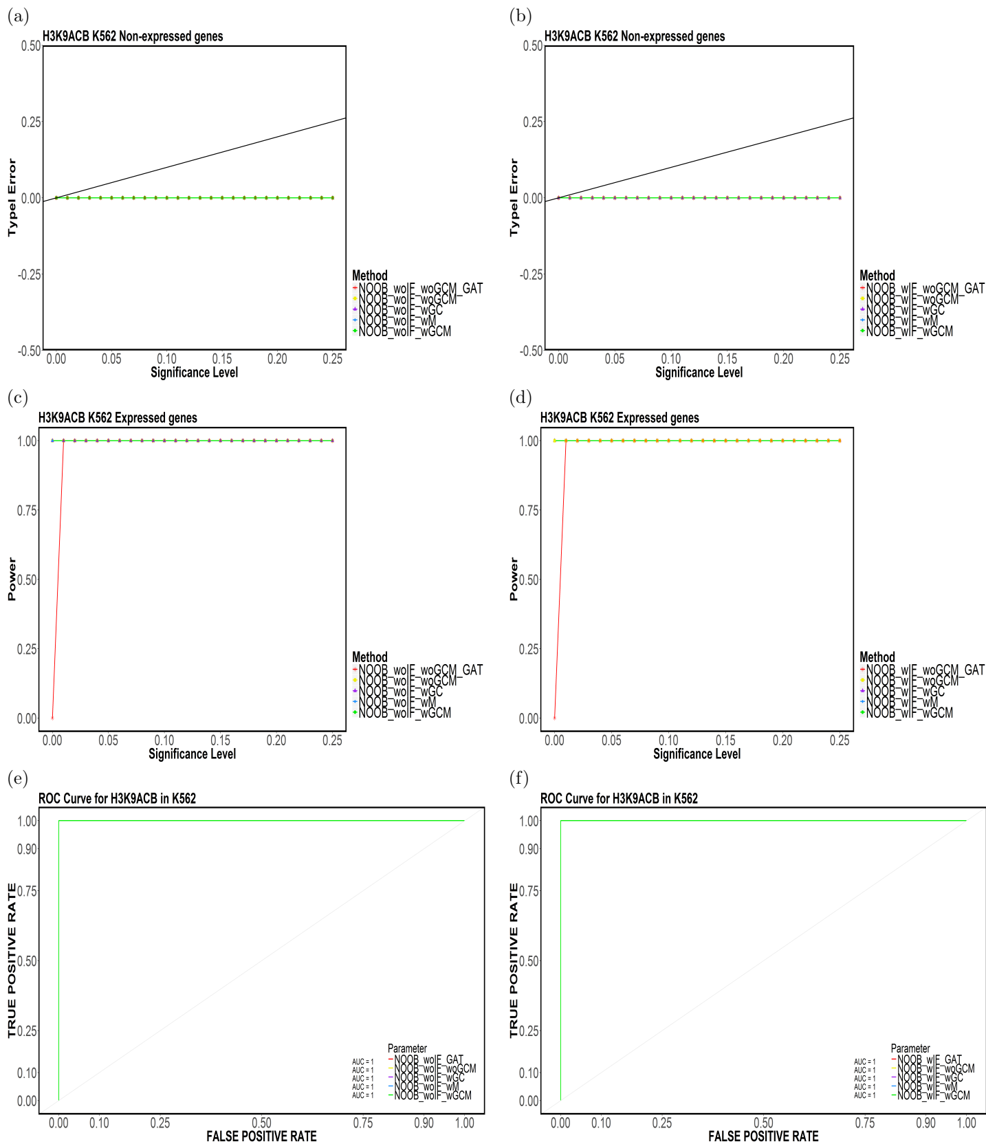
Figure 82: Element-based (a,b) Type-I Error, (c,d) Power and (e,f) ROC Curves for H3K9ACB in K562 for (NOOB, CompletelyDiscard, Top5).
