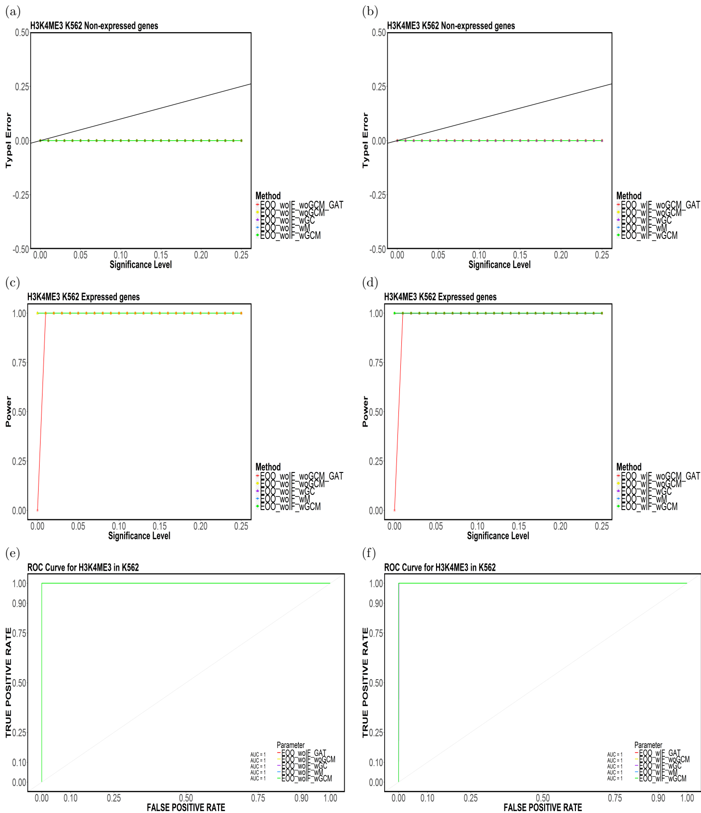
Figure 59: Element-based (a,b) Type-I Error, (c,d) Power and (e,f) ROC Curves for H3K4ME3 in K562 for (E00,CompletelyDiscard,Top5).
