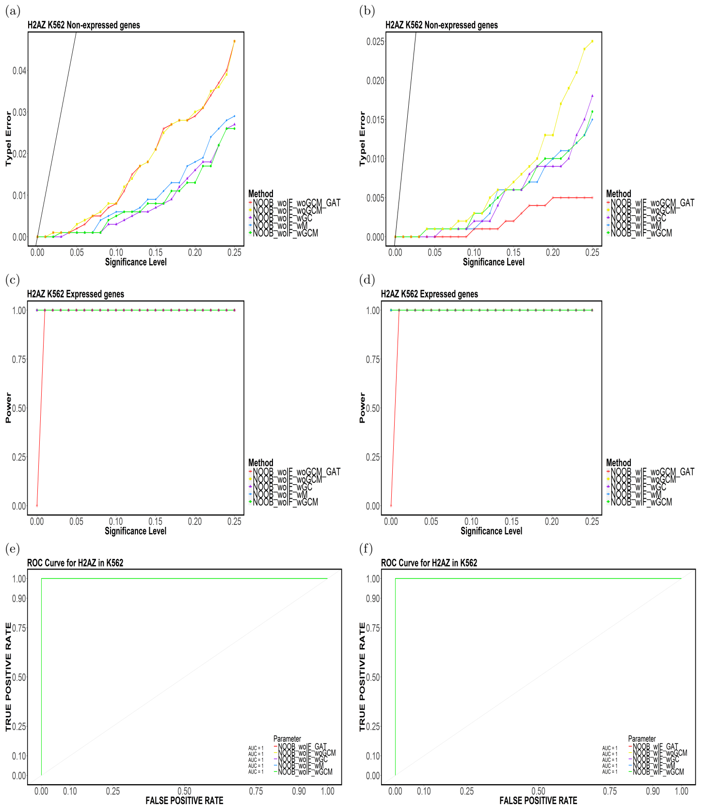
Figure 40: Element-based (a,b) Type-I Error, (c,d) Power and (e,f) ROC Curves for H2AZ in K562 for (NOOB,TakeTheLongest,Top20).
